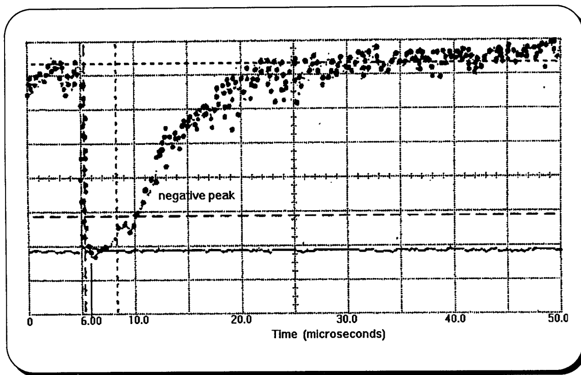
Figure 3.2. Typical Clear Air Back-scatter Signal Displayed on HP 5411D Oscilloscope
