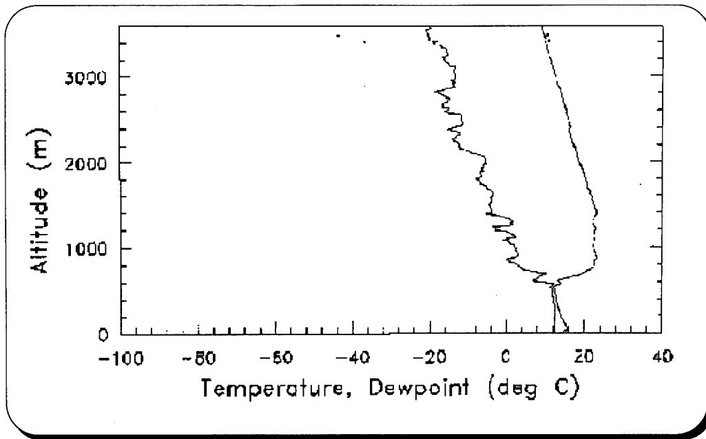
Figure 5.7. Radiosonde Profiles of Temperature and Dewpoint
