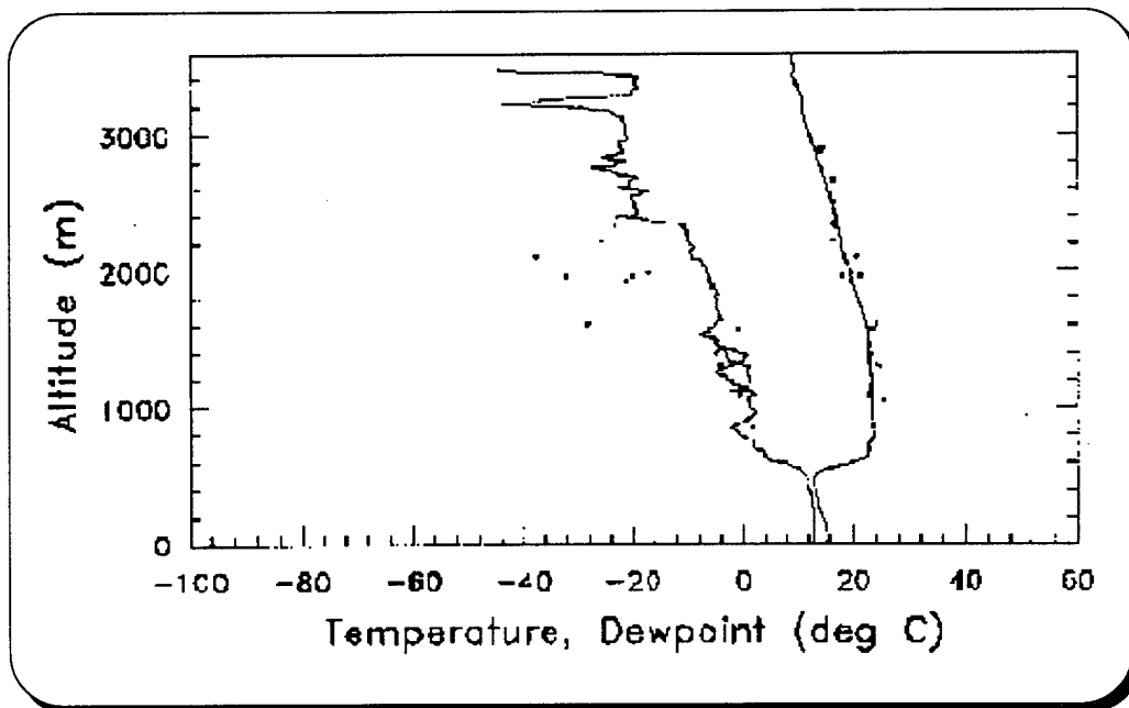
Figure 5.6. Radiosonde Profiles of Temperature and Dewpoint
