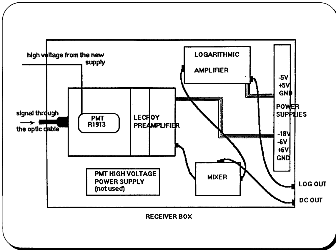
Figure 4.4. Block Diagram of the Receiver Box
