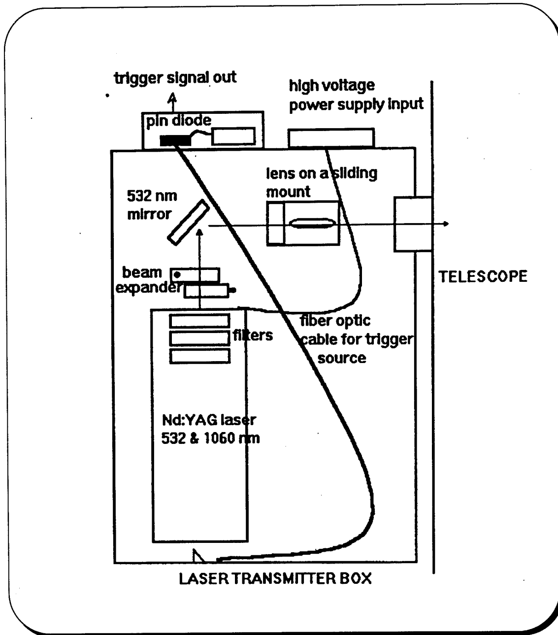
Figure 4.2. Block Diagram of the Laser Transmitter Box
