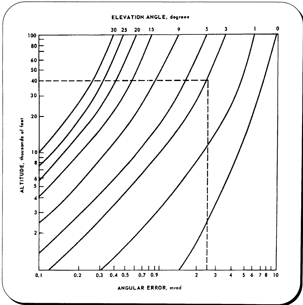
Figure 2.2. Target Angular Error vs. Target Altitude [Ref.5]
