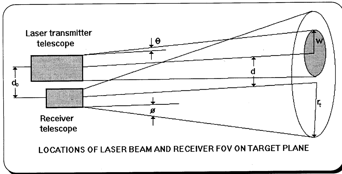
Figure 3.1. Field-of-View Configuration [Ref.8]
