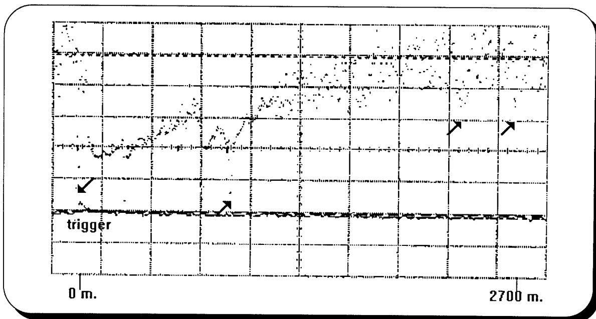
Figure 5.3. Lidar Returns Showing Hard Targets at 900m, 2400m and 2700m
