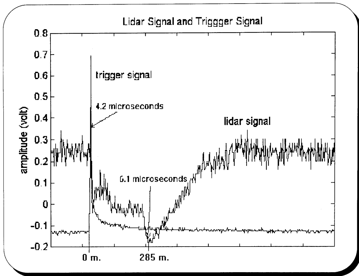
Figure 5.12. Night Time Lidar Return Signal from Clouds
