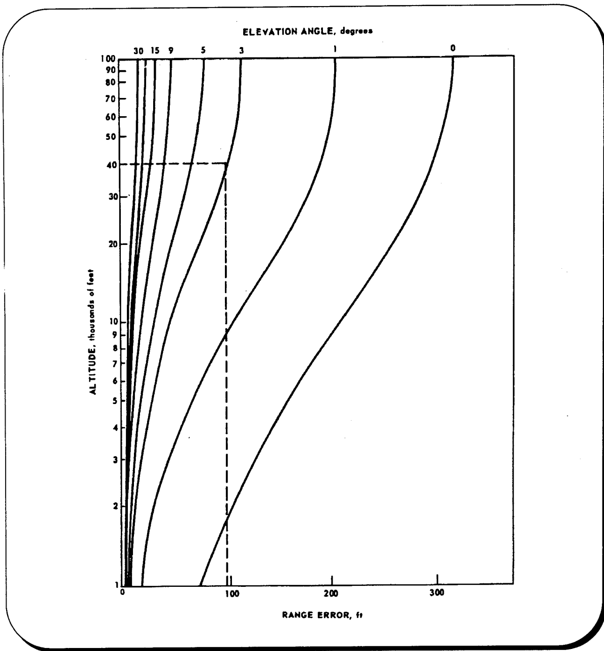
Figure 2.3. Target Range Error vs. Target Altitude [Ref.5]
