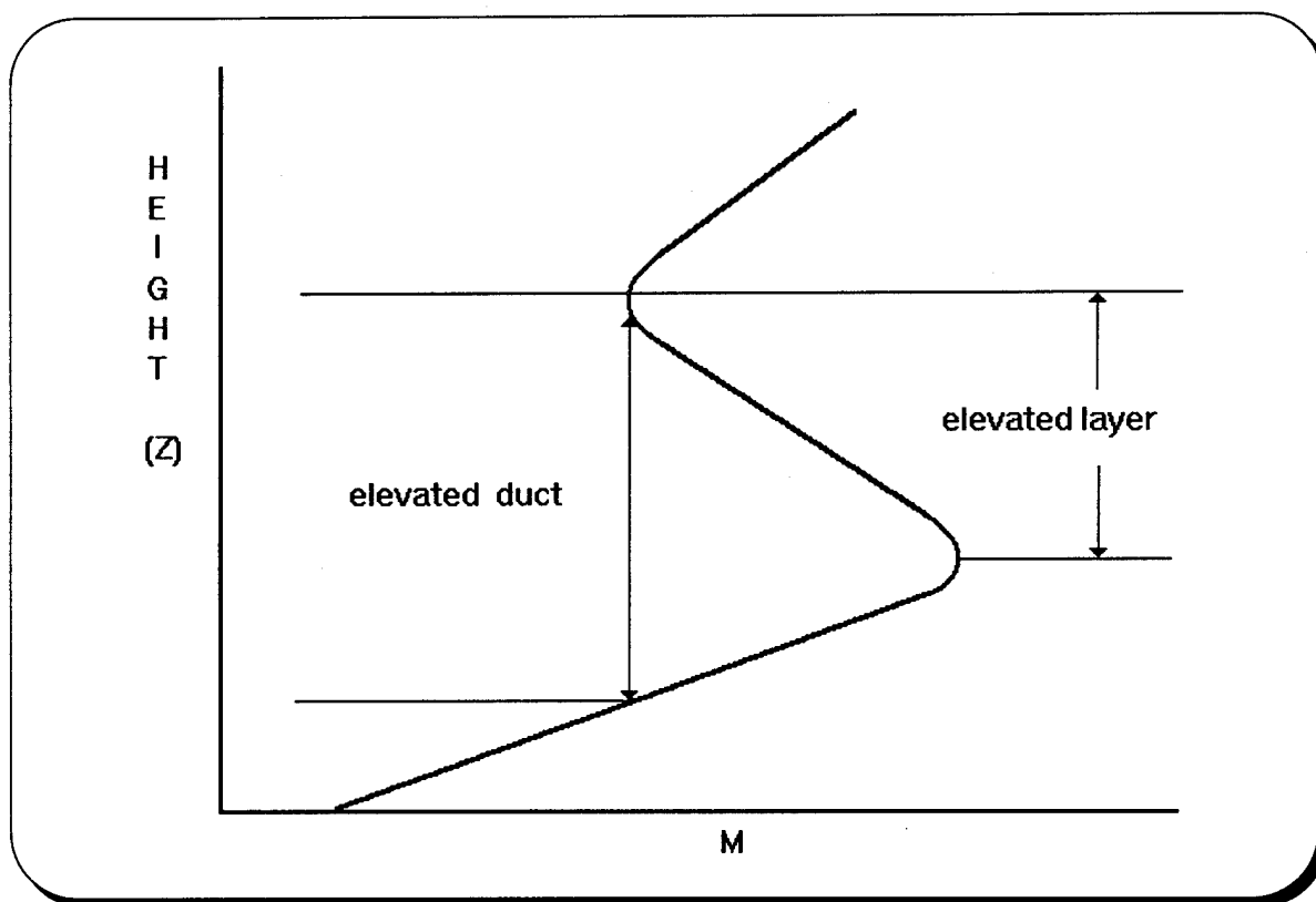
Figure 2.4. Trapping Layer and Duct Occurrence [Ref.6]
