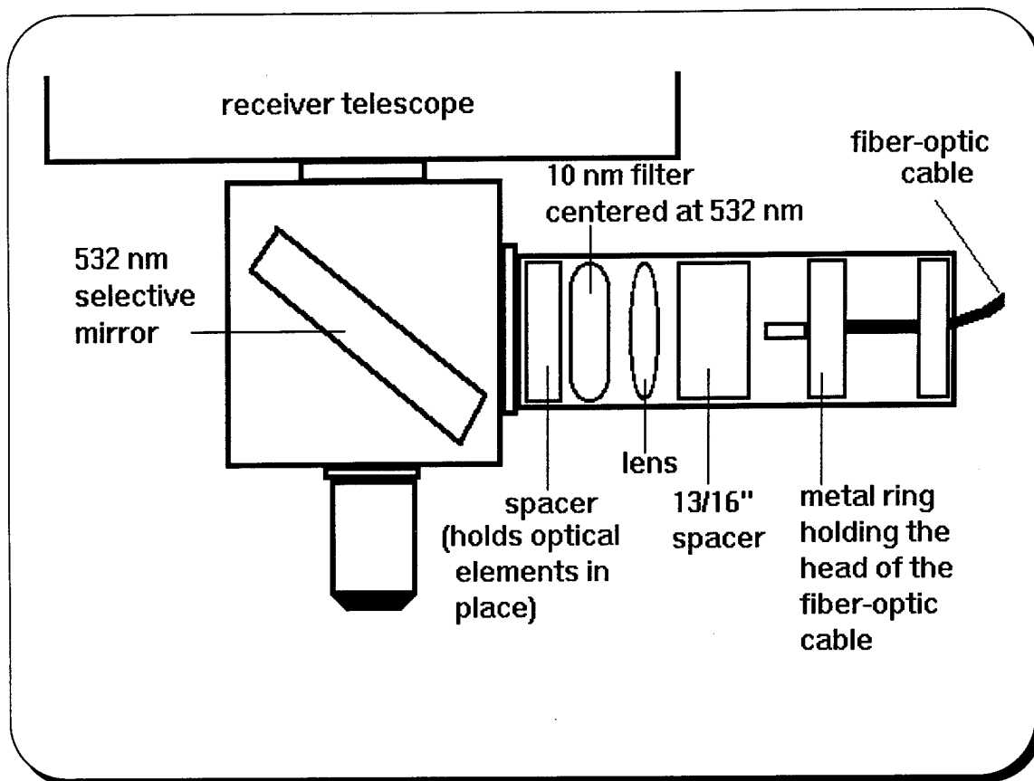
Figure 4.3. Receiver Telescope to PMT Connection
