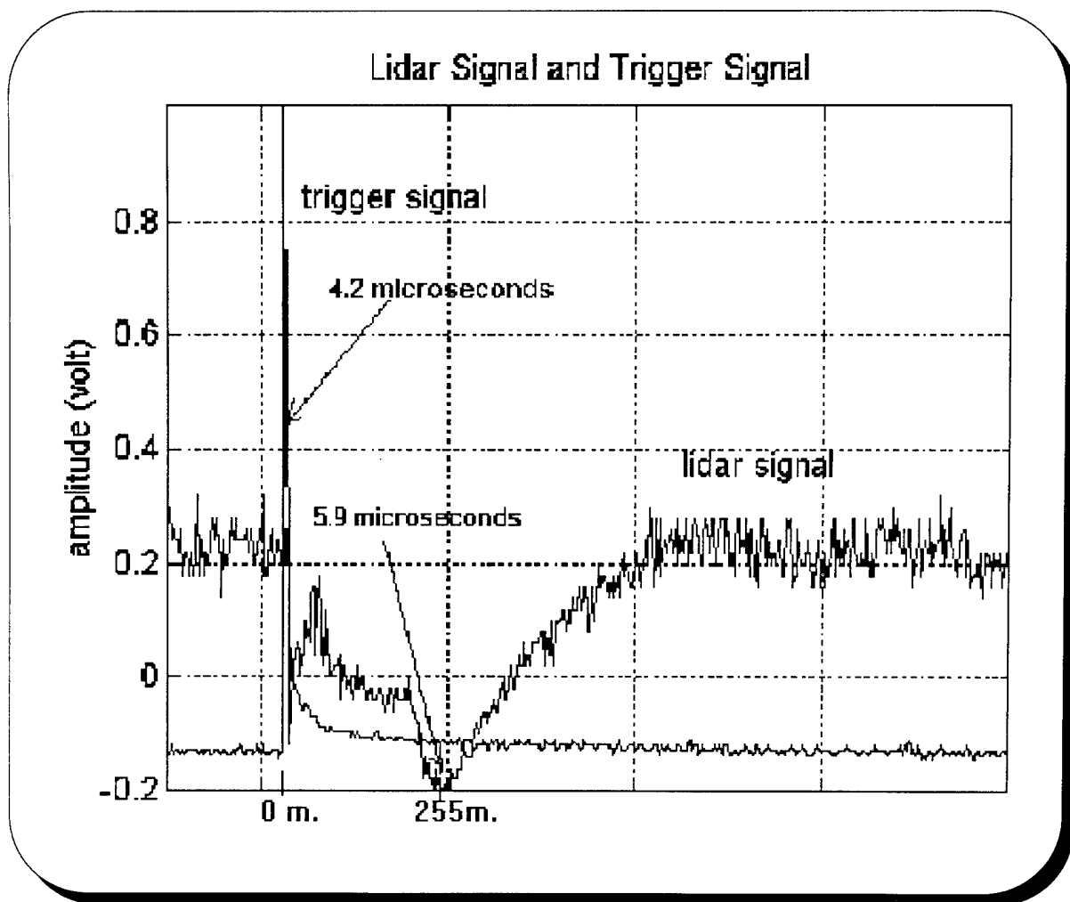
Figure 5.10. Night Time Lidar Return Signal from Haze Layer (Platform elevation is 30 m)
