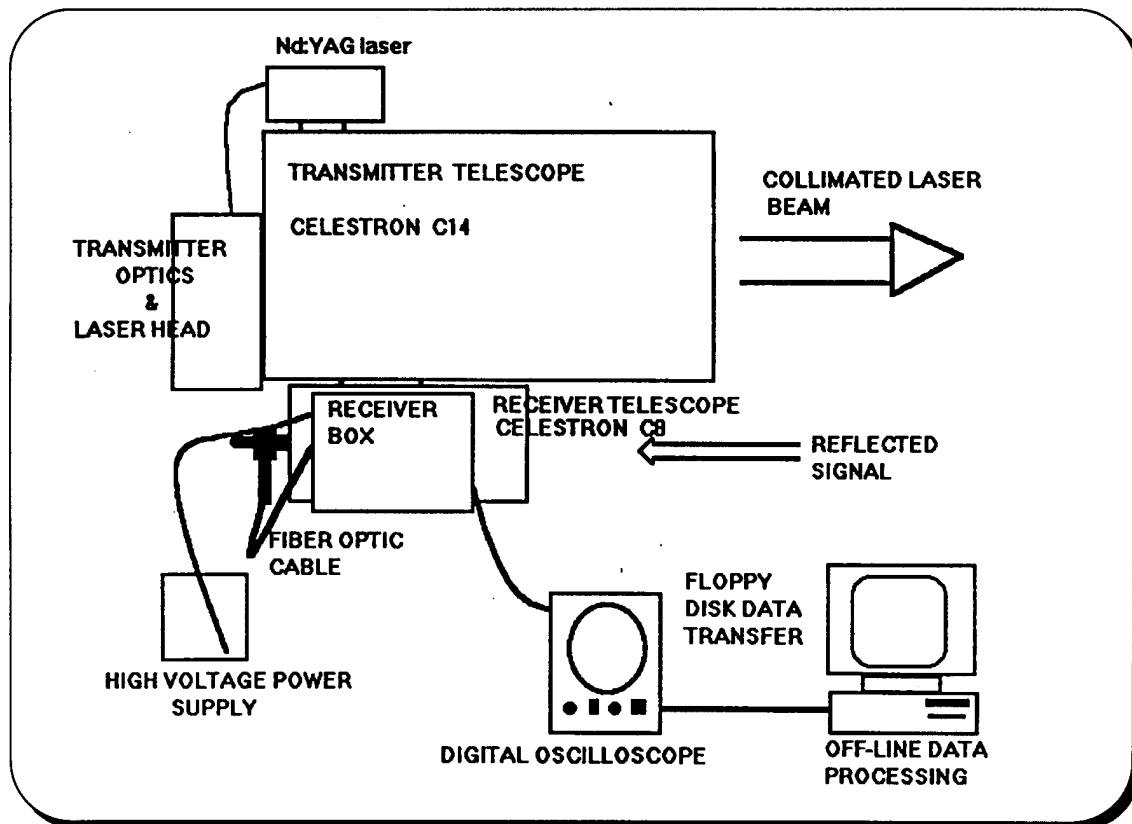
Figure 4.1. Block Diagram of the Lidar System
