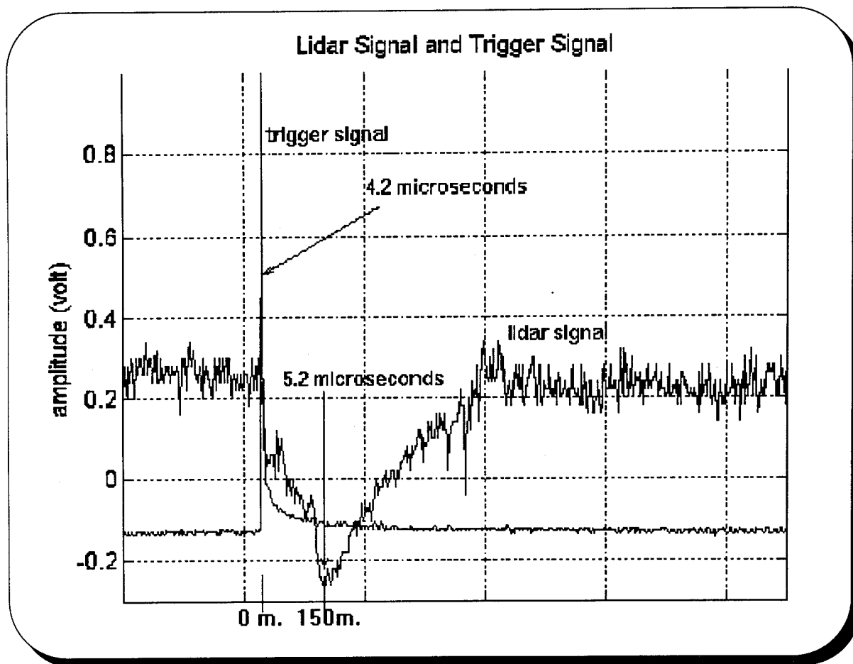
Figure 5.9. Night Time Lidar Return Signal from Haze Layer (Platform elevation is 30 m)
