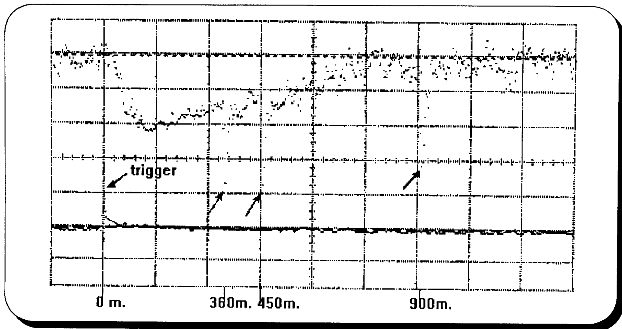
Figure 5.2. Lidar Returns Showing Hard (Tree) Targets at 340m, 450m and 900m.
