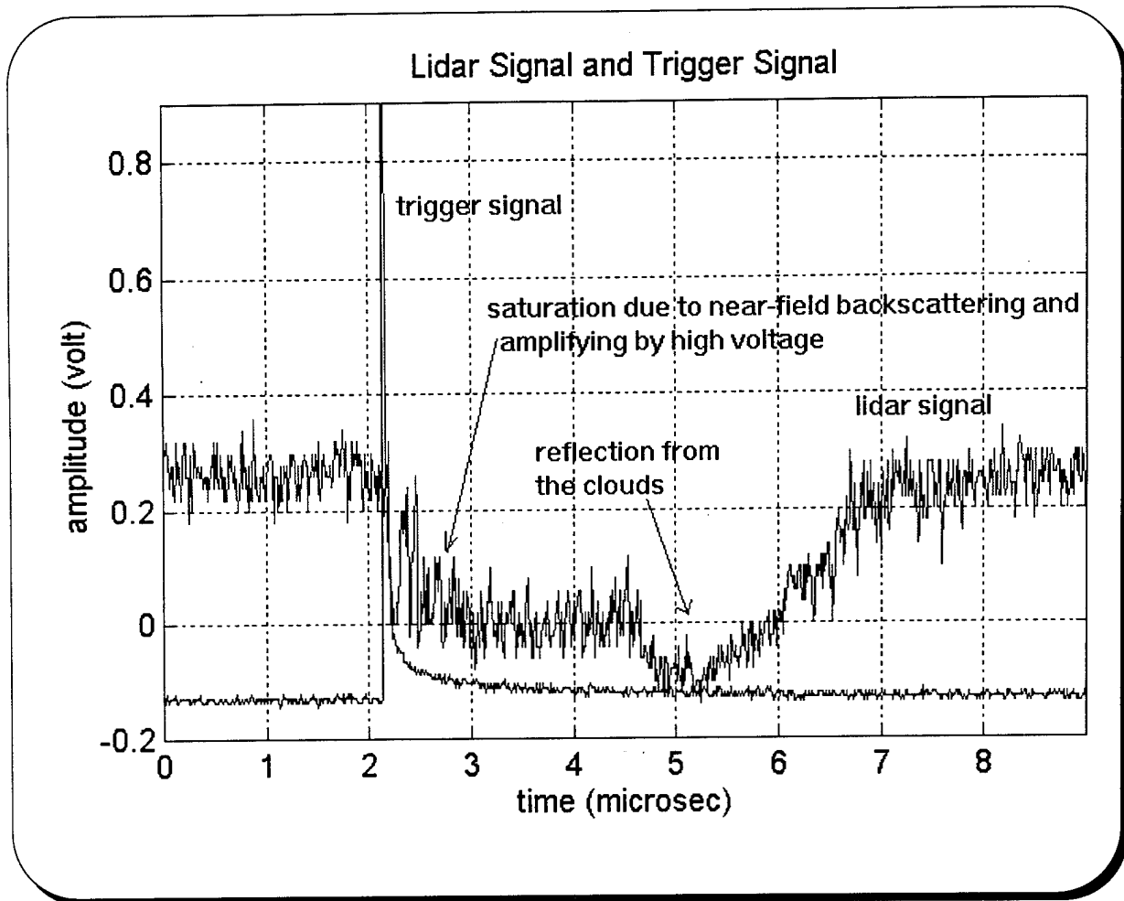
Figure 5.13. Night Time Lidar Return with Cloud. PMT Showing Deterioration.
