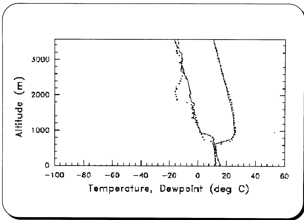
Figure 5.4. Radiosonde Profiles of Temperature and Dewpoint
