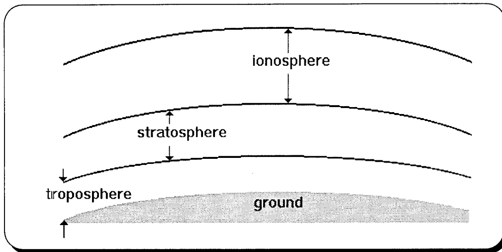
Figure 2.1. Atmospheric Layers
