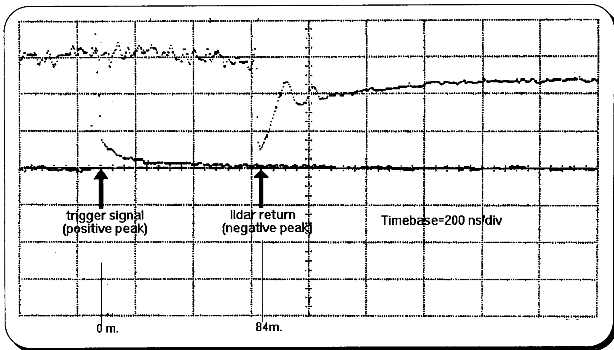
Figure 5.1. Lidar Signal in Close Range Test
