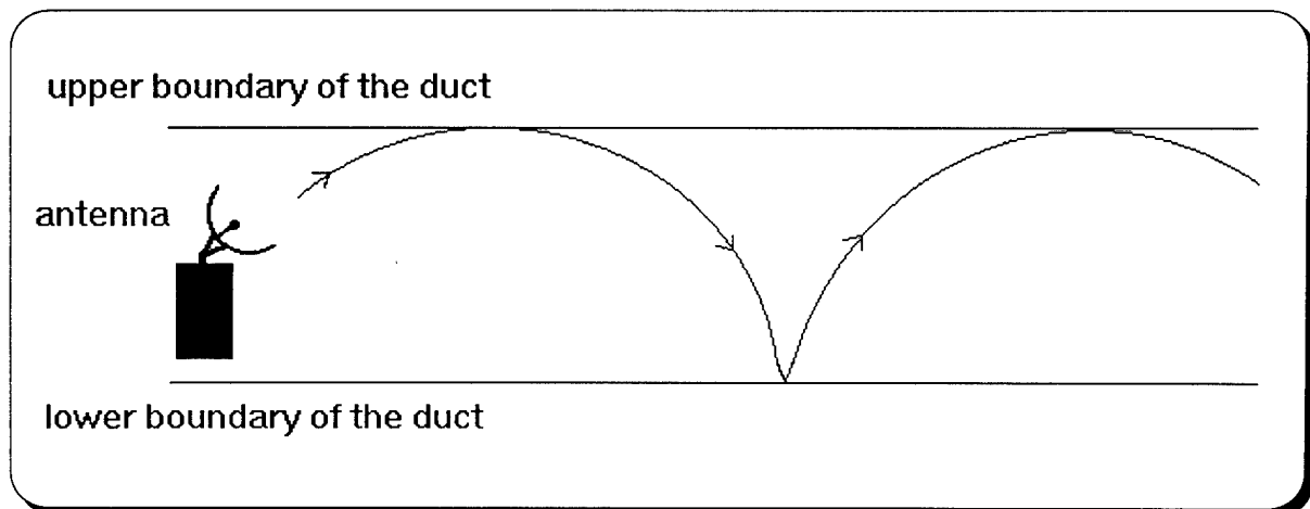
Figure 2.5. Ducting Effects in Propagation Patterns [Ref.4]
