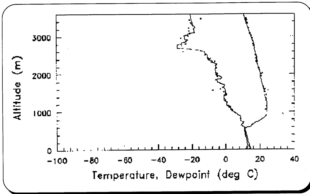
Figure 5.5. Radiosonde Profiles of Temperature and Dewpoint
