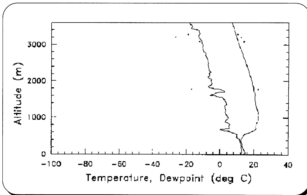
Figure 5.8. Radiosonde Profiles of Temperature and Dewpoint
