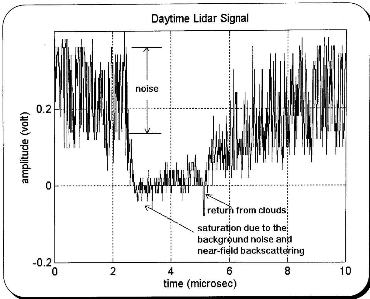
Figure 5.11. Daytime Lidar Return
