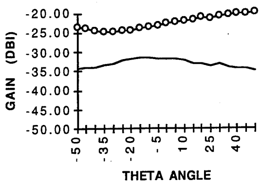
.90 GHZ (HTS1)
