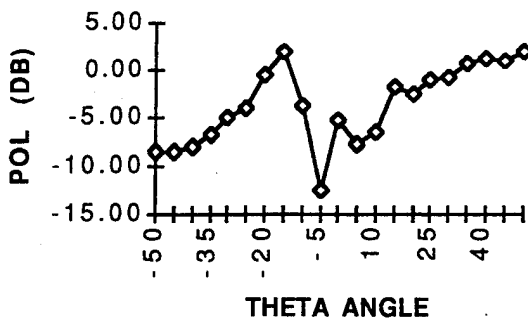
RIGHT TO LEFT CIRCULAR POLARIZATION-0.4 GHZ
