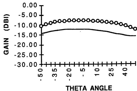
1.0 GHZ (HTS1)
