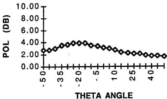
RIGHT TO LEFT CIRCULAR POLARIZATION-0.9 GHZ
