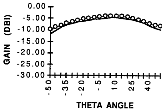
1.8 GHZ (HTS1)
