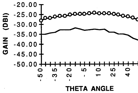
.60 GHZ (HTS1)
