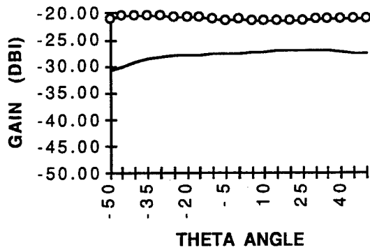
.70 GHZ (HTS1)
