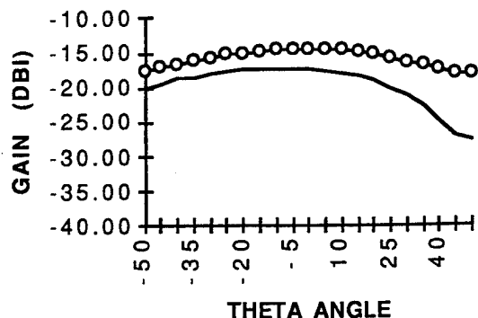
.90 GHZ (HTS1)
