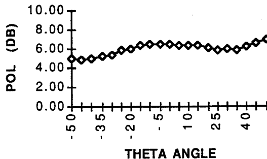
RIGHT TO LEFT CIRCULAR POLARIZATION-1.4 GHZ
