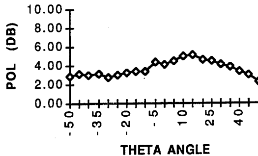
RIGHT TO LEFT CIRCULAR POLARIZATION-0.8 GHZ
