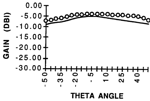
ORIENTATION 1 1.4 GHZ (HTS1)
