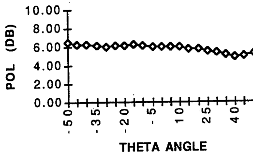
RIGHT TO LEFT CIRCULAR POLARIZATION-1.2 GHZ
