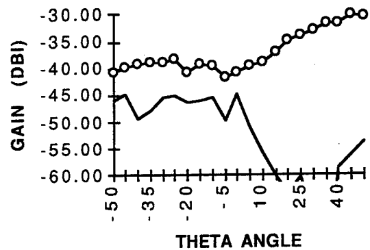
.9 GHZ (ROOM TEMP GOLD)
