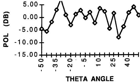
FIGURE 5. Comparative Plots of the Right- to Left-Hand Circular Polarization Ratio.
