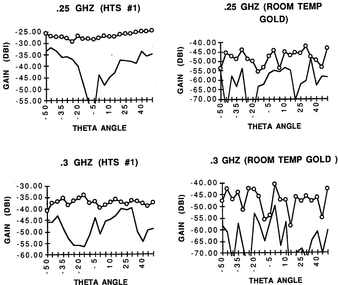
FIGURE 7. 2-Inch Diameter Archimedean Modulated Arm Sprial: HTSC to Normal Metal Comparison.
