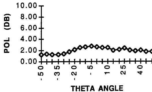
RIGHT TO LEFT CIRCULAR POLARIZATION-0.9 GHZ
