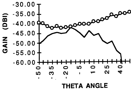
.60 GHZ (HTS1)
