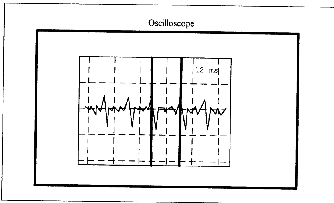
Figure 10 - O-Scope Measurements
