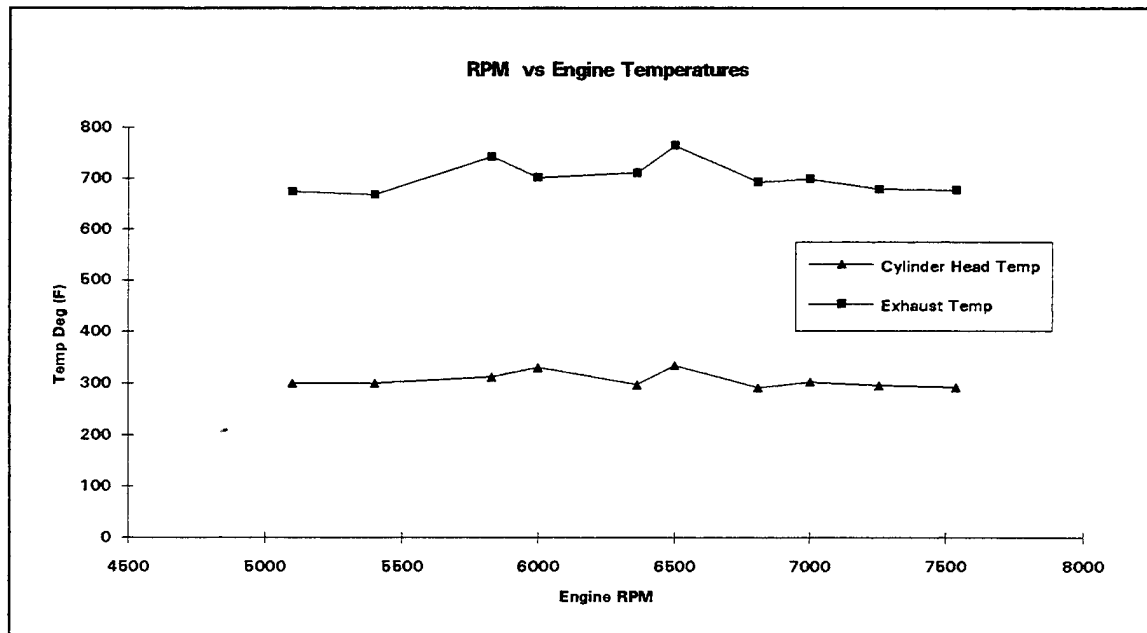
Figure 25 - Temperature Distribution
