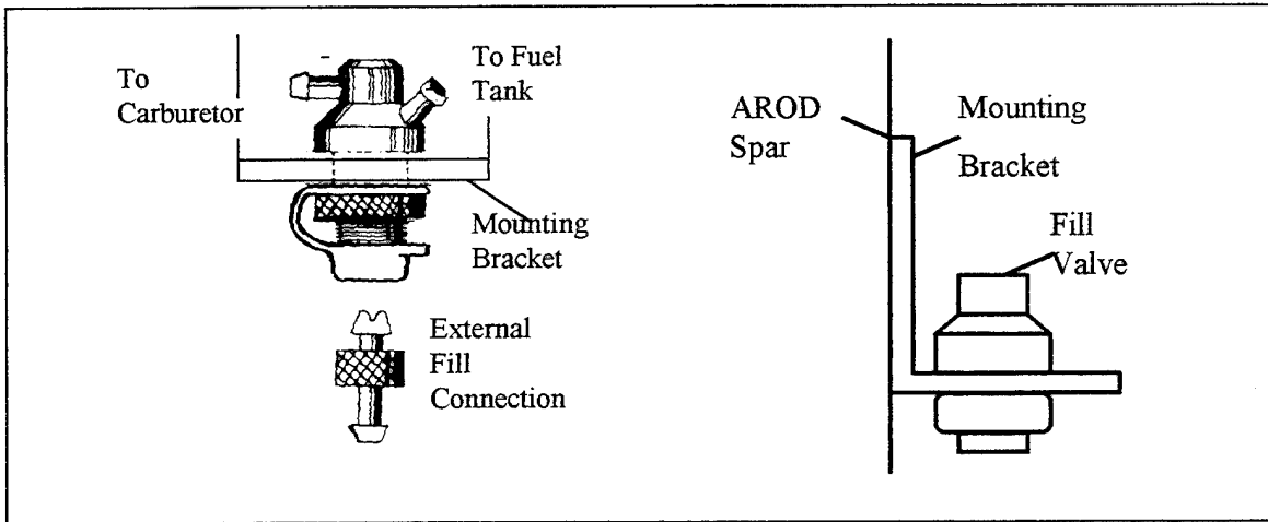
Figure 24- Filling Valve
