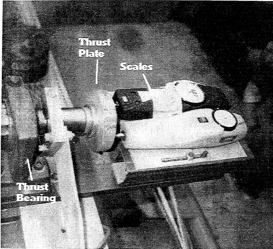
Figure 13 - Thrust Gauges
