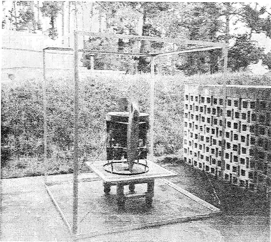
Figure 28 - HTS Construction
