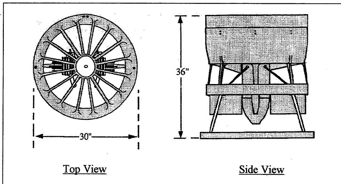
Figure 5 - AROD / ADF Frame
