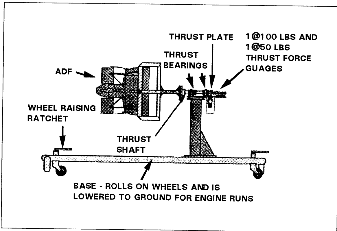
Figure 12 - Thrust Stand
