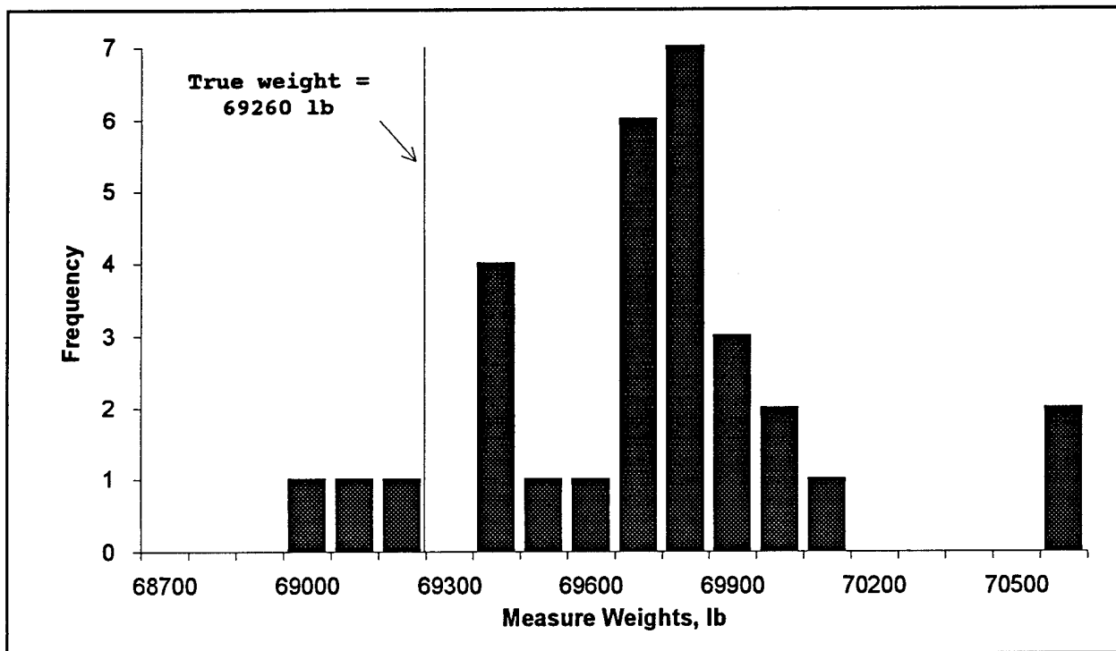
Figure 5-1. Frequency histogram, 3S2 truck (loaded).
