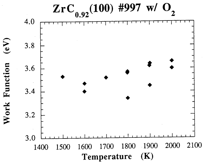
Figure 6. Thermionic effective work function of partially oxygen-covered ZrC_{0.92}(100) .
