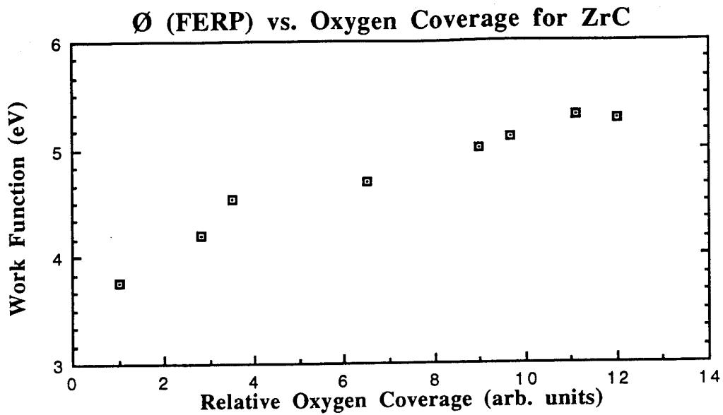
Figure 5. FERP work function of ZrC_{0.92}(100) with adsorbed oxygen.
