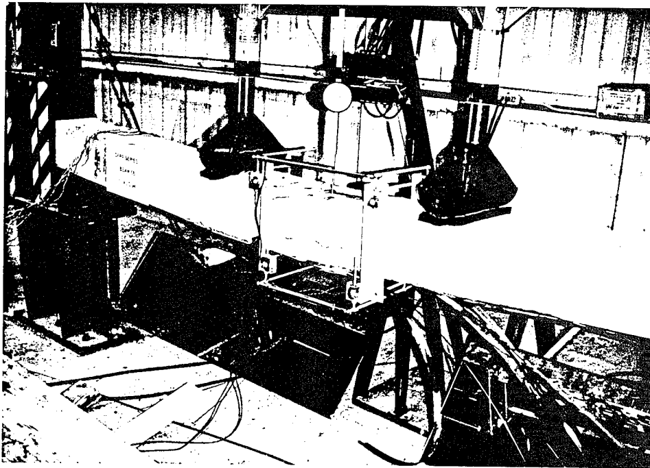
Figure 11. Photograph of beam failure by delamination for a Series 5 beam.
