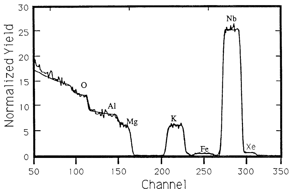
Figure 5 A Rutherford backscattering spectrum of an ion-assisted \text{KNbO}_3 film showing the presence of Fe and Xe impurities.
