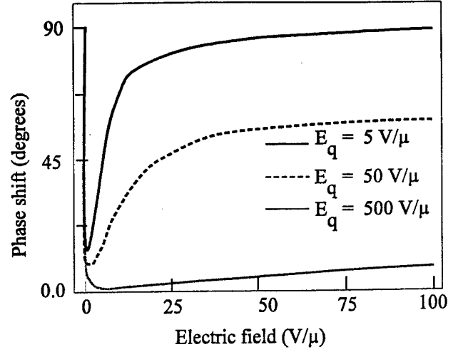
Figure 5 The phase shift of E^1 as a function of an externally applied field, for the same parameters as in Figure 4.
