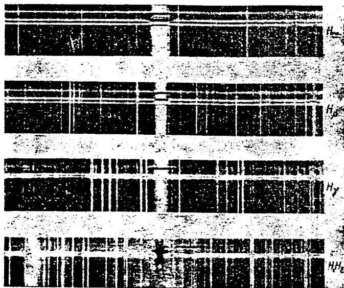
Fig. 4. Fine structure of emissive line reversal in spectrum of solar flare in different lines of hydrogen.
