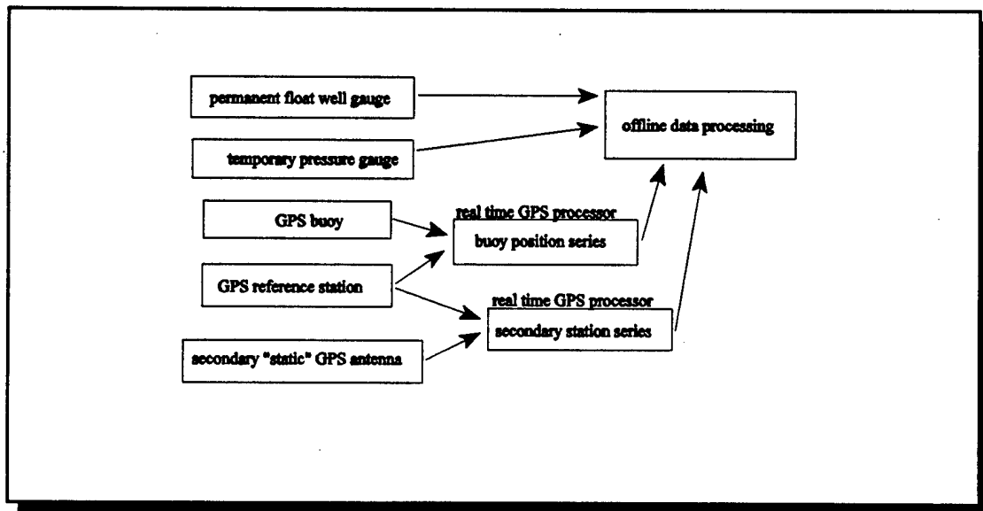
Figure 4.1 Data flow.
