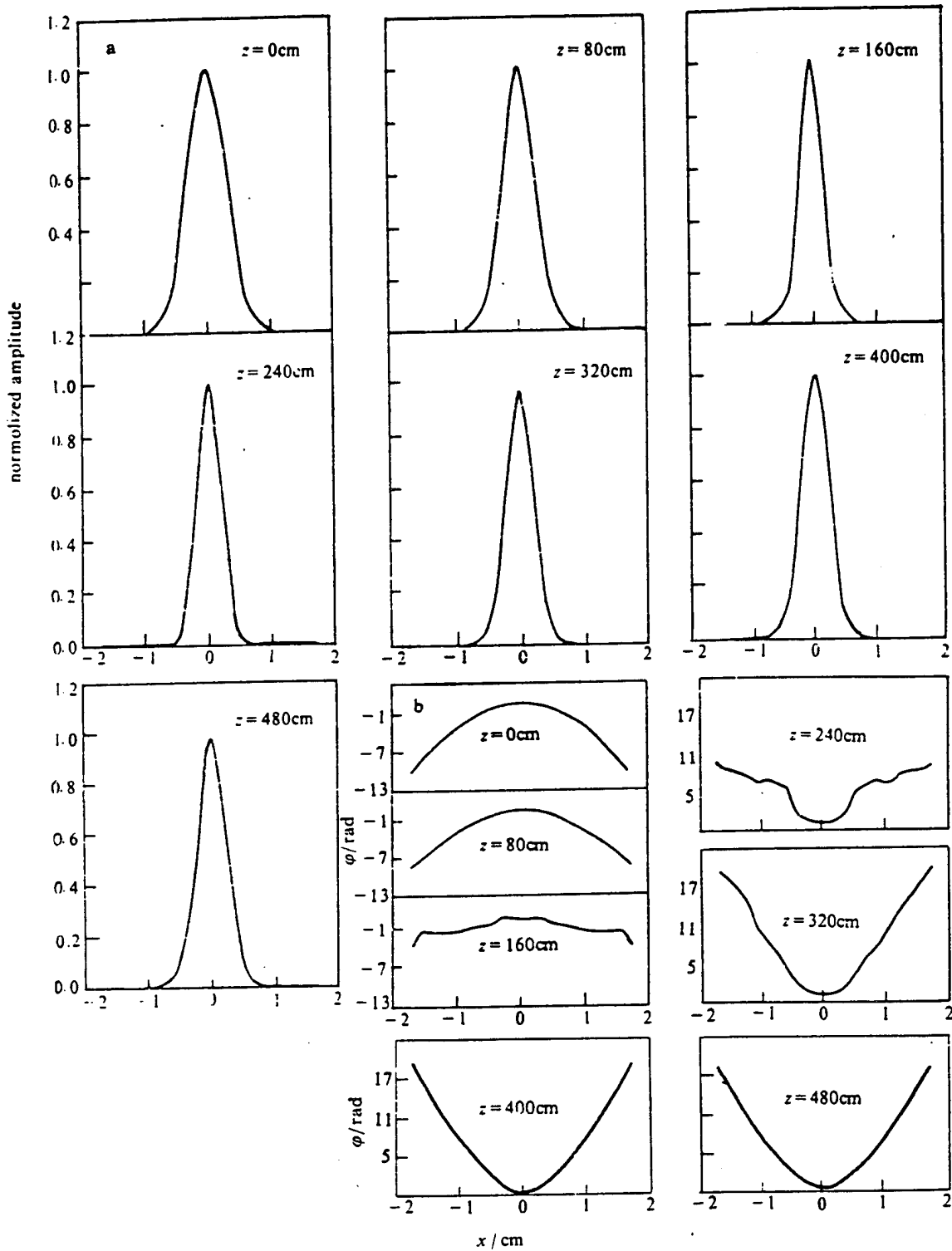
Fig. 5 (a) The evolution of the optical amplitude x - profile ( r_w = 0.444 cm, \gamma_0 = 101.5 ).
