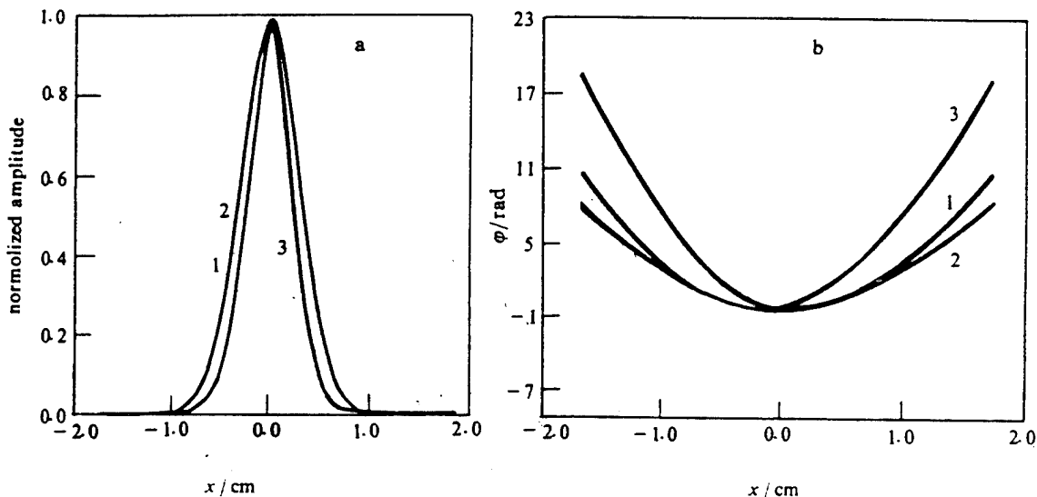
Fig. 1 (a) The comparison of the optical amplitude x - profile of the solution without e - beam. Curve 1 is numerical result ; curve 2 the gaussian fundamental mode. For illumination the corresponding numerical result but with e - beam also is shown in Fig as curve 3. (b) the same but for phase.
