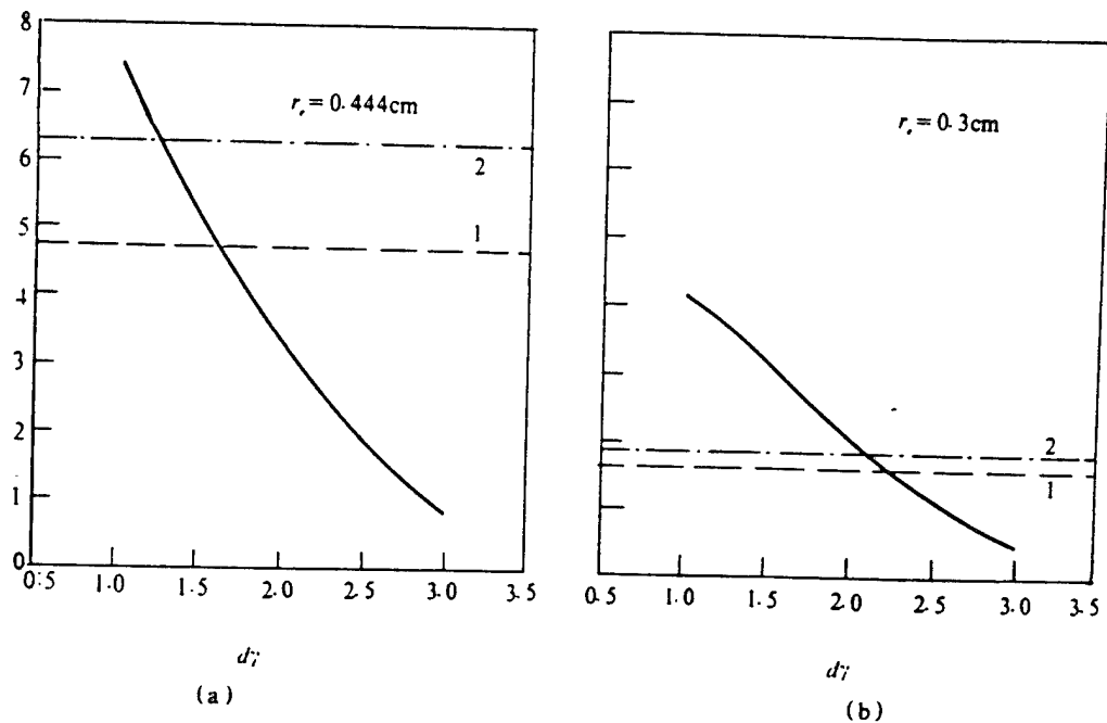
Fig. 8 The determination of the additional equivalent energy spread by the emittance. (\epsilon_v = 0.14\text{cm} \cdot \text{rad} \cdot r_e = 0.444\text{cm}) (see the text)
