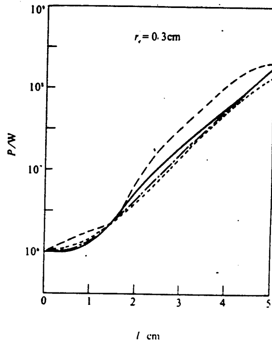
Fig. 3 The evolution of optical power as a function of l - the undulator length. Solid line is the result of ours, dashed line and dotted line are for MICFEL DM , and dot - and - dash line for FRED DM ( r_s = 0.30\text{cm} )
