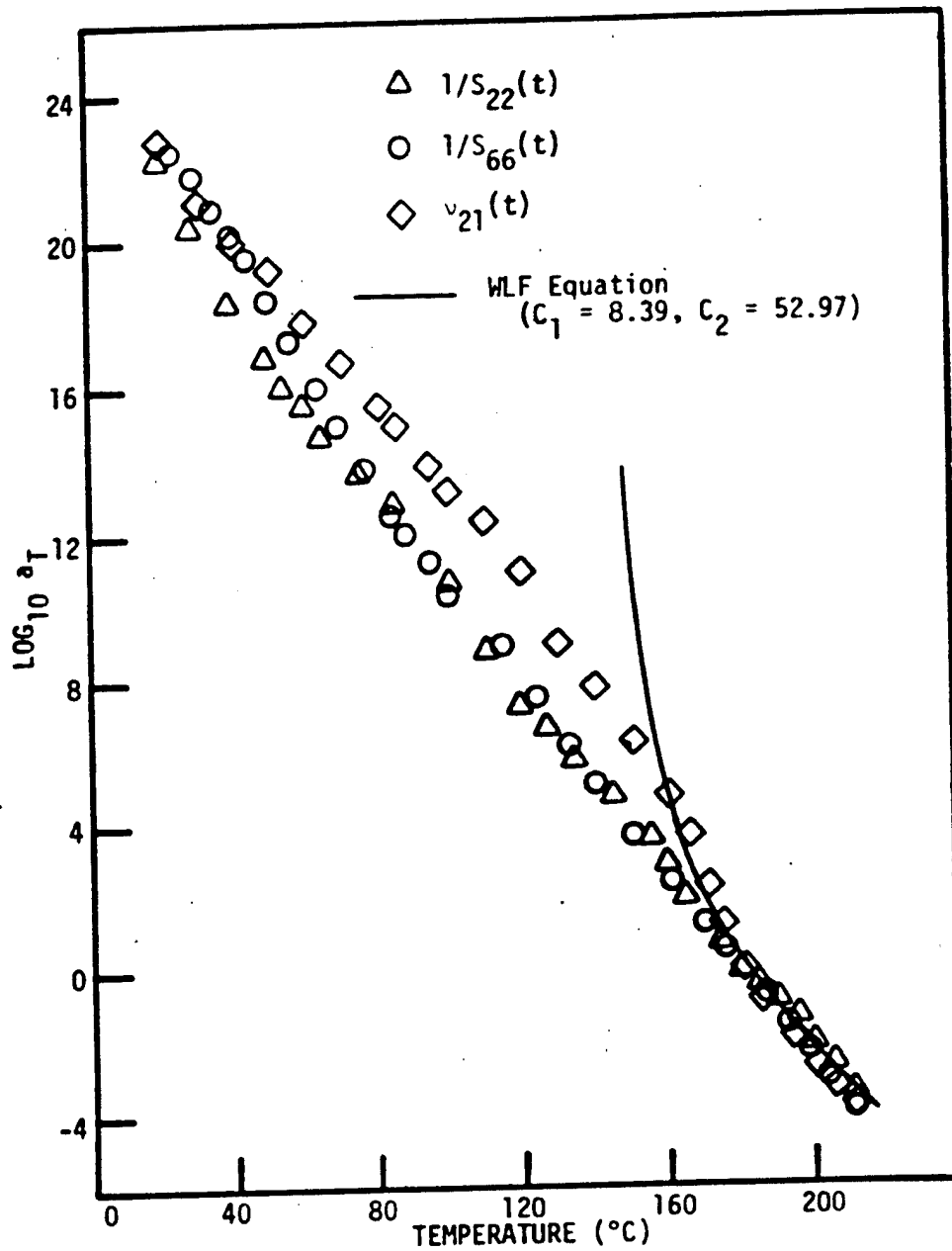
Figure 26. \text{Log}_{10} a_T Versus Temperature.
