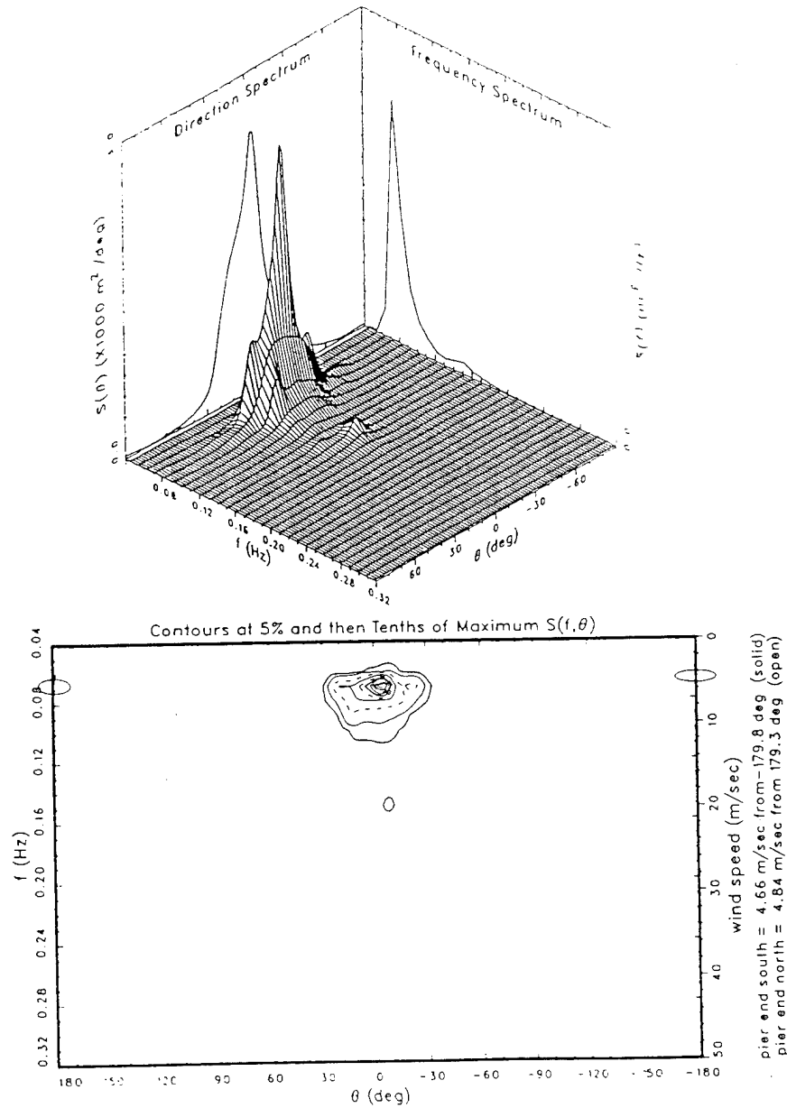
Figure 4.2 Wave spectrum data from Duck, N.C., for 20 Oct 94.
