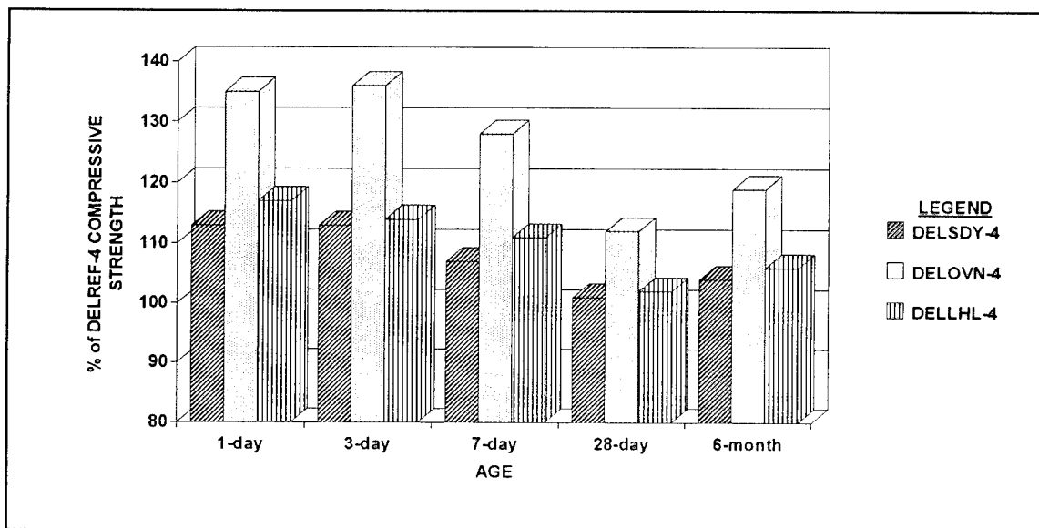
Figure 4. Relative compressive-strength comparison between stabilized mixtures and reference mixture DELREF-4
