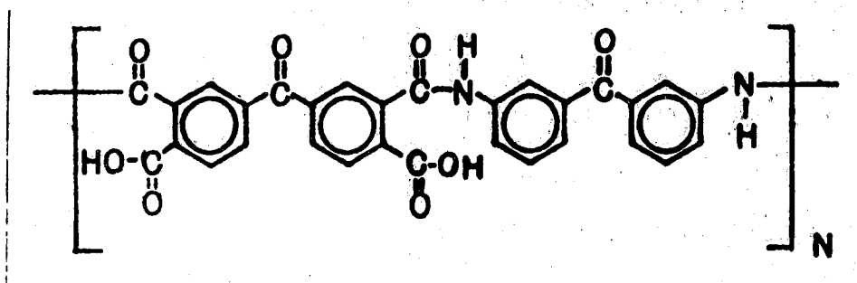
3. LaRC-2(polyamic acid)
