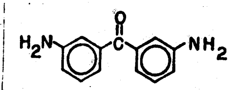
2. m,m'-DABP
