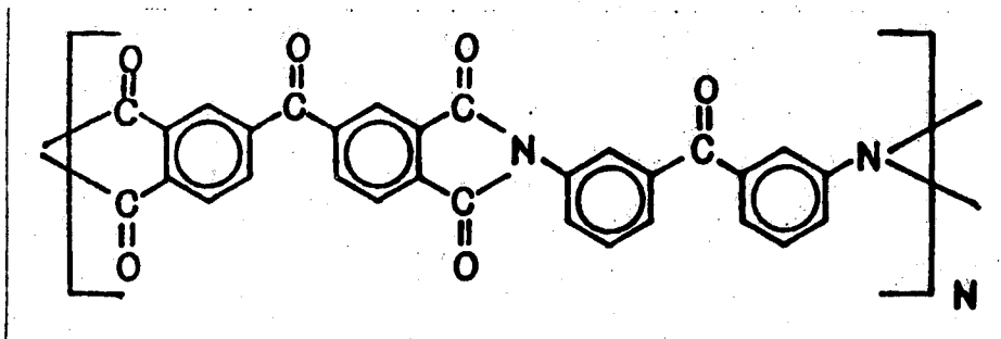
4. LaRC-2 (polyimide)
