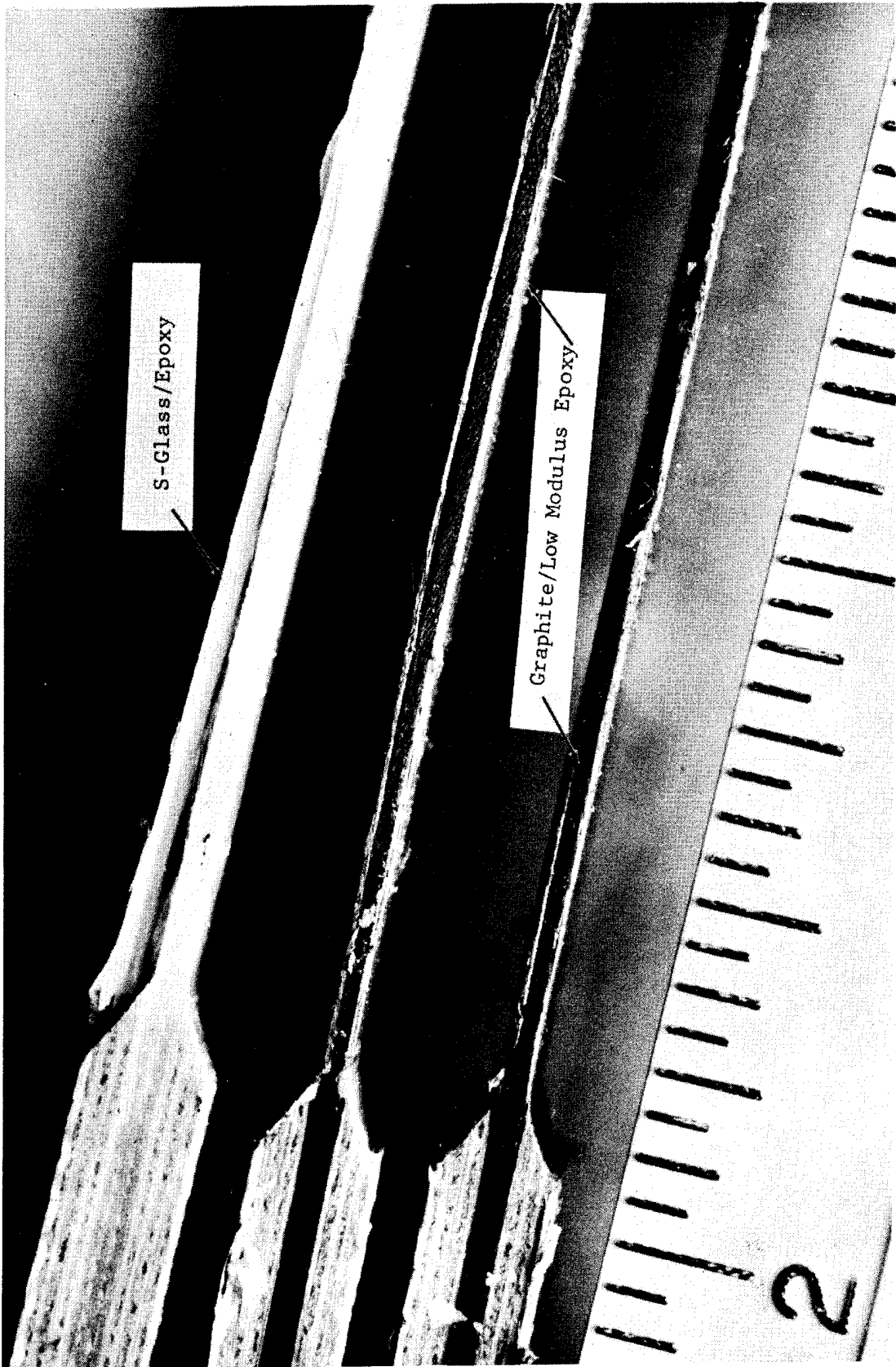
Fig. 5-43 DELAMINATIONS DEVELOPED IN S-GLASS/EPOXY AND GRAPHITE/LOW MODULUS EPOXY SPECIMENS DURING COLD CYCLING WITH TENSILE LOAD.
