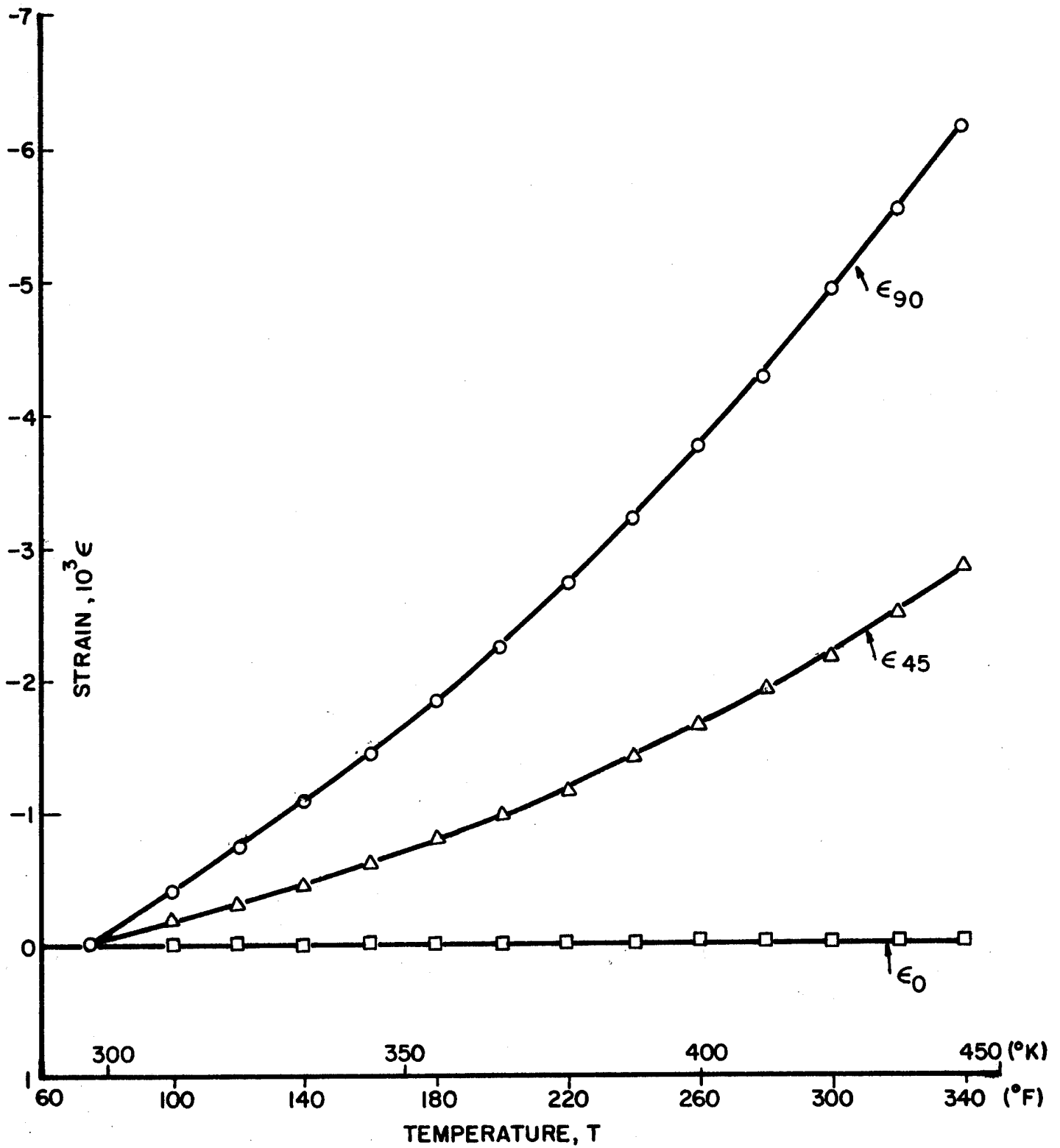
Fig. 3-69 RESTRAINT STRAINS IN 0-DEGREE PLYS OF [0_2/+45]_s GRAPHITE/HIGH MODULUS EPOXY SPECIMEN
