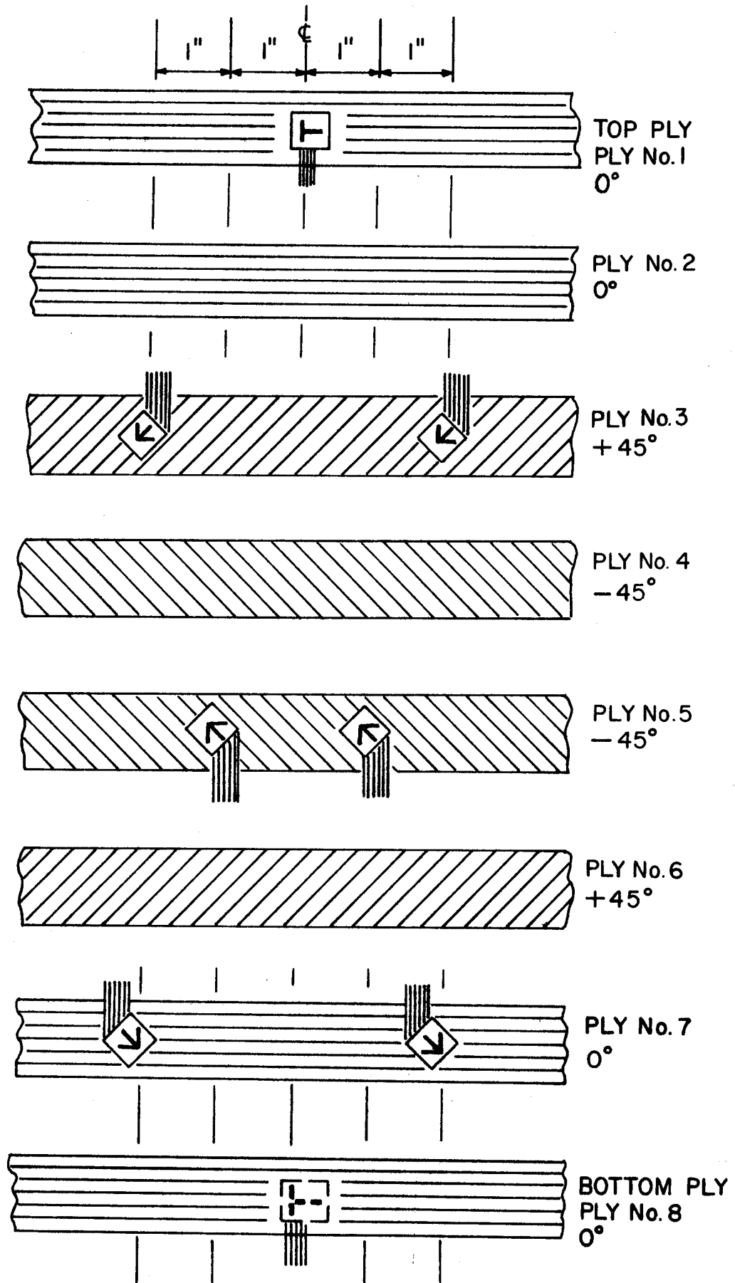
Fig. 3-29 STRAIN GAGE LAYOUT IN [0_2/\pm 45]_8 SPECIMEN
