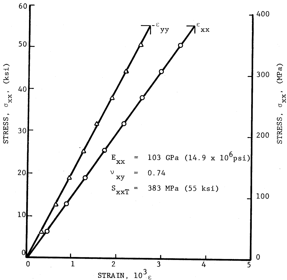
Fig. 5-80 STRESS-STRAIN CURVES FOR [0_2/\pm 45]_s GRAPHITE/HIGH MODULUS EPOXY SPECIMEN UNDER UNIAXIAL TENSILE LOADING AFTER 100 THERMAL CYCLES BETWEEN ROOM TEMPERATURE AND 411 degK ( 280^\circ\text{F} ) UNDER TENSILE LOADING OF 340 MPa (49 ksi)
