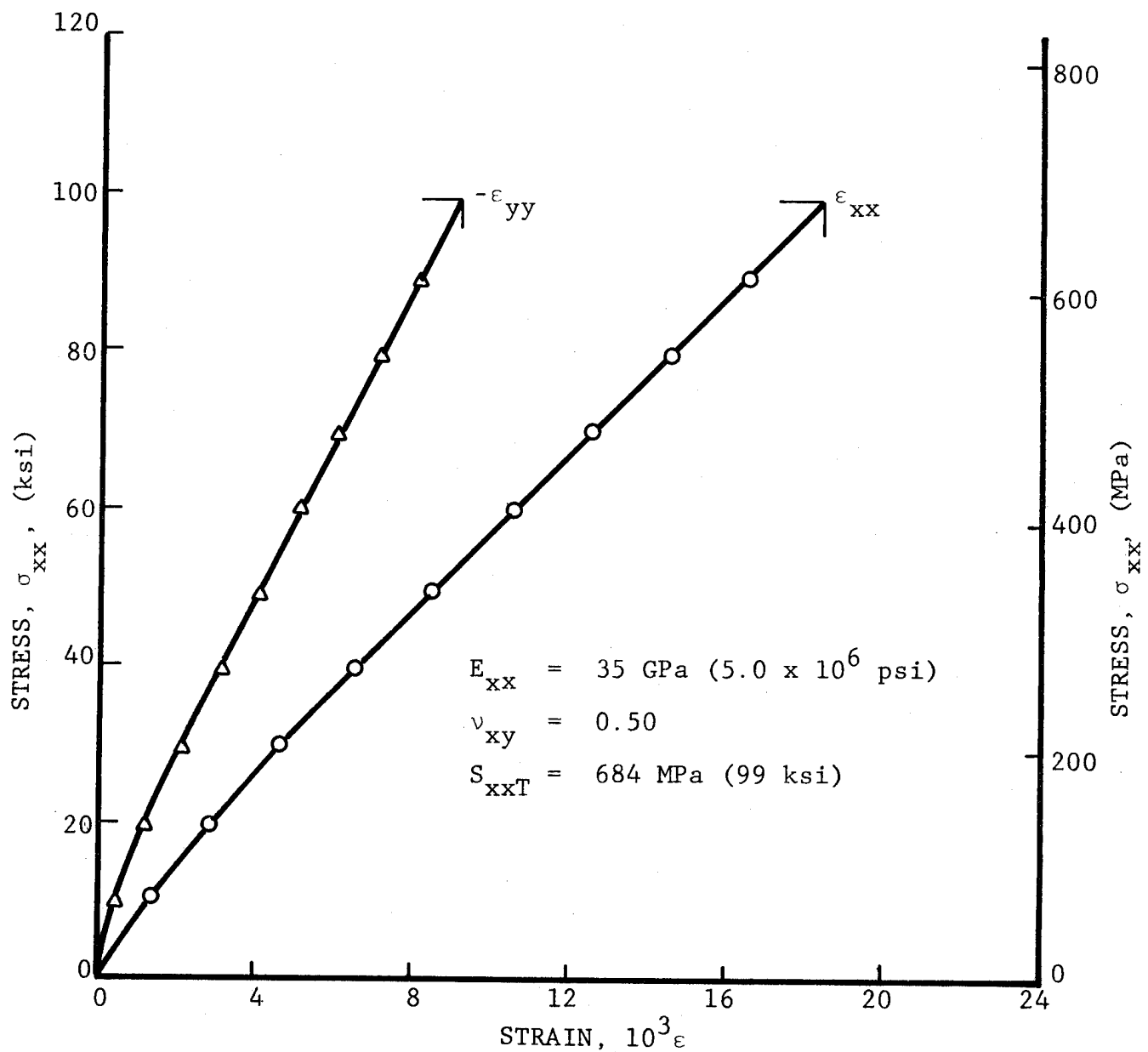
Fig. 5-62 STRAINS IN [0_2/\pm 45]_s S-GLASS/EPOXY SPECIMEN UNDER UNIAXIAL TENSILE LOADING AFTER 100 THERMAL CYCLES BETWEEN ROOM TEMPERATURE AND 200 degK (-100°F)
