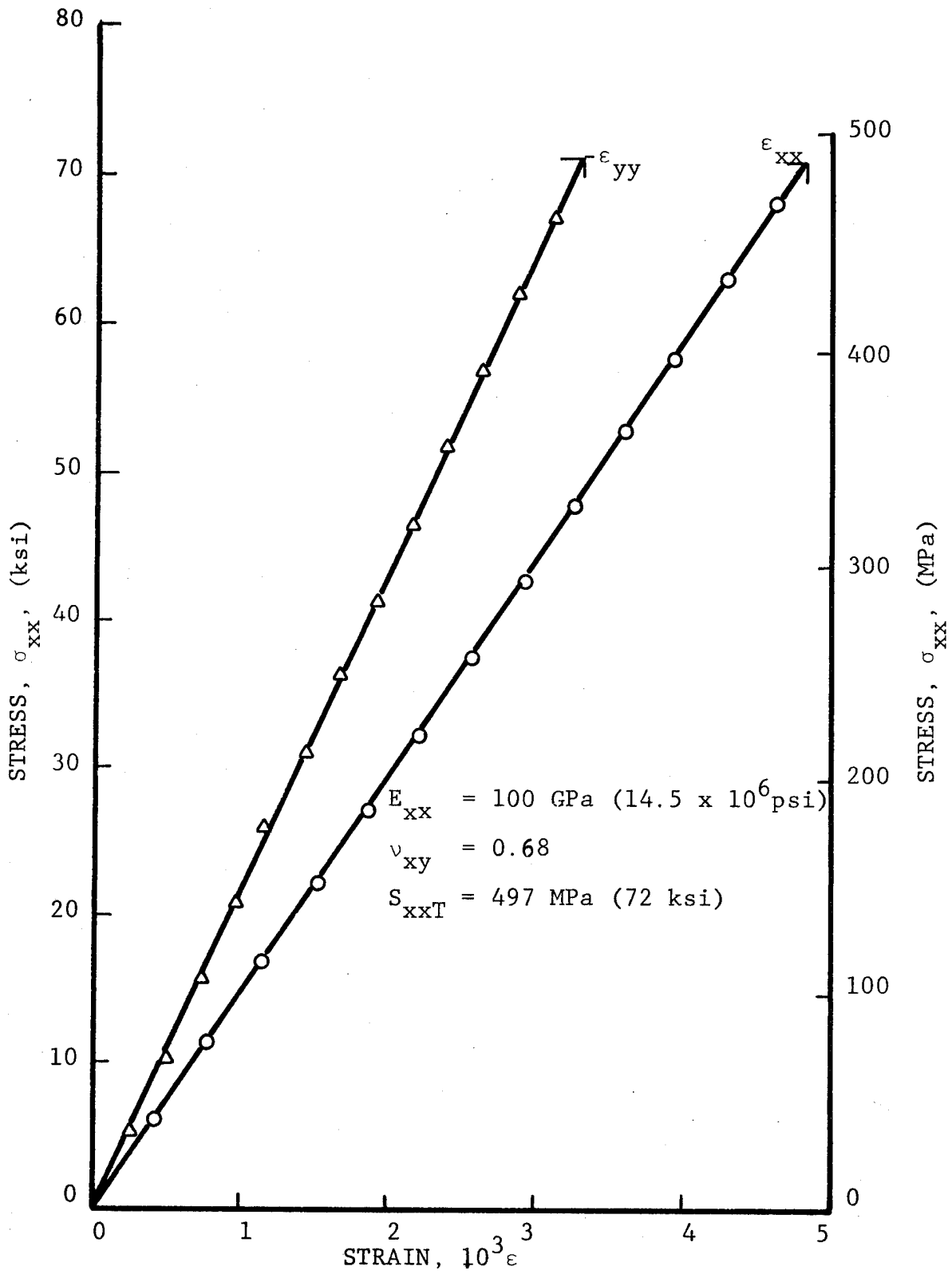
Fig. 5-72 STRESS-STRAIN CURVES FOR [0_2/+45]_s GRAPHITE/HIGH MODULUS EPOXY UNDER UNIAXIAL TENSILE LOADING AFTER 10^7 CYCLES TO 70 PERCENT OF ULTIMATE.
