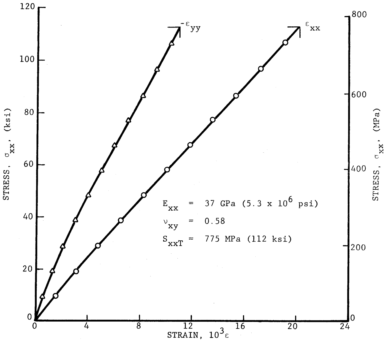
Fig. 5-97 STRAINS IN [0_2/\pm 45]_s S-GLASS/EPOXY SPECIMEN UNDER UNIAXIAL TENSILE LOADING AFTER 100 THERMAL CYCLES BETWEEN ROOM TEMPERATURE AND 200 degK ( -100^\circ\text{F} ) UNDER TENSILE LOADING OF 520 MPa (75 ksi)
