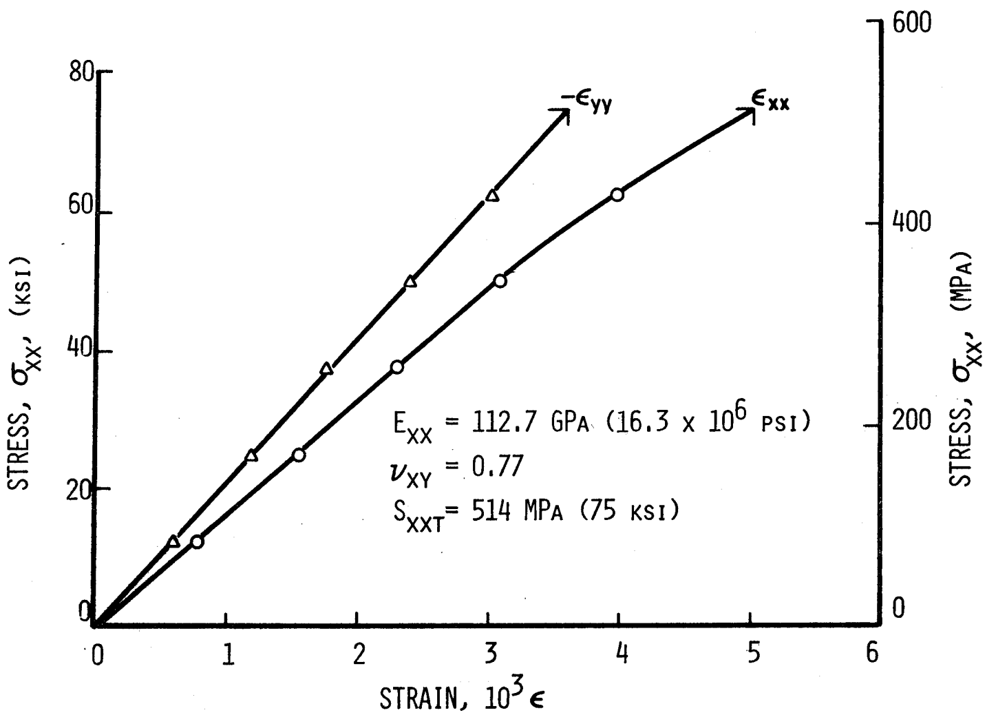
Fig. 4-12 STRAINS IN [O_2/\pm 45]_s BORON/POLYIMIDE SPECIMENS UNDER UNIAXIAL TENSILE LOADING EIGHT MONTHS AFTER CURING
