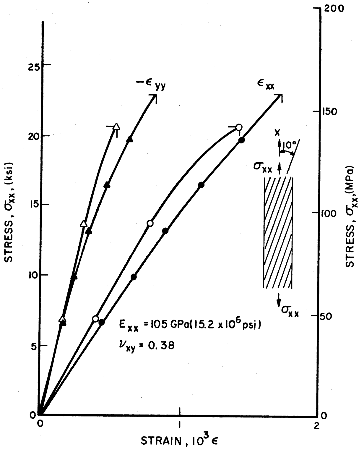
Fig. 3-21 STRESS-STRAIN CURVES IN 10-DEGREE OFF-AXIS UNIDIRECTIONAL BORON/POLYIMIDE SPECIMEN UNDER UNIAXIAL TENSION
