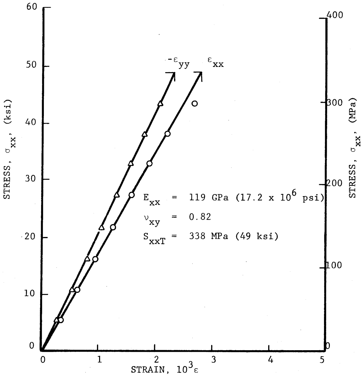
Fig. 5-75 STRESS-STRAIN CURVES FOR [0_2/+45]_s GRAPHITE/POLYIMIDE SPECIMEN UNDER UNIAXIAL TENSION AFTER 10^7 CYCLES TO 70 PERCENT OF ULTIMATE
