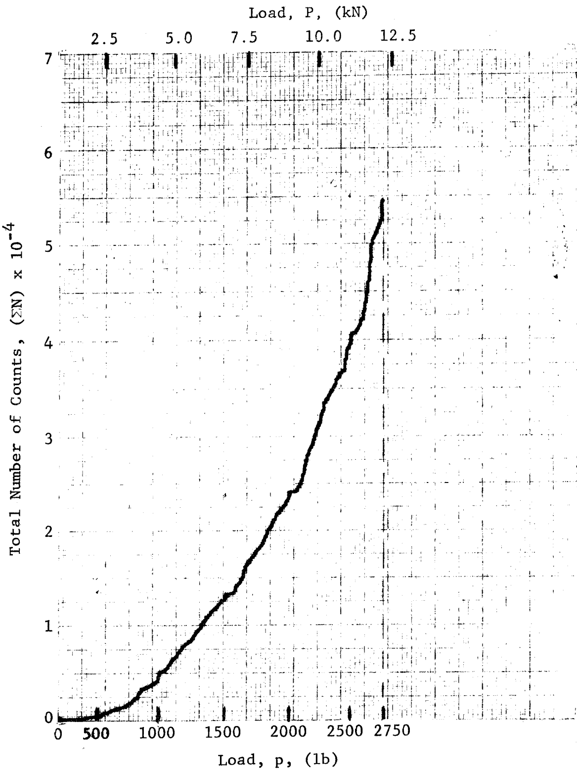
Fig. 3-98 ACOUSTIC EMISSION FOR [0_2/+45]_s GRAPHITE/POLYIMIDE SPECIMEN UNDER TENSILE LOADING
