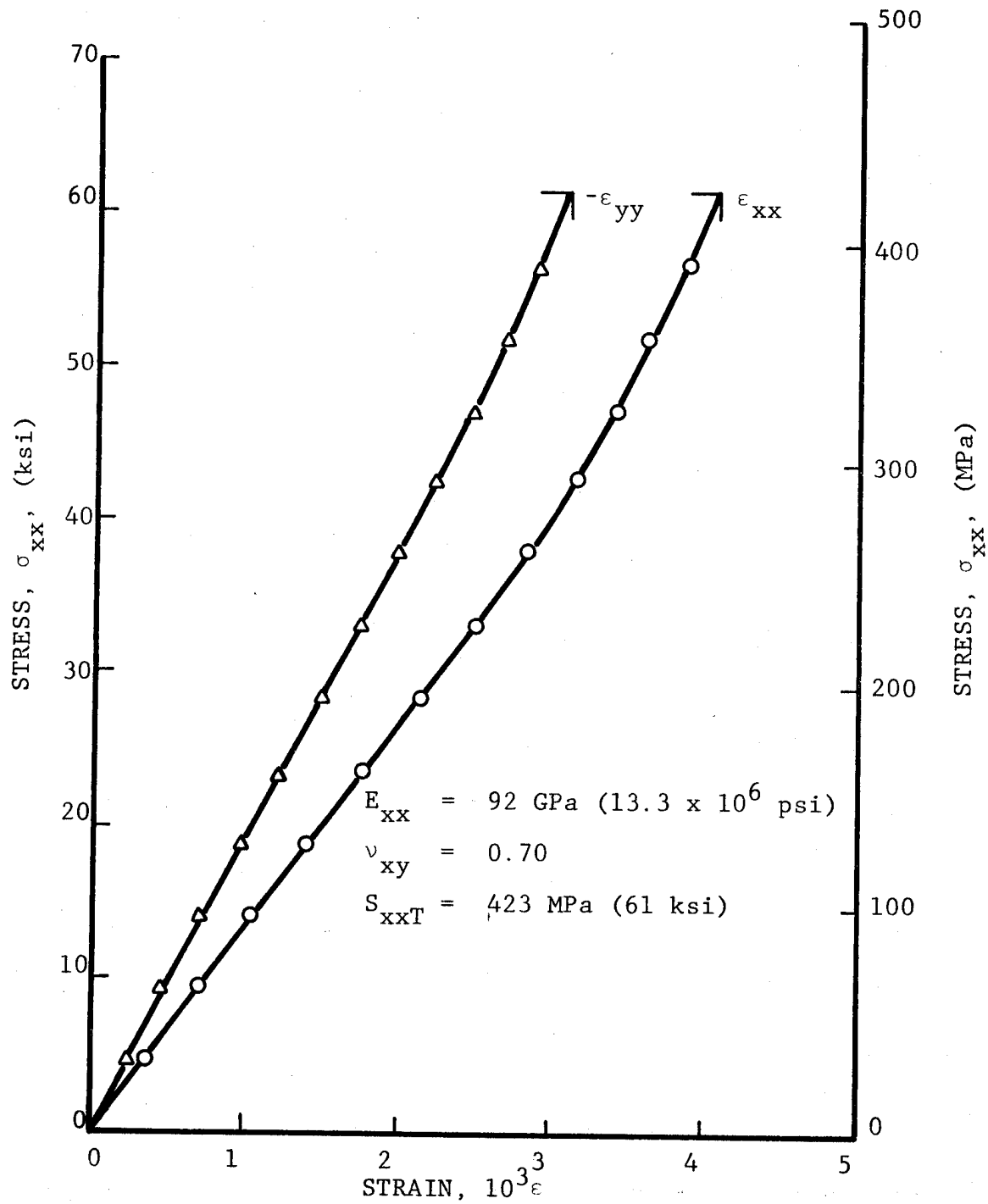
Fig. 5-92 STRAINS IN [O_2/\pm 45]_s GRAPHITE/LOW MODULUS EPOXY SPECIMEN UNDER UNIAXIAL TENSILE LOADING AFTER 100 THERMAL CYCLES BETWEEN ROOM TEMPERATURE AND 200 degK (-100°F) UNDER TENSILE LOADING OF 395 MPa (57 ksi)
