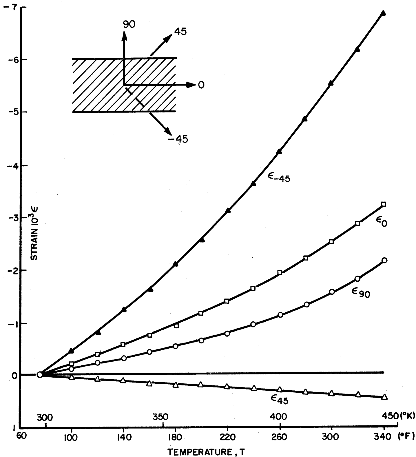
Fig. 3-70 RESTRAINT STRAINS IN 45-DEGREE PLYS OF [0_2/\pm 45]_s GRAPHITE/HIGH MODULUS EPOXY SPECIMEN
