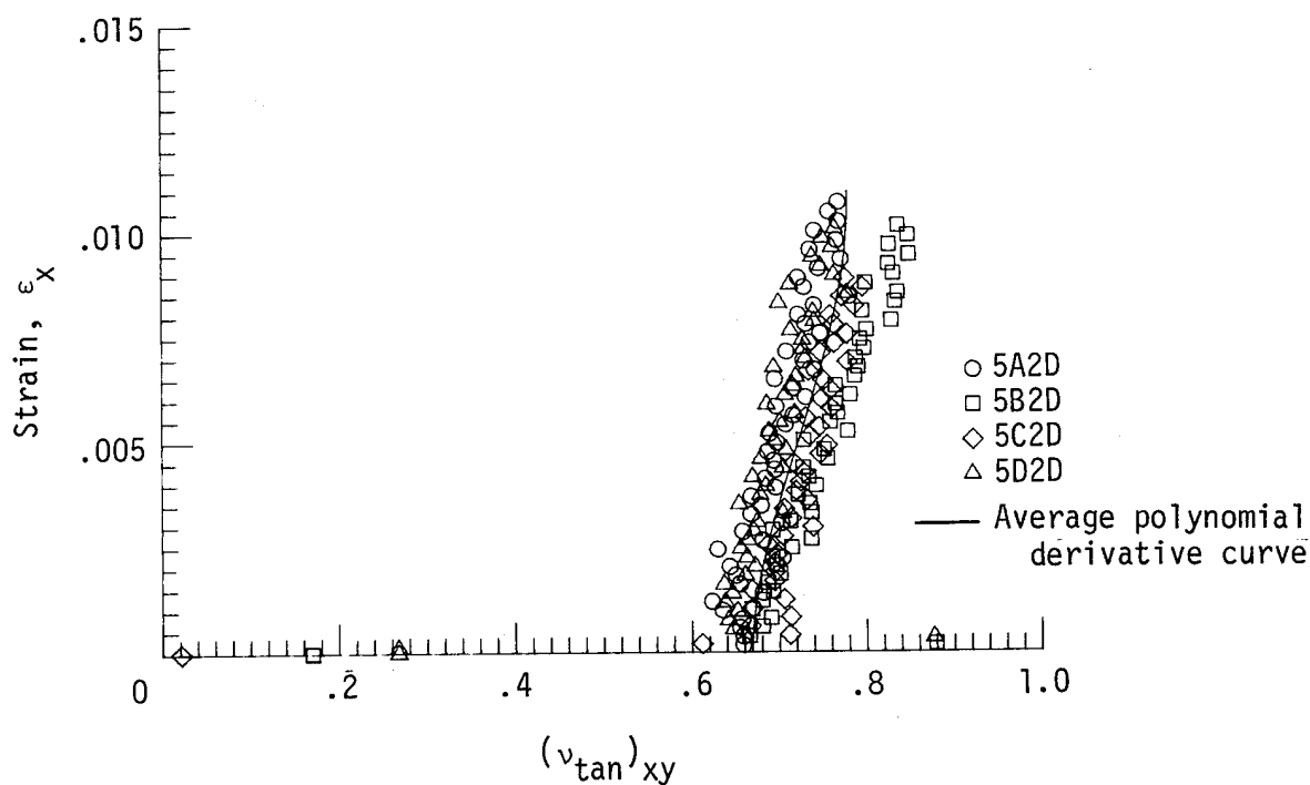
Figure 47. - Tangent modulus and Poisson's ratio for [\pm 45/0/\pm 45/0]_S and [\pm 45/0/\mp 45/0/\pm 45/0/\pm 45]_T laminates.
