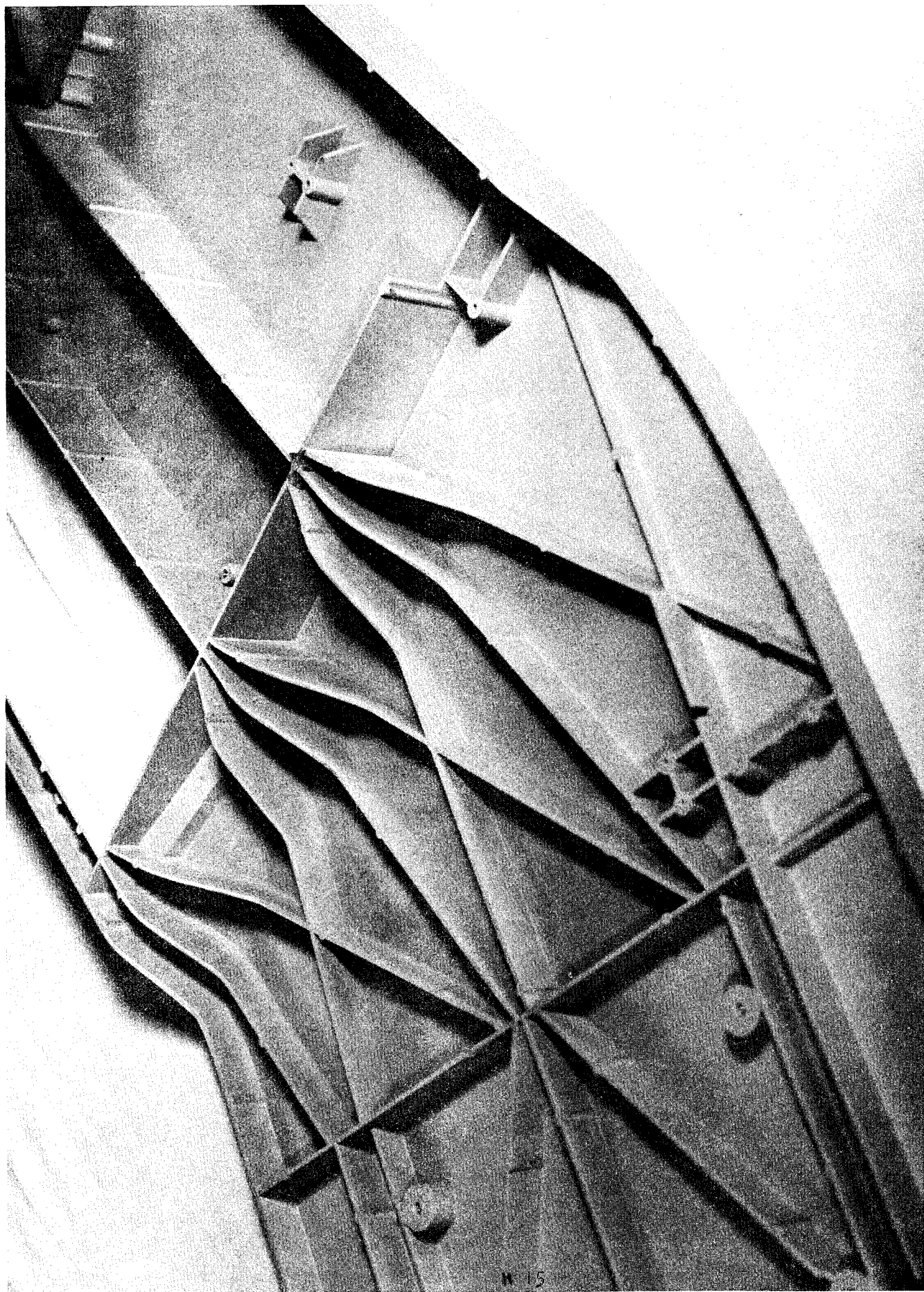
Figure 2. Underside of Desktop shows ribs and bosses for strengthening.
