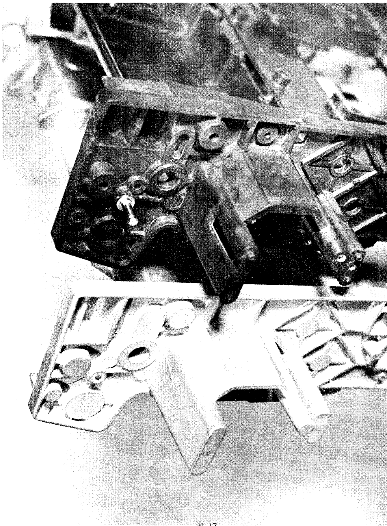
Figure 4. Detail of business machine frame member of aluminum sand casting compared with the replacement molded of BMC.
