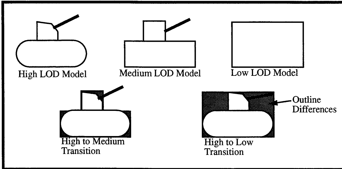
Figure 3. Effect of Differing Outlines on Model Switching
