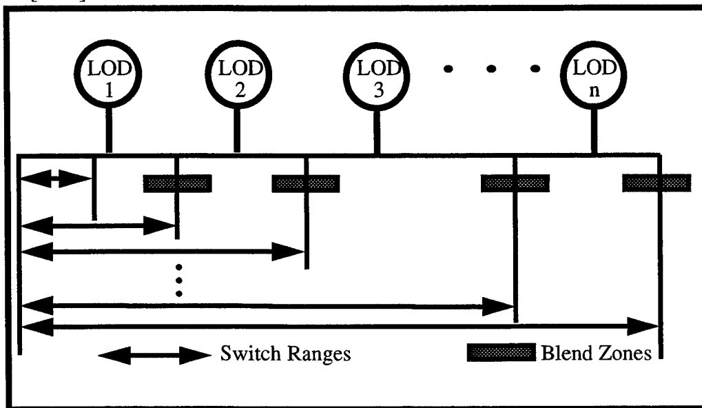
Figure 5. Level of Detail Processing [IRIS]
