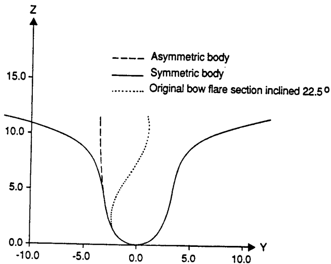
Fig. 3-30. Effect of Velocity Time History and Body Geometry on Free-Surface Elevation and Pressure Distribution on the Cross Section With Bow Flare at Final Time of Numerical Simulation (a) Results of simulation (b) Impact velocity time history (c) Cross sections of model used in numerical simulation
