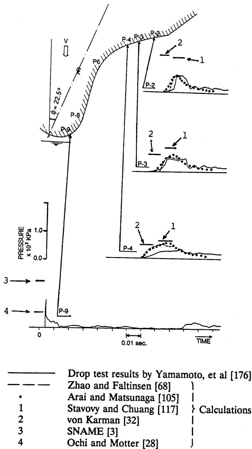
Fig. 6-4. Comparisons Between Numerical and Experimental Pressure Measurements on Bow Flare Section
