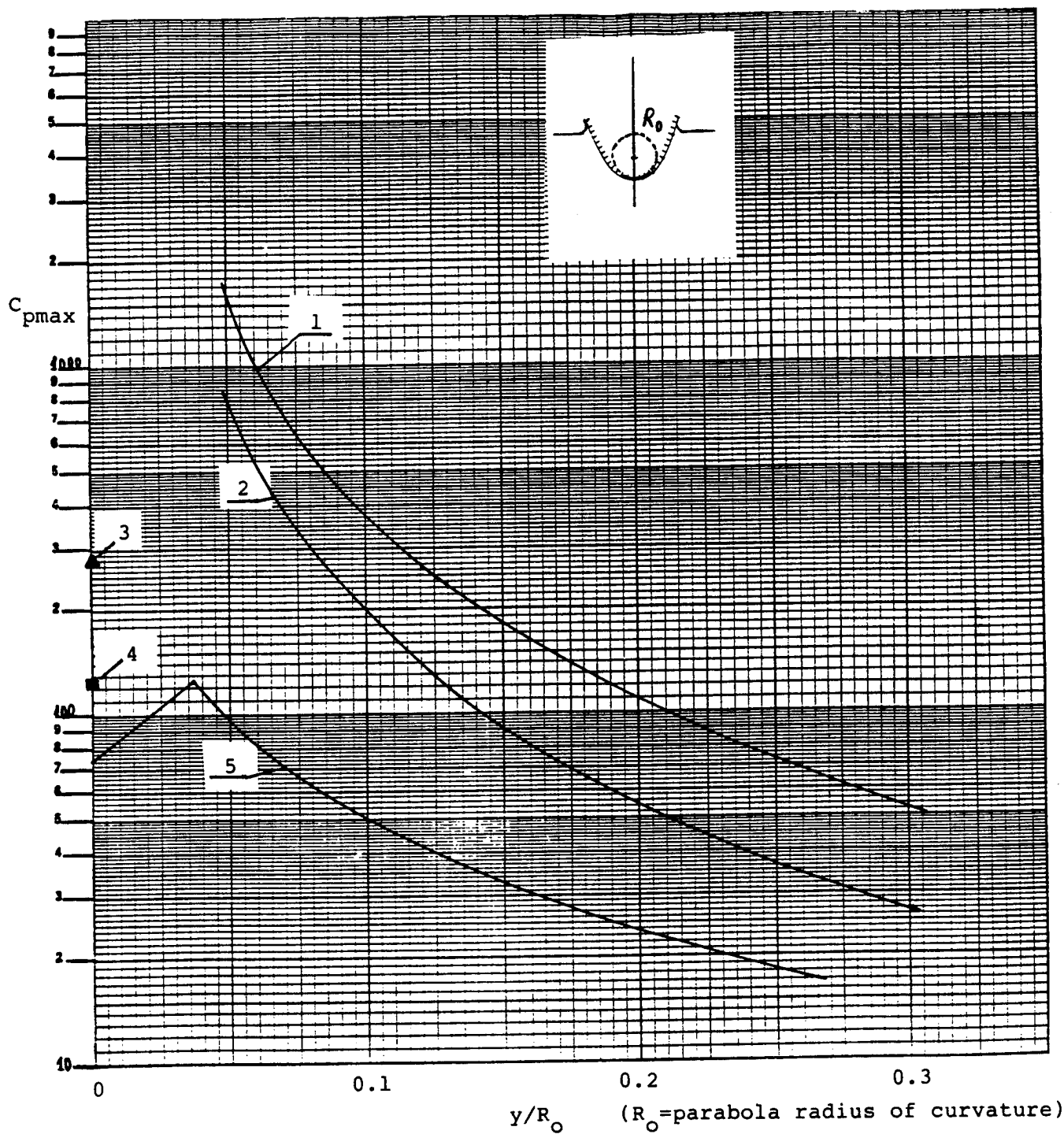
Fig. 6-3. Comparison of Maximum Pressure Coefficient for Parabolic Section as Determined by Various Methods
