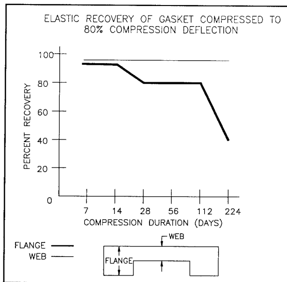
Figure 39. Results of gasket compression test
