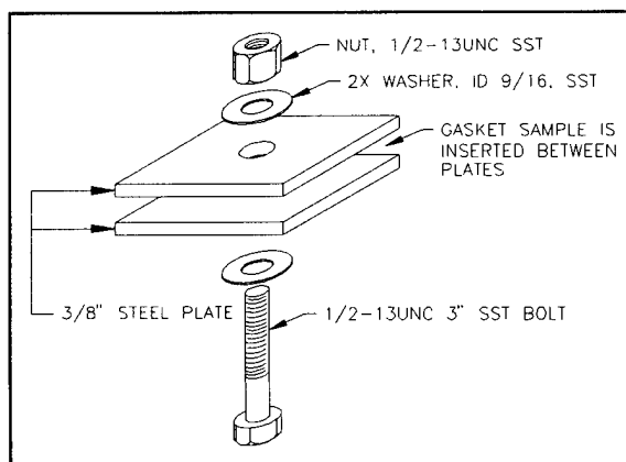
Figure 38. Gasket compression device
