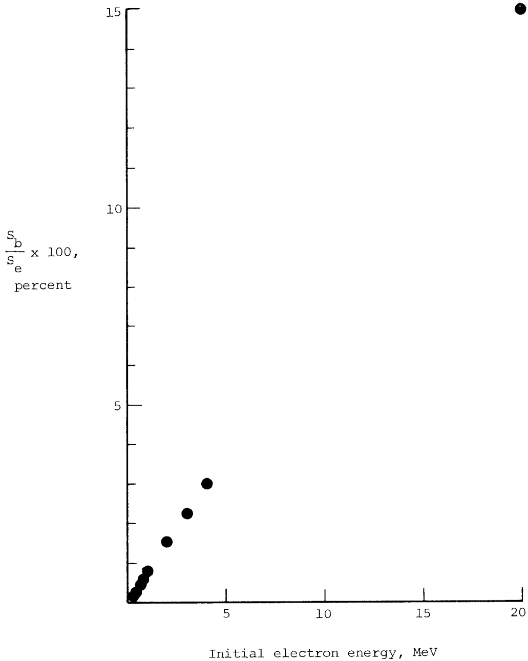
Figure 13.- Ratio of electron energy loss in CMOSH1 due to bremsstrahlung S_b , to energy loss due to inelastic scattering S_e .
