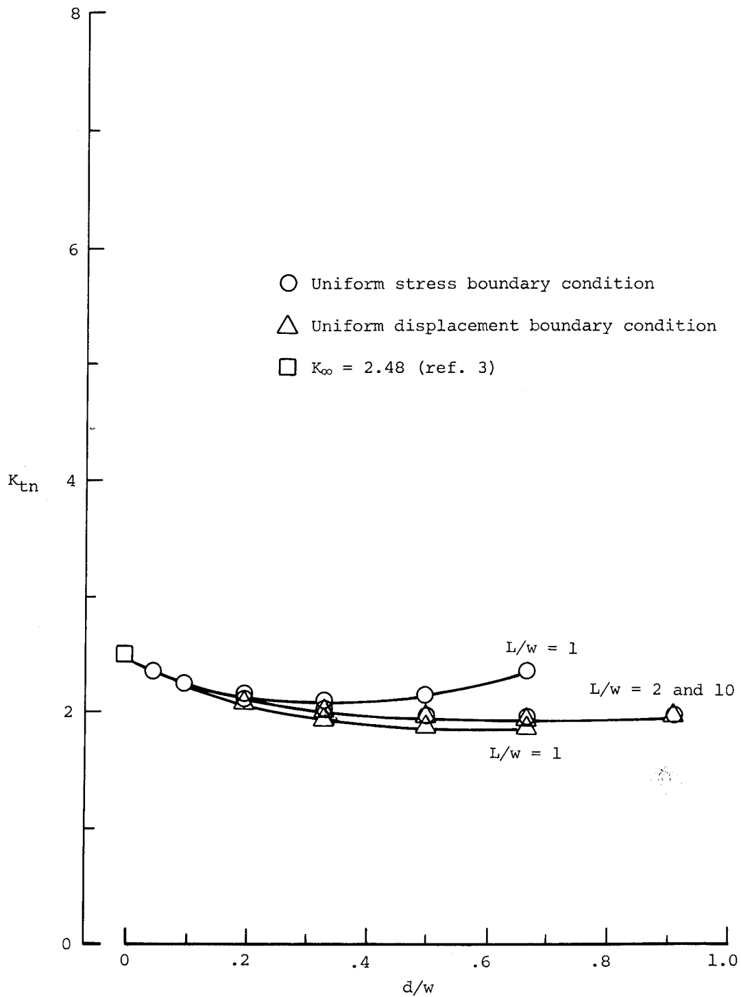
Figure 11.- Stress-concentration factors for a 90^\circ laminate with a circular hole.
