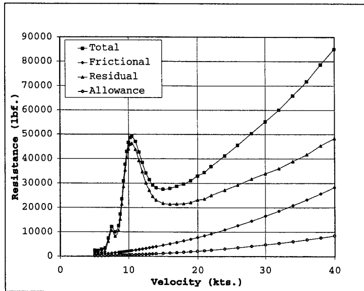
Figure 4.2. ITTC ship resistances versus ship velocity for a single length analysis of the SLICE hull.
