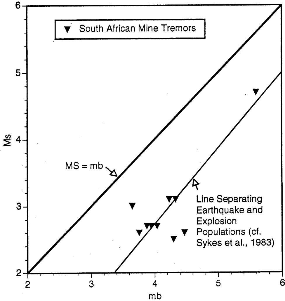
Figure 16. MS versus mb inferred for some recent South African mine tremors based on comparison of long-period amplitude levels observed at station BOSA for the events relative to similar amplitude levels for the October 30, 1994 tremor (4.7 MS). Note that MS values for several smaller events are estimated as upper bounds.
