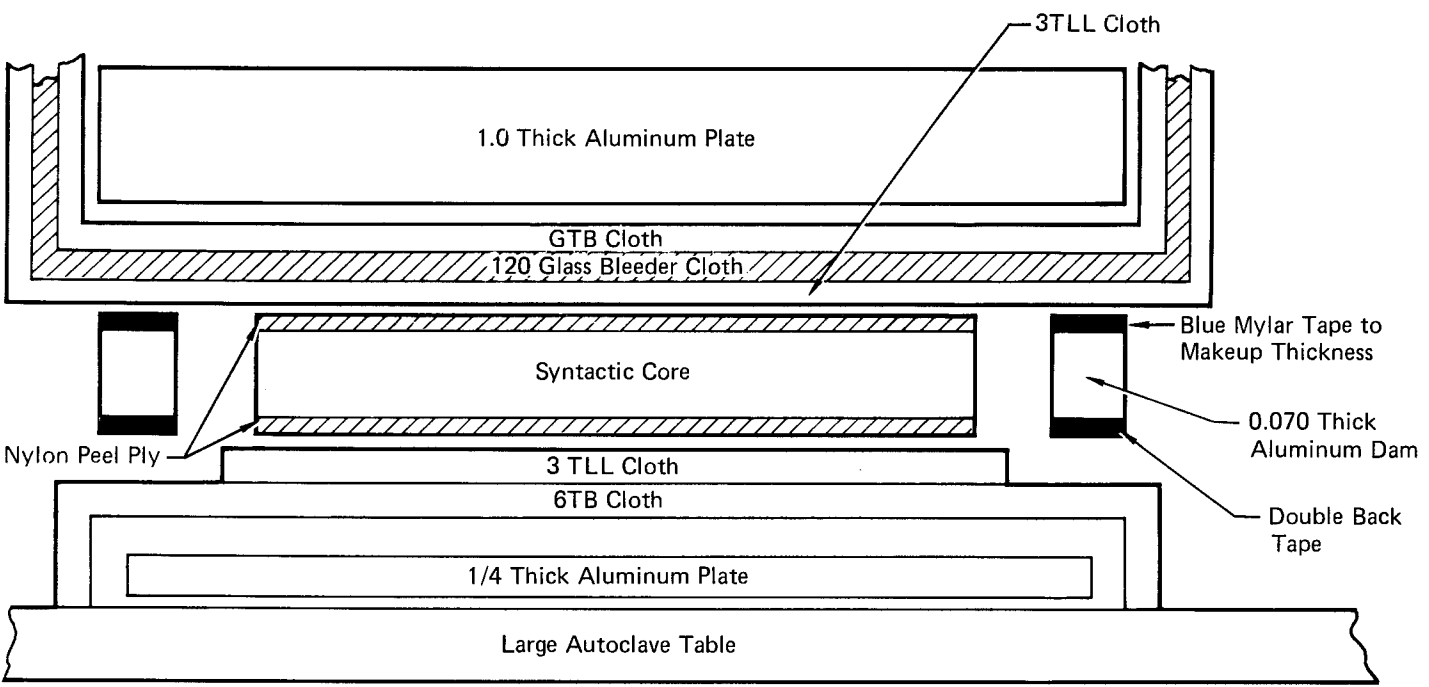
Figure 4. Autoclave Layup for Syntactic Core Sheet
