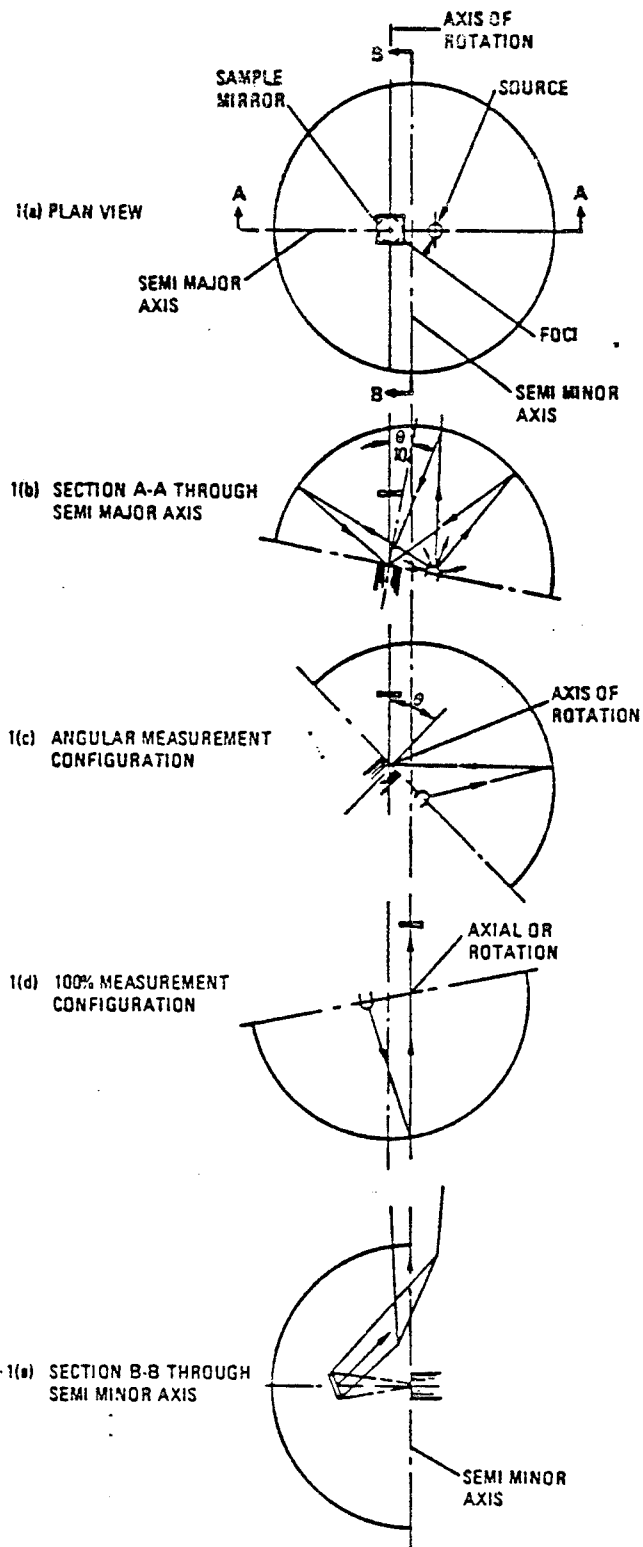
Figure 13. Ellipsometer System
