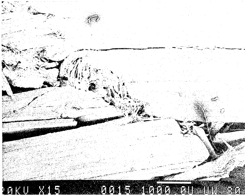
Figure 6.4 Specimen No. XIX-ACL-4211B-13-42, C-C", 218FW; Longitudinal Sawcut Section
