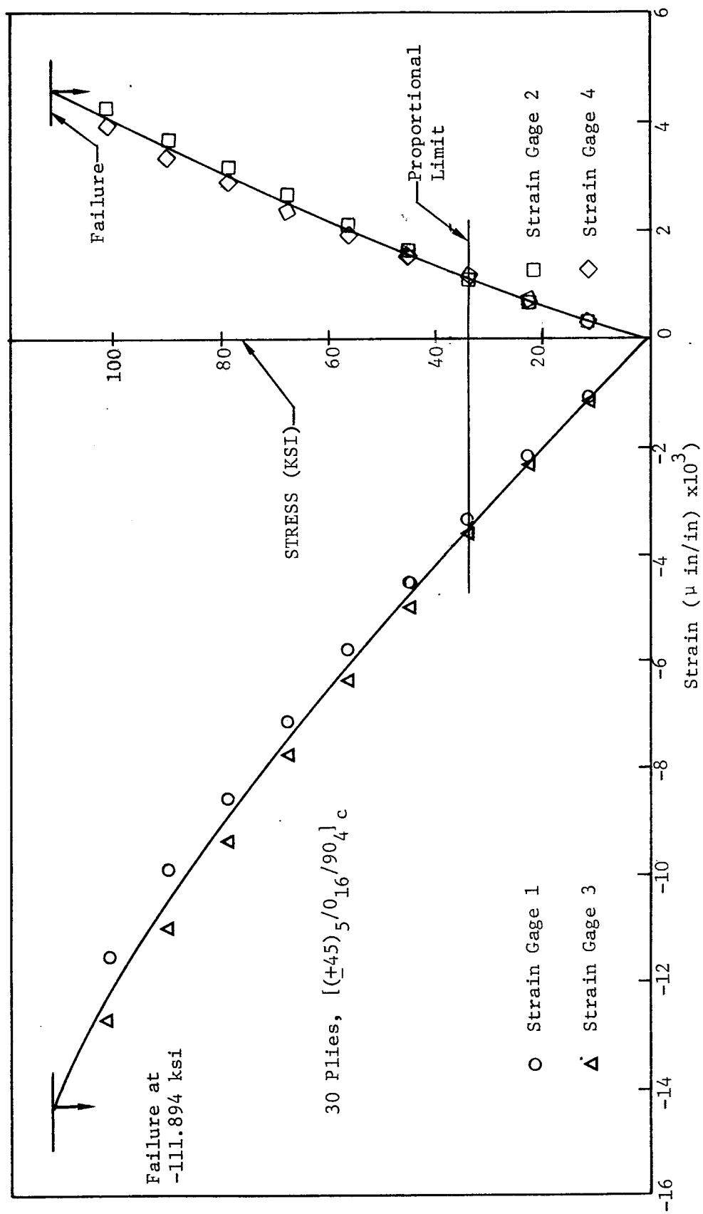
Figure 5.2 0^\circ Static Compression Test Series I, Specimen ACL 4210A-1-6 Stress-Strain Curves, -65FW, Plain Laminate
