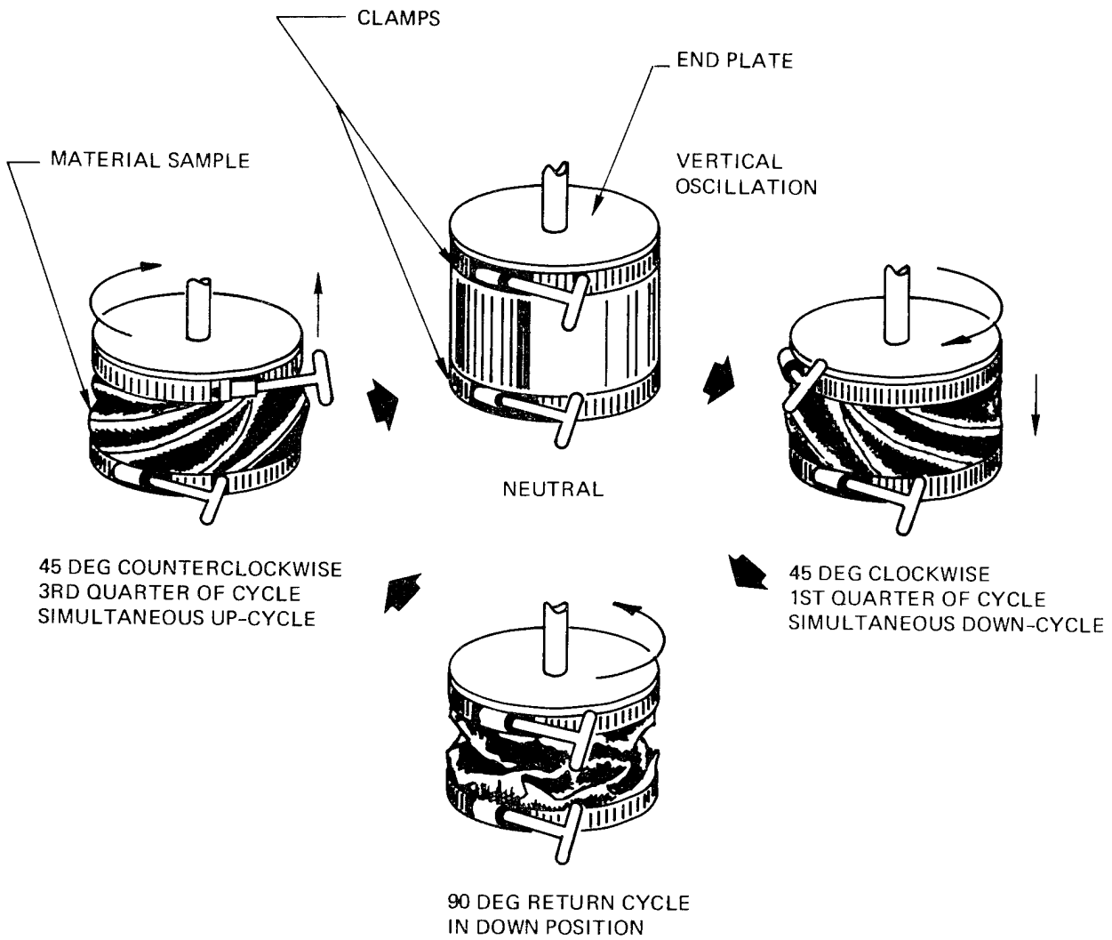
Figure 17 : TWIST-FLEX ACTION
