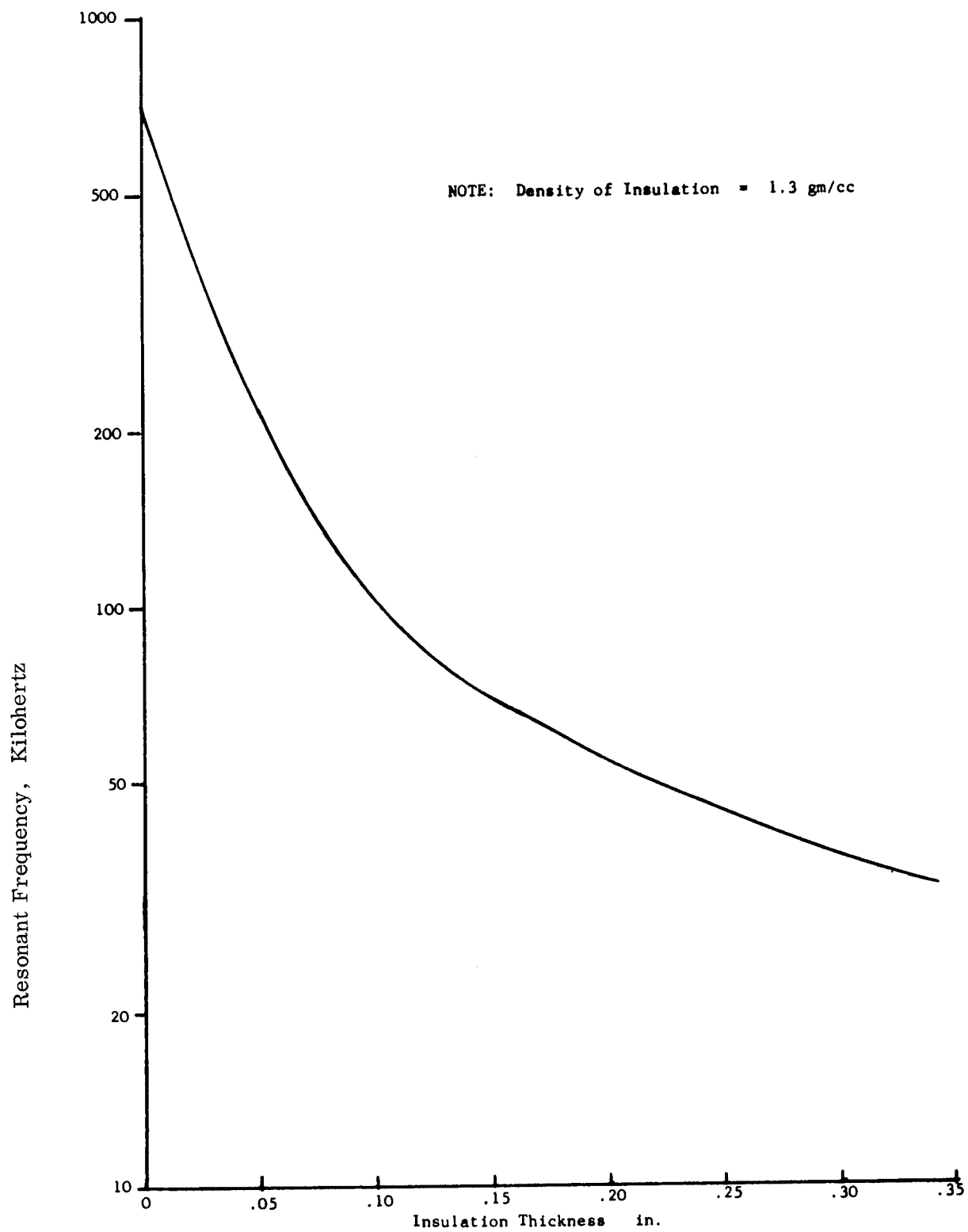
Figure 51. Lowest Resonant Frequency as a Function of Insulation Thickness
