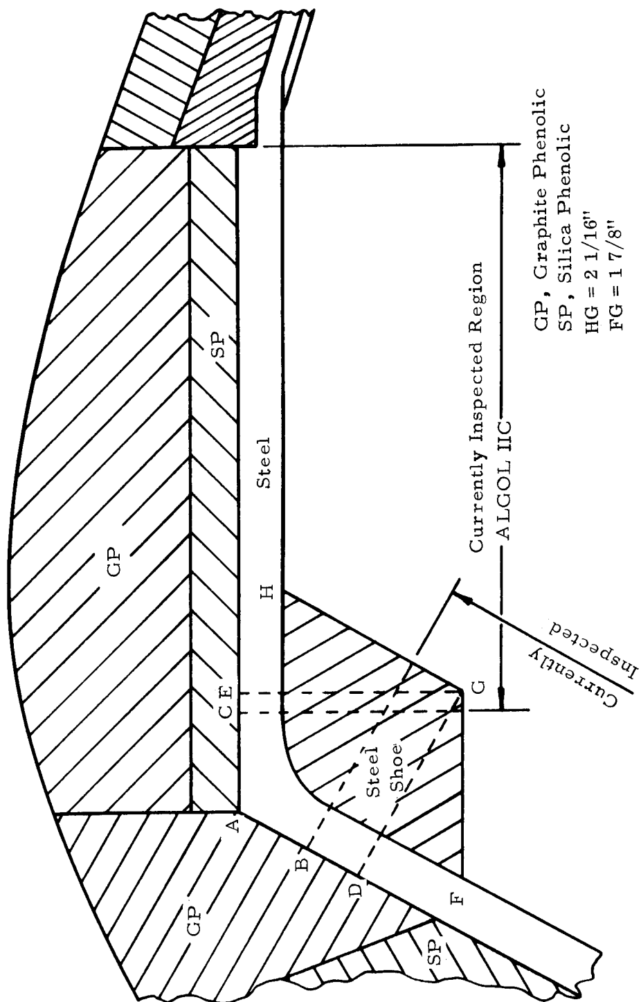
Figure 4. Proposed Advanced Ultrasonic Inspection Technique for ALGOL IIC Nozzle
