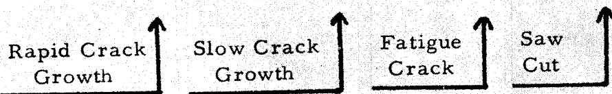
Fracture Cross Section of Epoxy-Novolac (with Elastomeric Second Phase) Specimen - 10X
