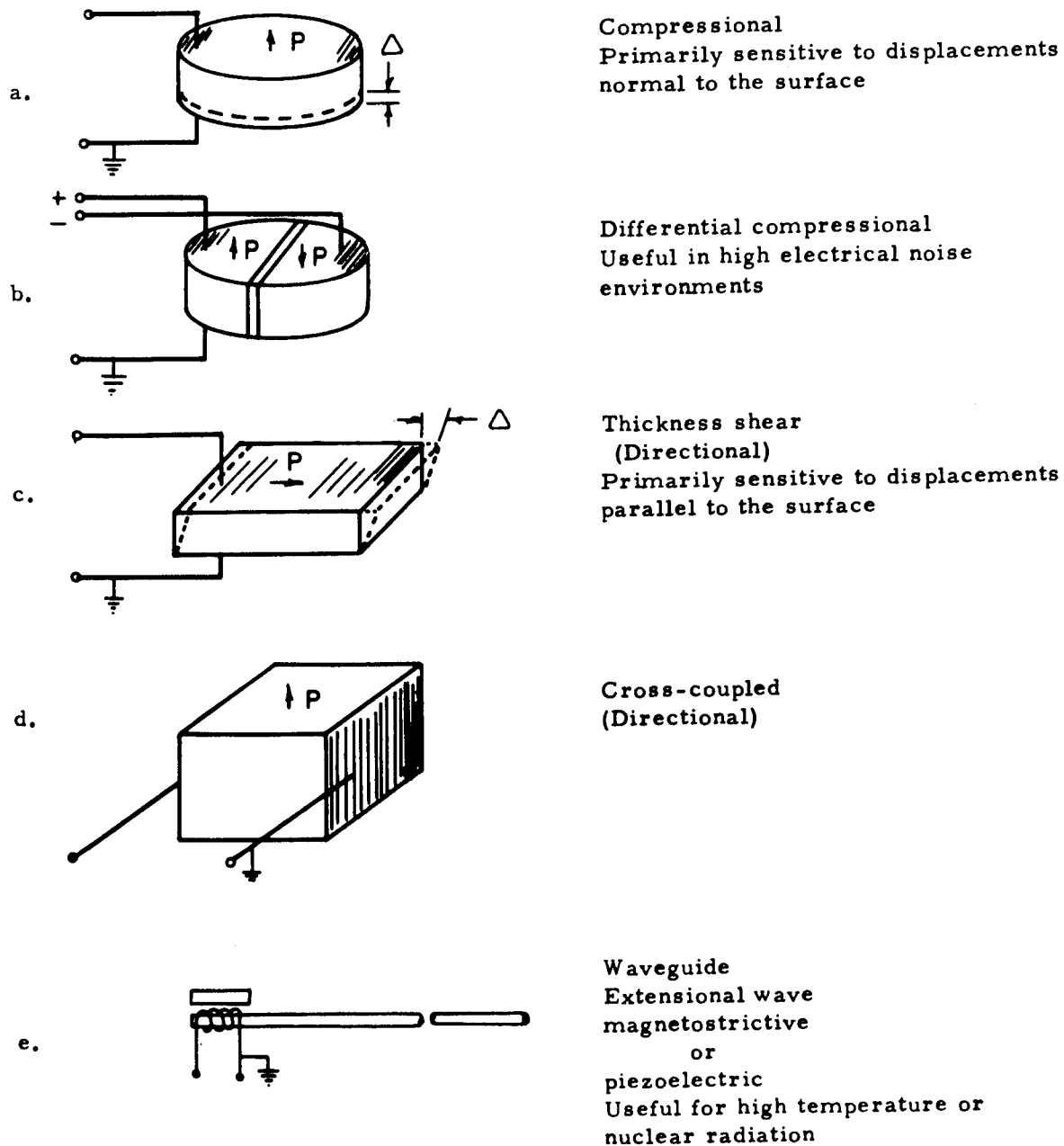
Figure 76. Types of Transducers in Acoustic Emission (Ref. 14)
