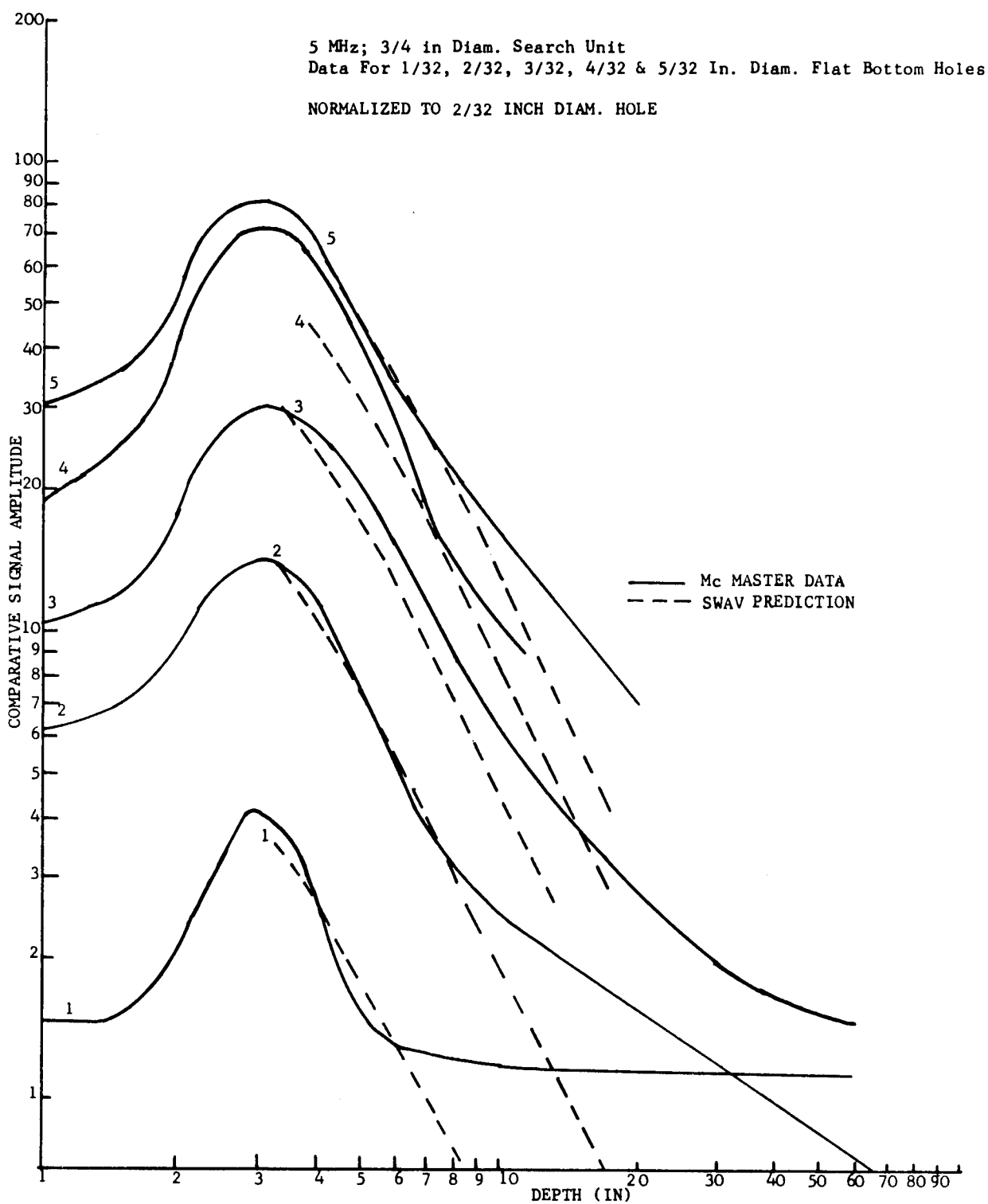
Figure 32. Comparative Amplitude/Distance Data on Flat Holes in Aluminum - Contact Test
