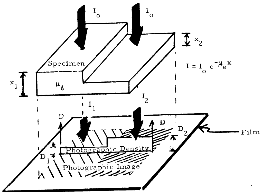
Figure 16. Production of X-Radiographic Image
