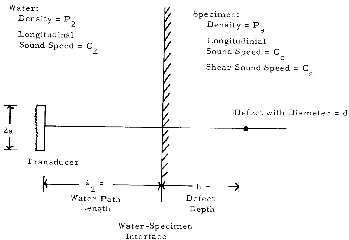
Figure 30. Test Configuration Used As Basis For The Mathematical Model
