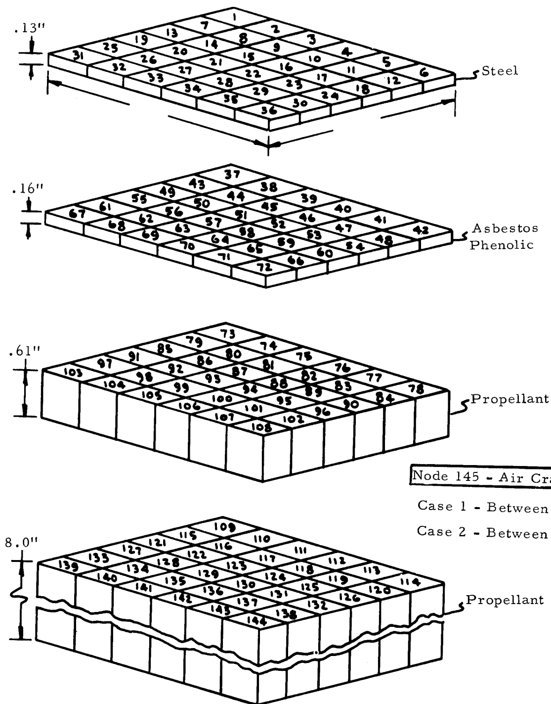
Figure 56. Nodal Spacing for Finite Computer Analysis Model
