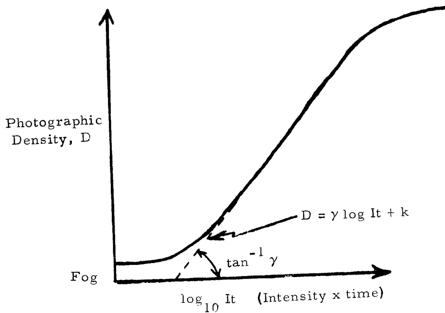
Figure 15. Conventional Characteristic Curve for Film
