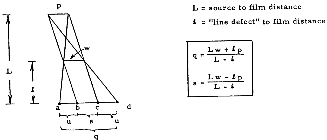
Figure 8. Geometric Unsharpness
