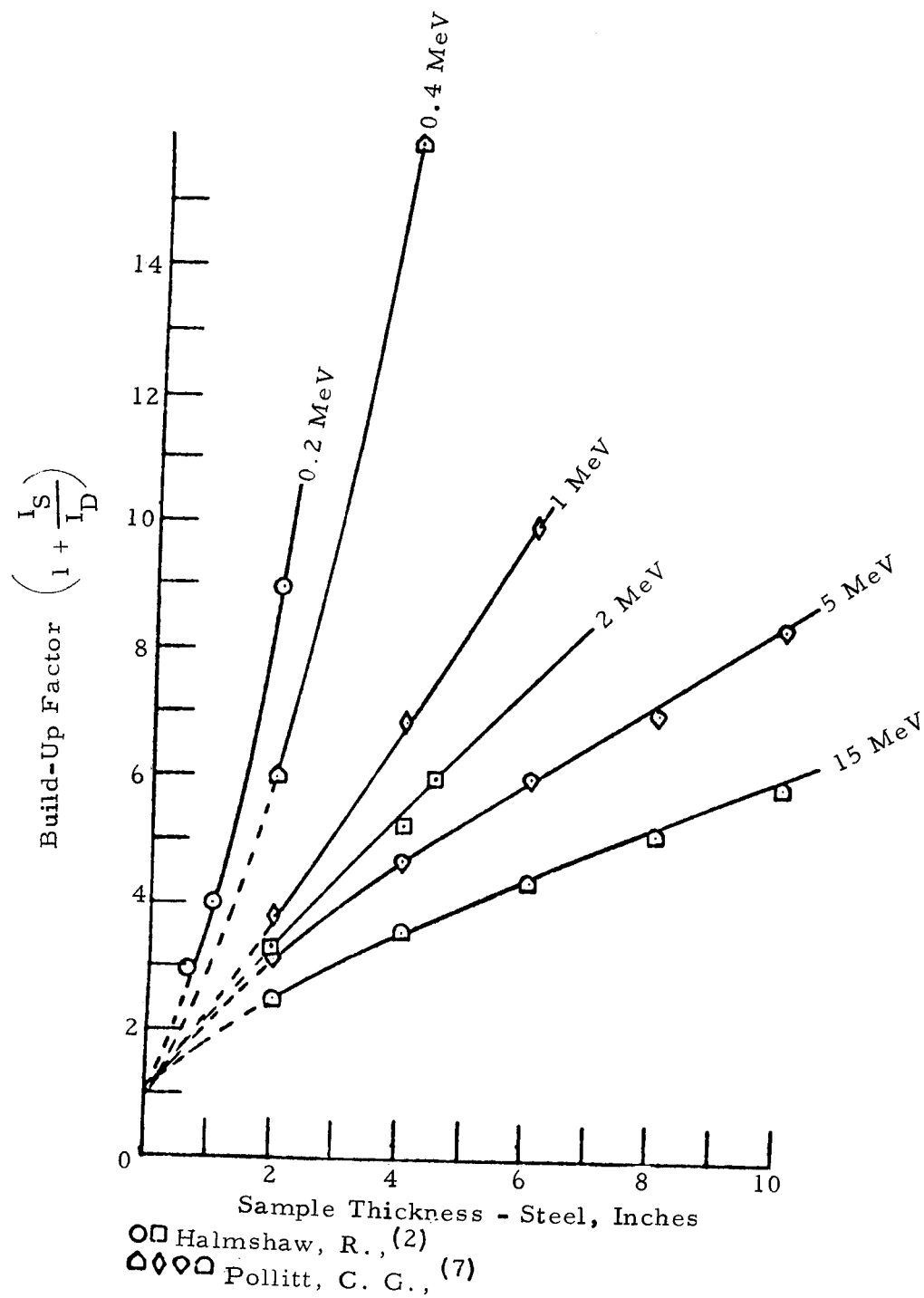
Figure 17. Build/Up Factor vs Sample Thickness (Steel)
