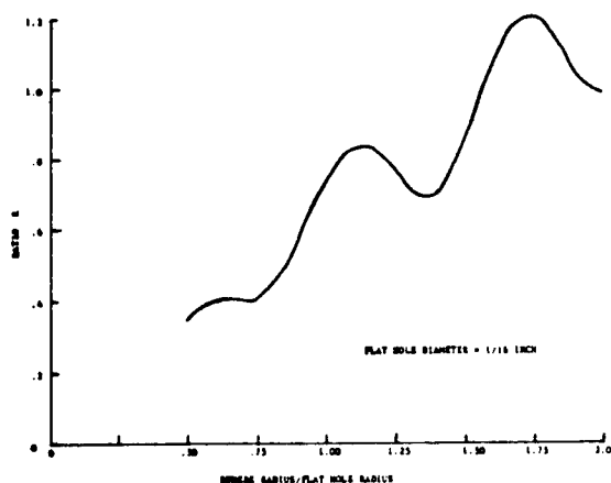
b) Sphere Size Varying with Constant Flat Hole Size.
