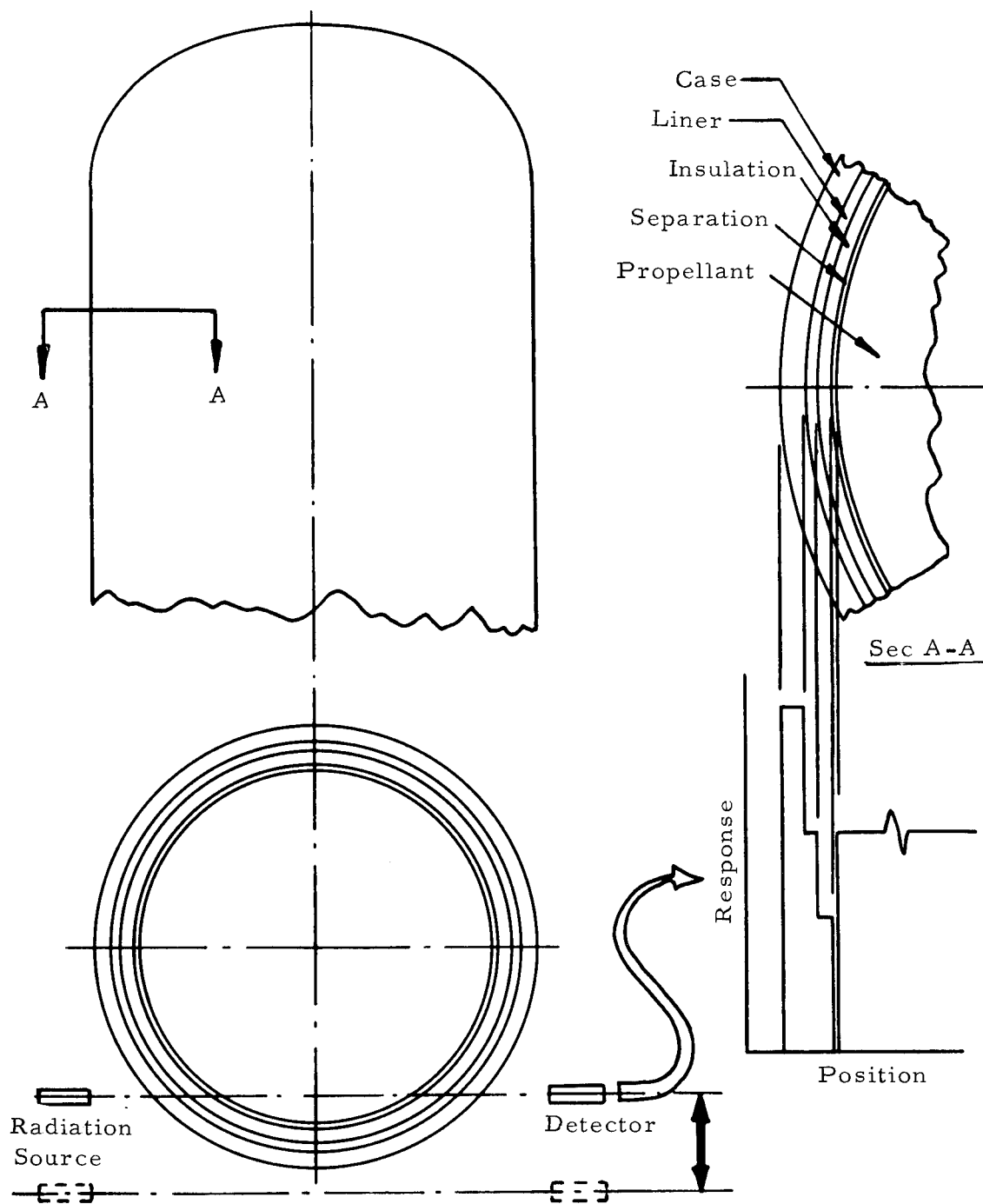
Figure 47. The Fundamentals of FABIS
