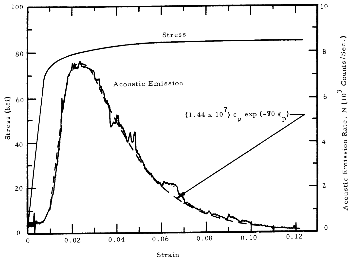
Figure 71. Acoustic Emission and Stress vs Strain for a 7075-T6 Aluminum Tensile Specimen (Ref. 9)
