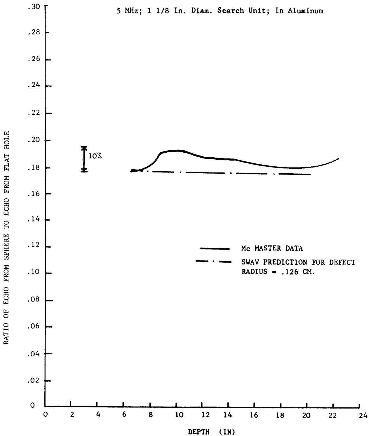
Figure 34. Echo Ratio vs. Distance - Contact Test
