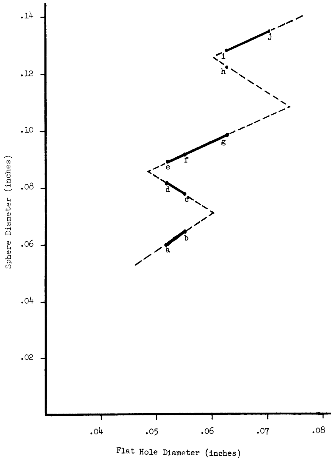
Figure 42. Comparison of Defect Sizes Required to Make Echo Ratio R=1
