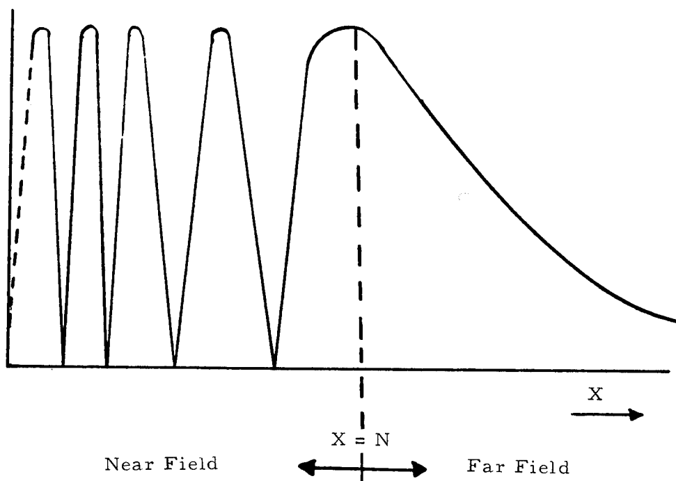
Figure 26. Axial Variations In Sound Intensity
