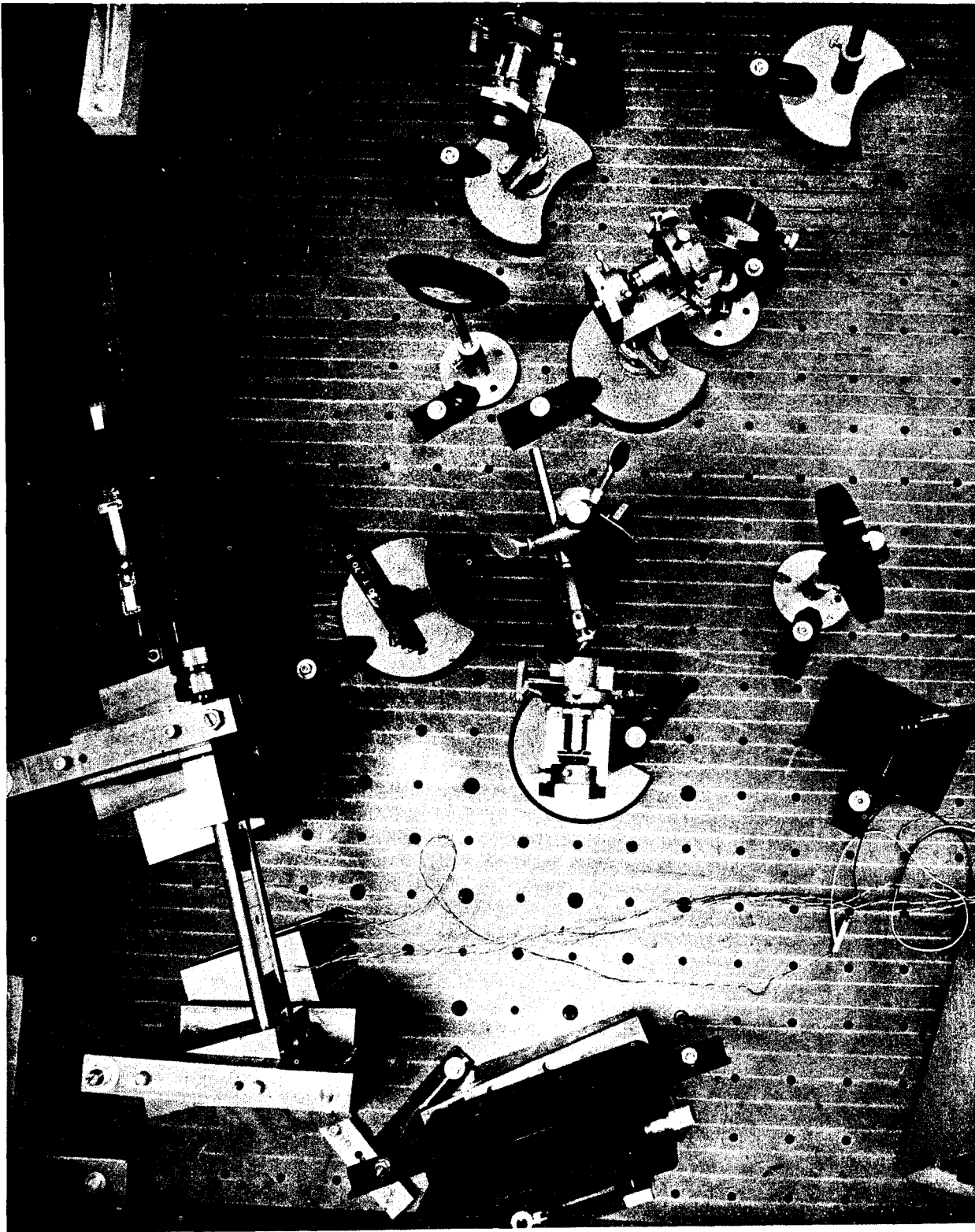
Figure 68. Typical Fixture for Holograph Inspection
