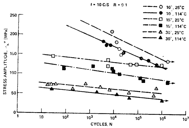
Fig. 7 - S-N curves of various off-axis unidirectional laminae at different temperatures.
