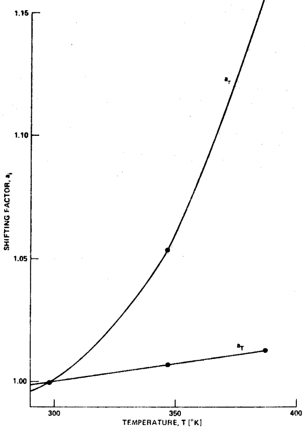
Fig. 10 - Shifting factors for inplane shear, a_{\tau} , and transverse tension, a_T .
