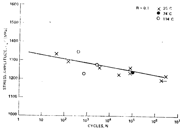
Fig. 6 - S-N curve of unidirectional lamina loaded in the fiber direction.
