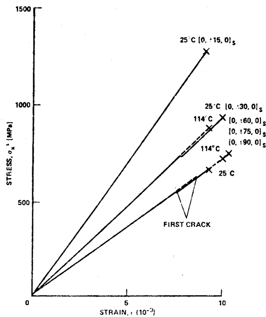
Fig. 5 - Stress-strain curves of various symmetrically balanced graphite/epoxy (T300/5208) laminates at different temperatures.
