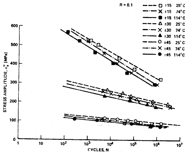
Fig. 8 - S-N curves of some angle-ply laminates at different temperatures.
