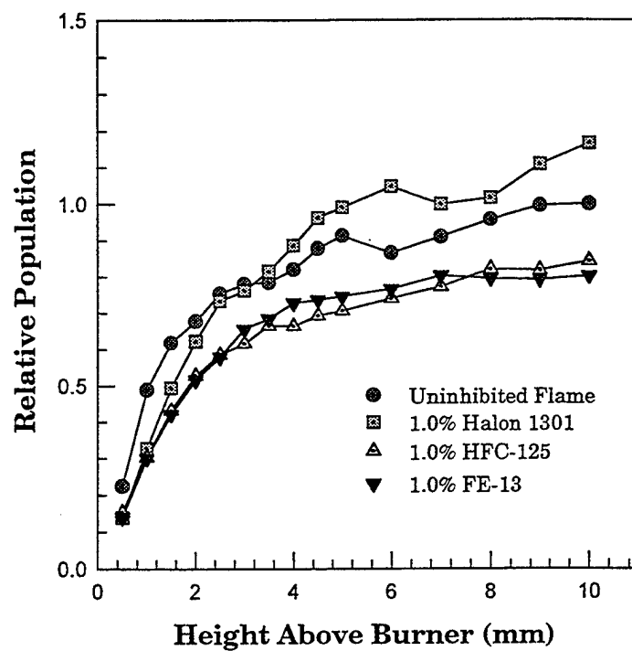
Figure 7. Appearance profiles of water in 32-torr inhibited flames relative to an uninhibited flame.
