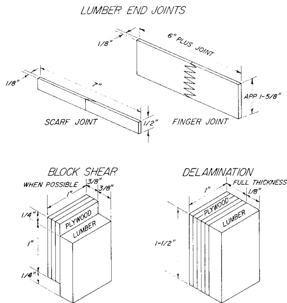
Figure 73. Suitable test specimens for lumber and lumber-plywood combinations for shear, tension, and delamination.
