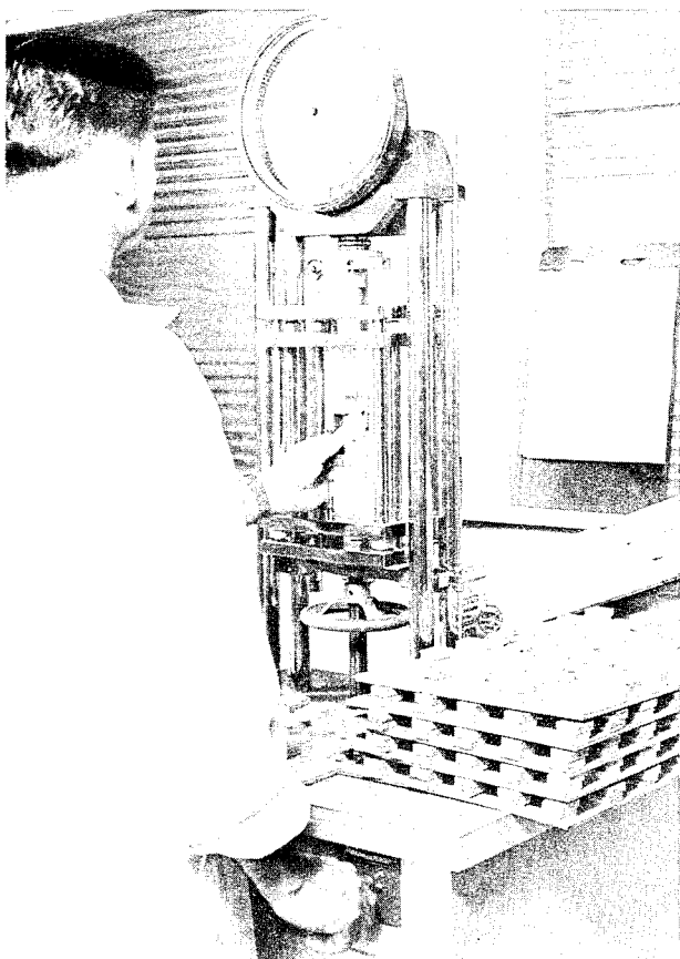
Figure 72.—Testing specimens for shear strength.
