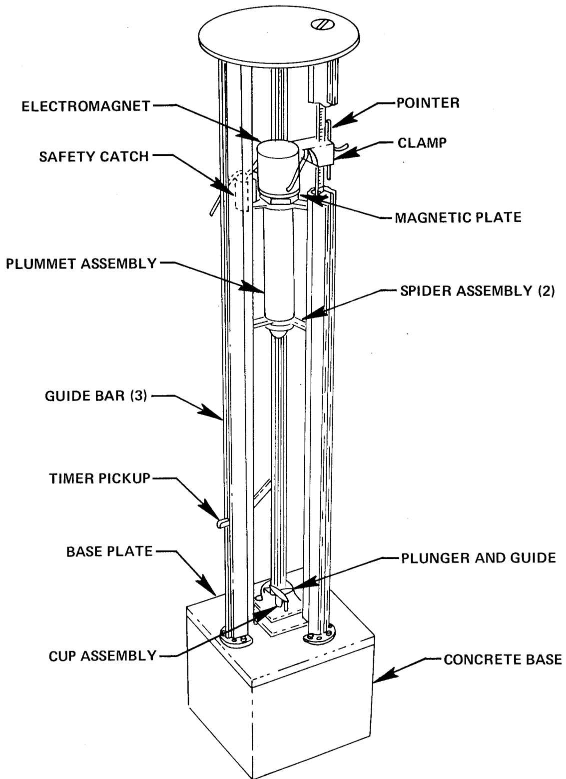
Figure 1. LOX Impact Sensitivity Tester
