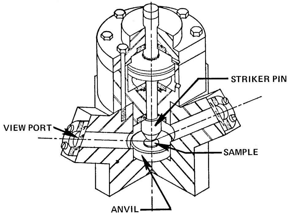
Figure 2. Striker, Cup, and Sample Arrangement of LOX Impact Sensitivity Tester
