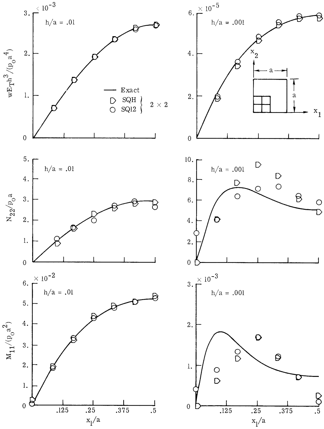
Figure 20.- Distribution of transverse displacement and stress resultants along center lines. Simply supported, nine-layered, orthotropic spherical segments. \frac{h}{a} = 0.01 and 0.001 .
