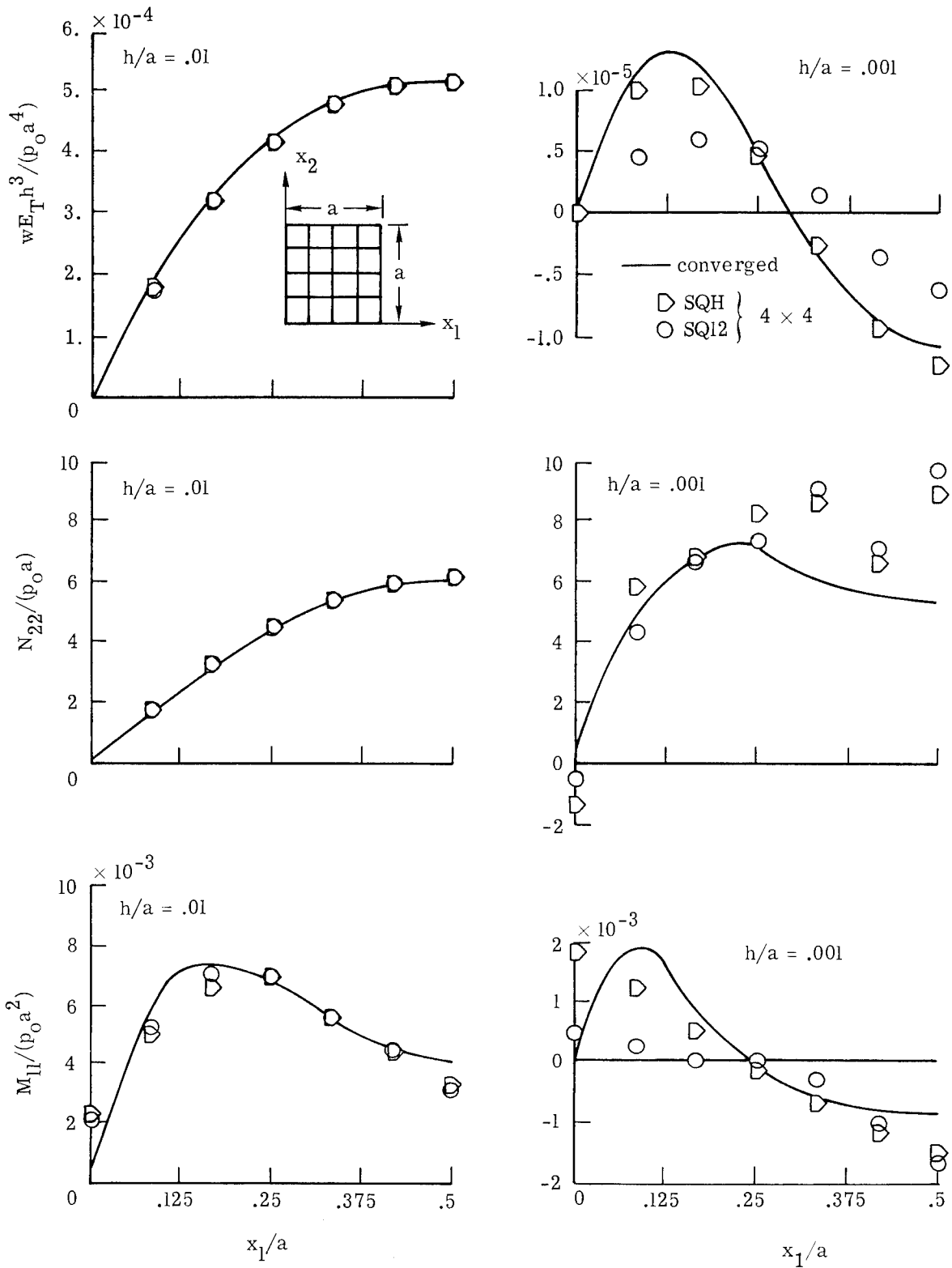
Figure 23.- Distribution of transverse displacement w and stress resultants N_{22} and M_{11} along x_2 = \frac{a}{2} . Simply supported, nine-layered, anisotropic spherical segments. \frac{h}{a} = 0.01 and 0.001 .
