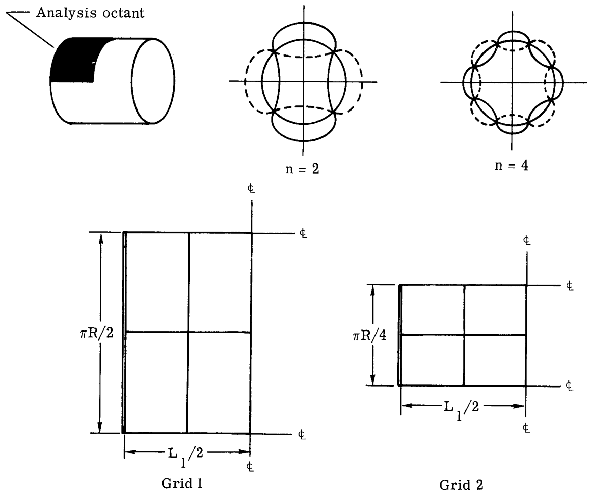
Figure 29.- Grids and modes for orthotropic cylinder.
