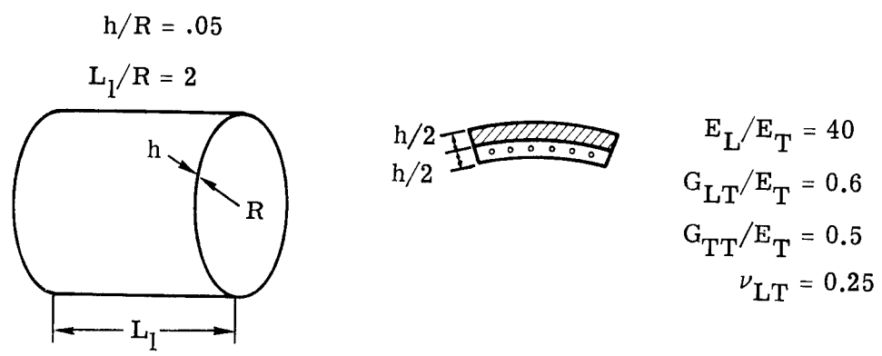
Figure 28.- Characteristics of two-layered graphite-epoxy cylinders.
