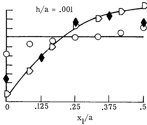
Figure 11.- Distribution of transverse displacement w and bending-moment resultant M_{11} along x_2 = \frac{a}{2} . Clamped, nine-layered, orthotropic square plate. \frac{h}{a} = 0.01 and 0.001.
