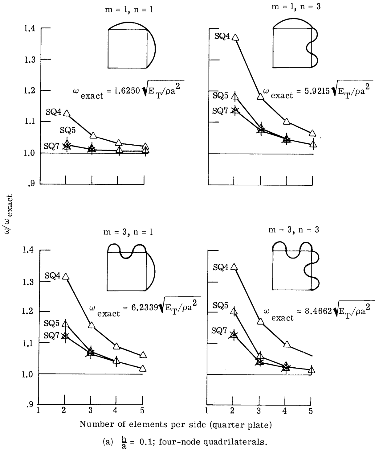
Figure 8.- Effect of internal degrees of freedom on accuracy and convergence of vibration frequencies. Simply supported, nine-layered, orthotropic square plate.
