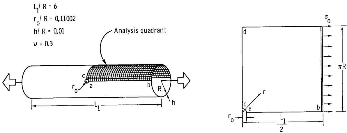
Figure 24.- Cylinder with a circular cutout loaded in tension.
