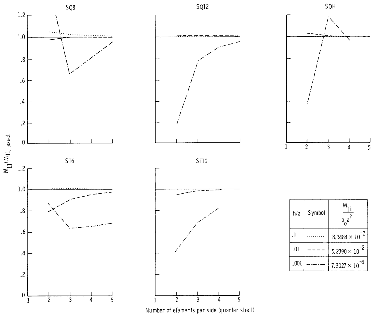
(c) Bending-moment resultant M_{11} at center.
