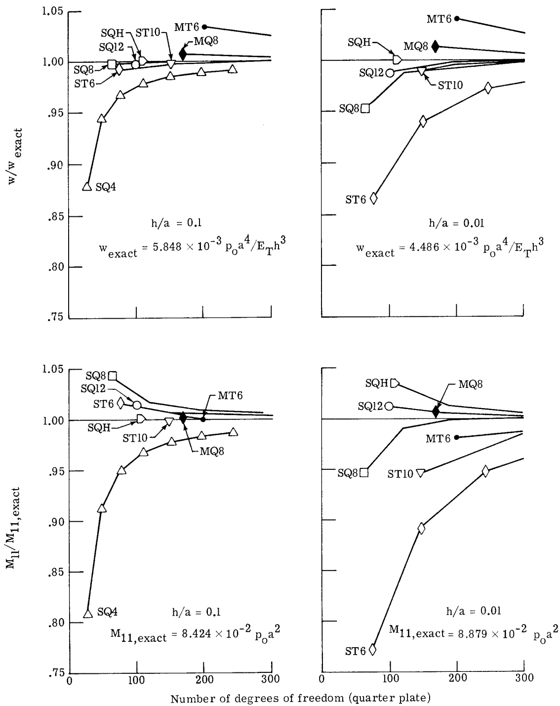
Figure 5.- Convergence of w and M_{11} obtained by different stiffness and mixed models with increasing number of degrees of freedom. Simply supported, nine-layered, orthotropic square plate with \frac{h}{a} = 0.1 and 0.01 .
