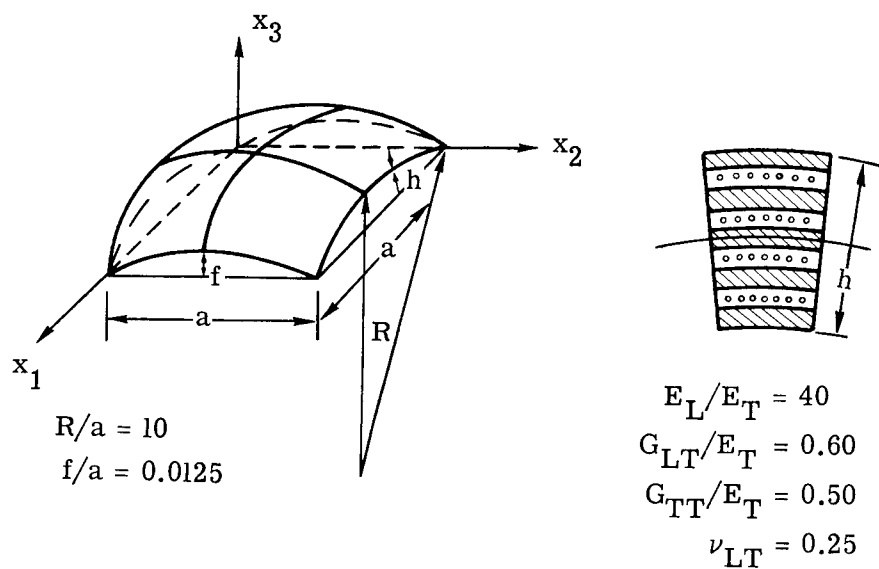
Figure 17.- Characteristics of laminated graphite-epoxy shallow shells used in present study.
