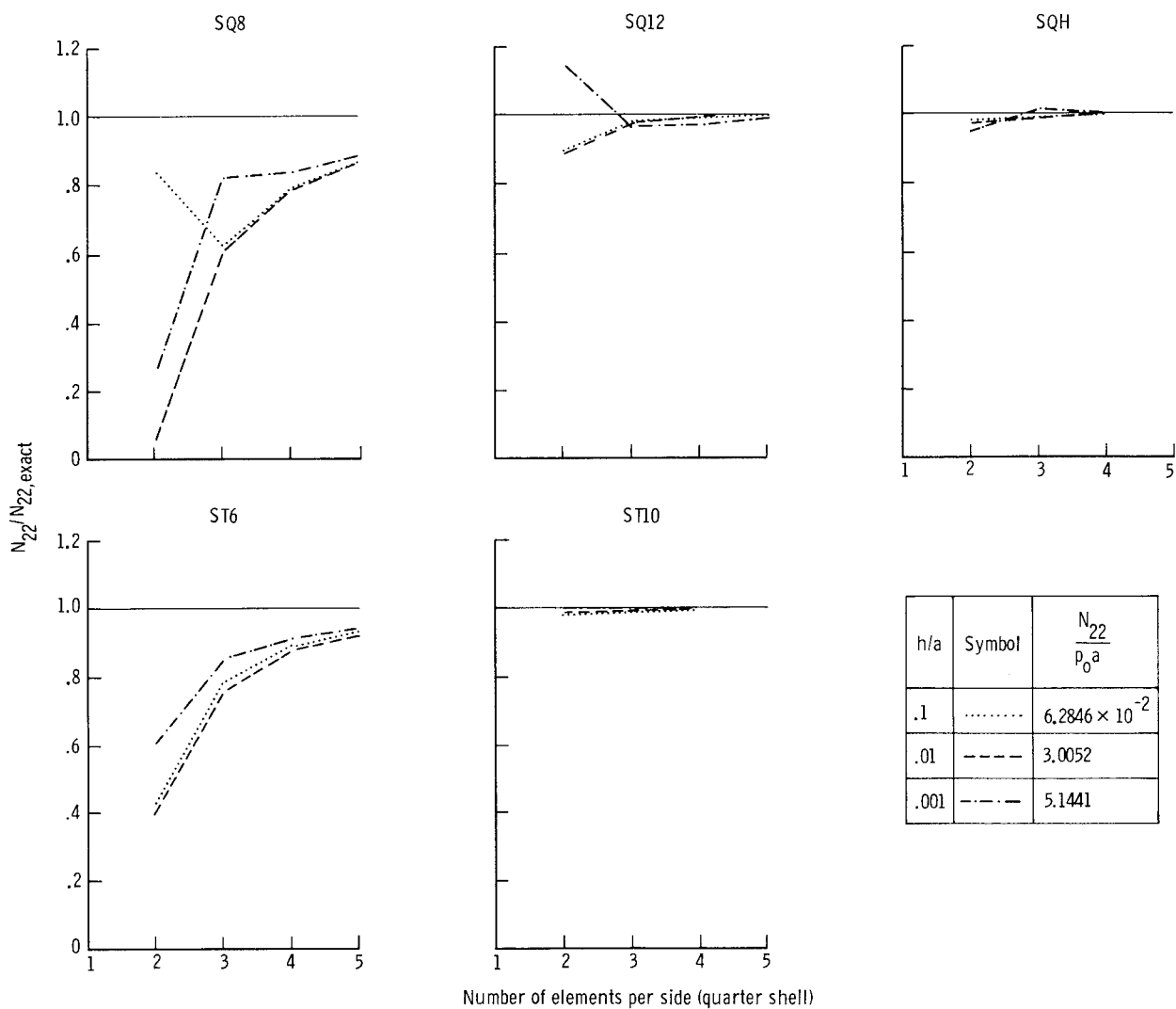
(b) Membrane stress resultant N_{22} at center.
