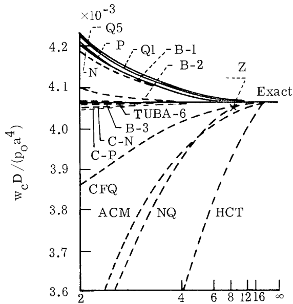
(a) w at center for previously developed classical-theory elements (ref. 11).
