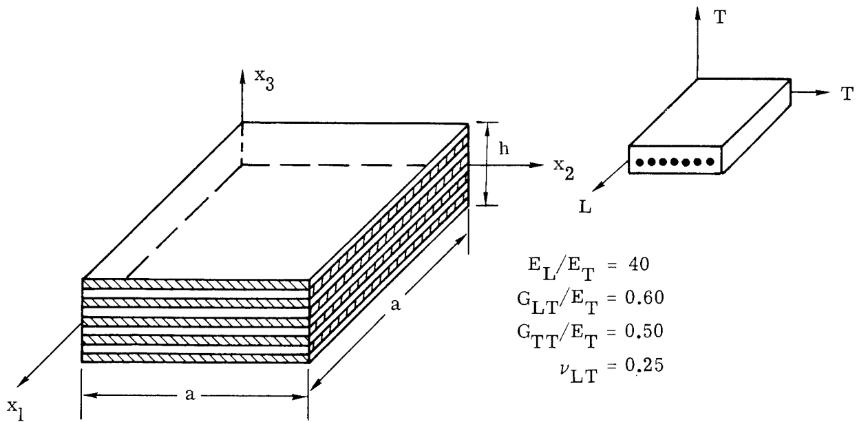
Figure 3.- Characteristics of laminated graphite-epoxy plates used in present study.
