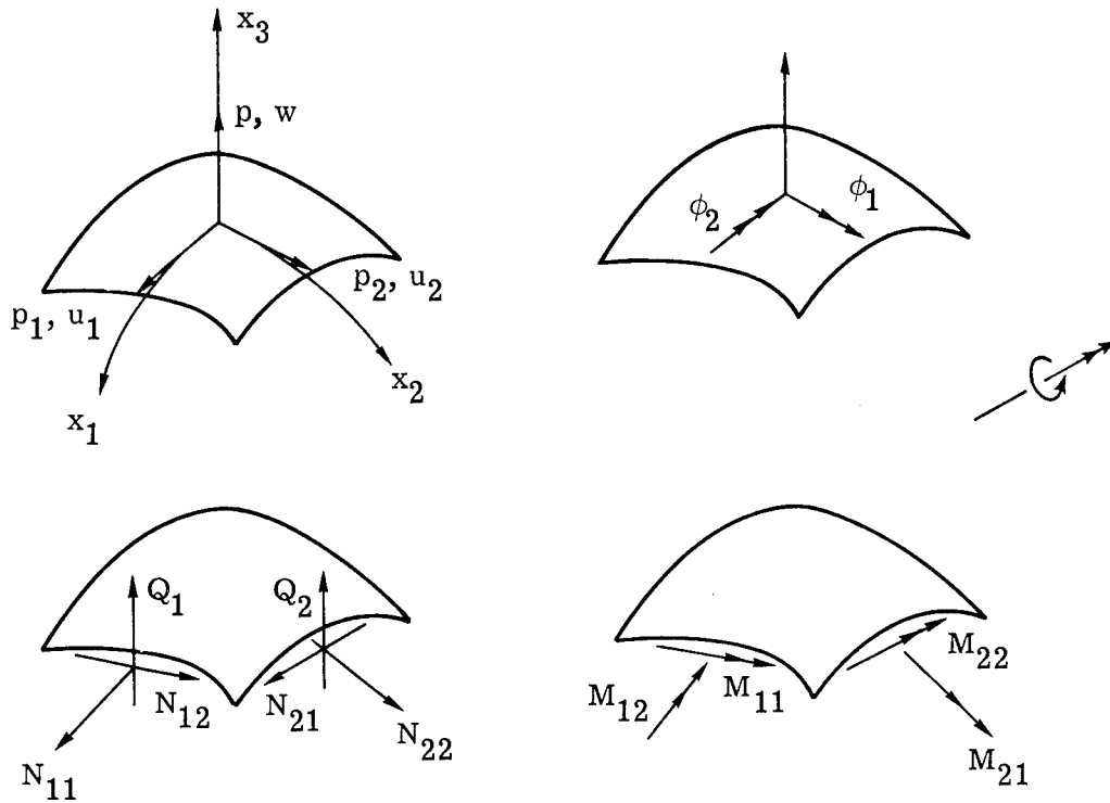
Figure 1.- Shell element and sign convention.
