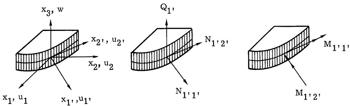
Figure 2.- Stress resultants and displacements at a curved boundary.
