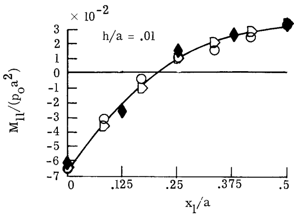
Figure 11.- Distribution of transverse displacement w and bending-moment resultant M_{11} along x_2 = \frac{a}{2} . Clamped, nine-layered, orthotropic square plate. \frac{h}{a} = 0.01 and 0.001.
