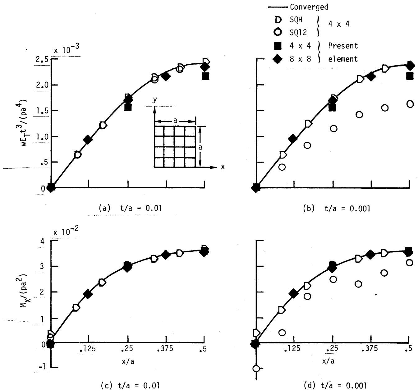
Figure 9.1-3 - Distribution of transverse displacement w and bending-moment resultant M_x along Y = a/2 . Simply supported, nine-layered (45/-45/45/-45/45/-45/45/-45/45), anisotropic square plate (ref. 9.1-15).
