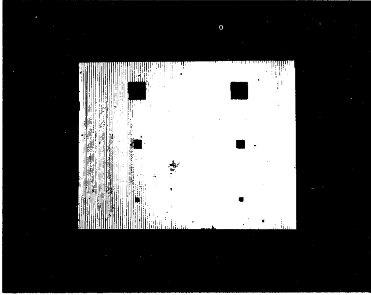
(b) C-scan, gain 30.
