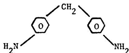
4,4'-Methylenedianiline (MDA)
