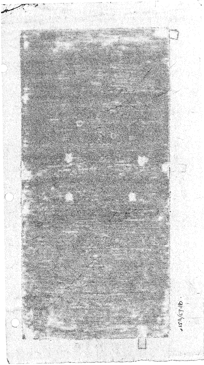
Figure C-9A. Ultrasonic C-scan of panel 15.
