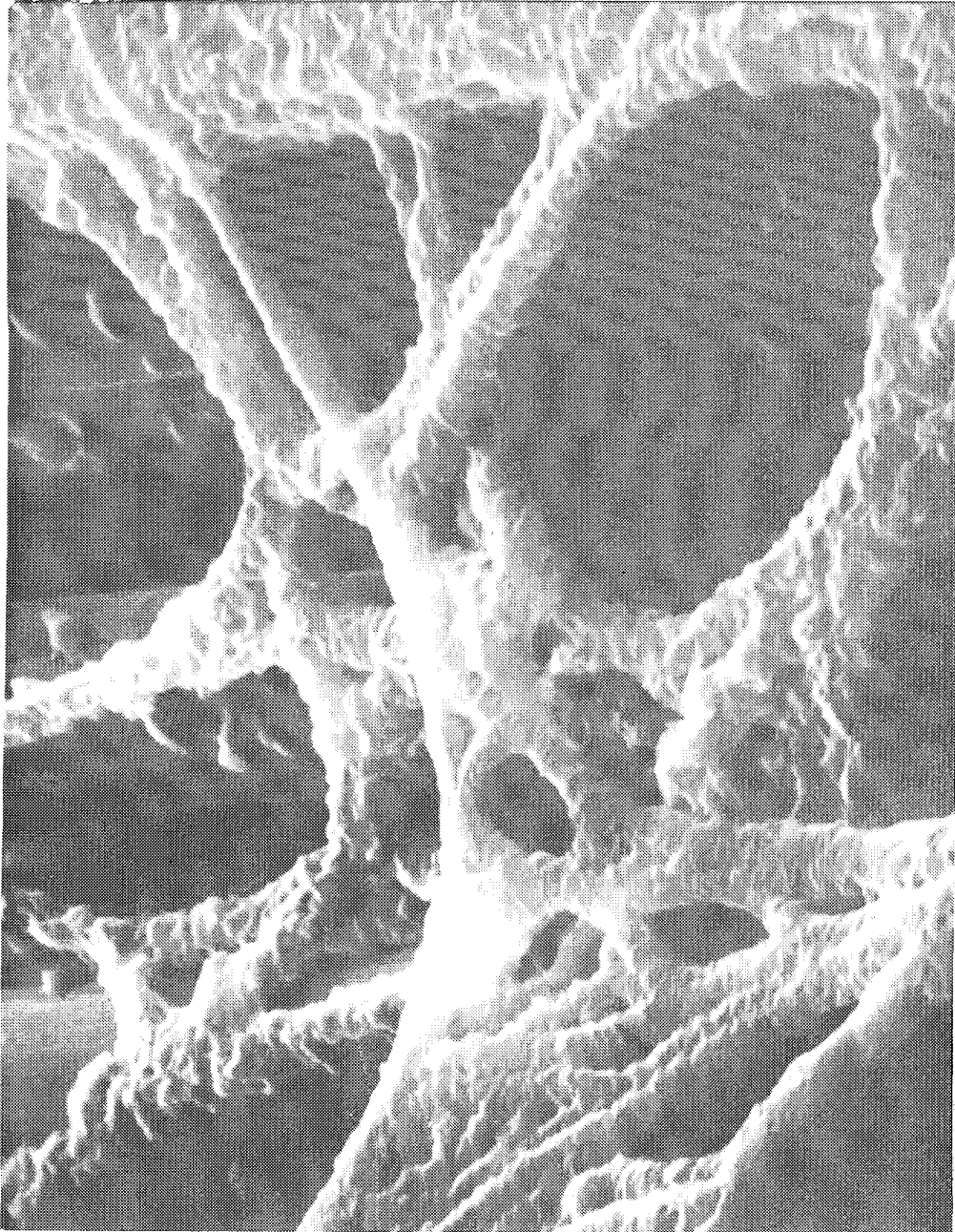
Figure 5-5. SEM of unidirectionally oriented graphite fibers interconnected by In Situ Fiberized polypropylene. Magnification \approx 6000X.
