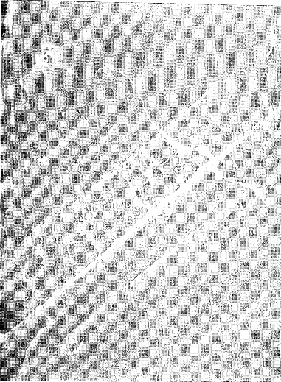
Figure 5-14. SEM of polypropylene In Situ Fibers deposited on graphite cloth from a 1.5 percent solution at 380 K (225°F). Magnification \approx 1500\times .
