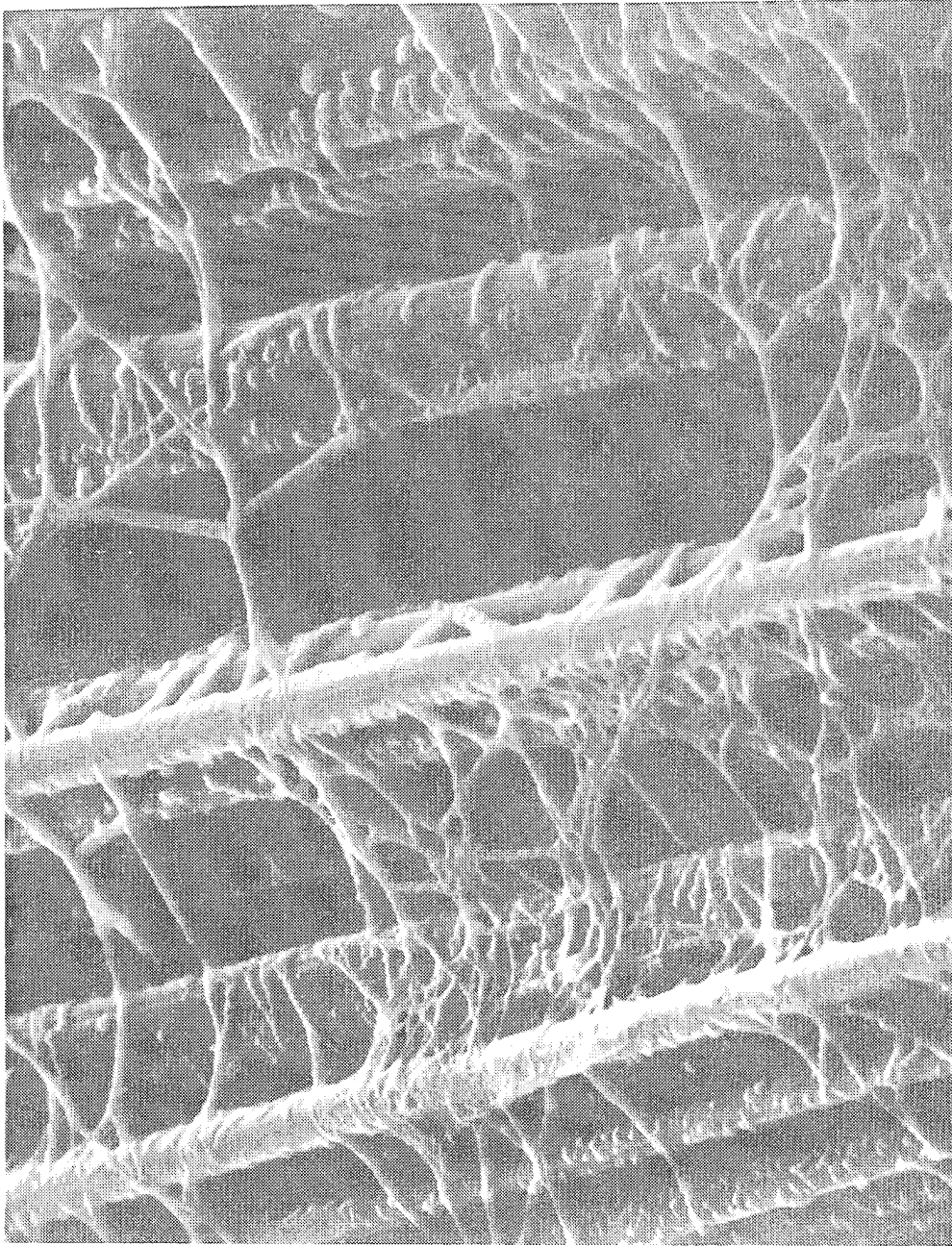
Figur5-1. SEM of unidirectionally oriented graphite fibers interconnected by In Situ Fiberized polypropylene. Magnification \approx 1200X.
