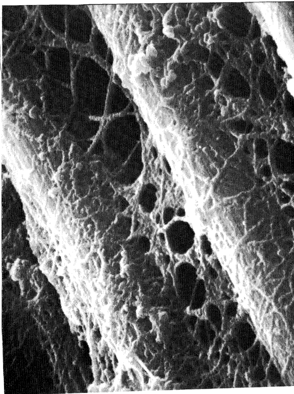
Figure 5-15. SEM of polypropylene In Situ Fibers deposited on graphite cloth from a 1.5 percent solution at 380 K (225°F). Magnification \approx 6000X.
