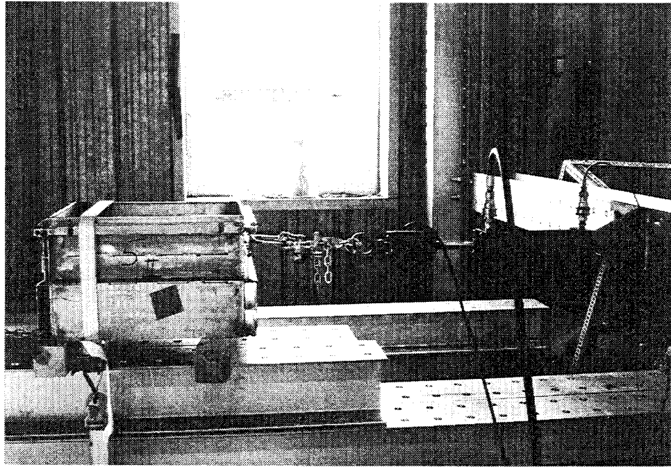
Figure 1. TEST SETUP.
