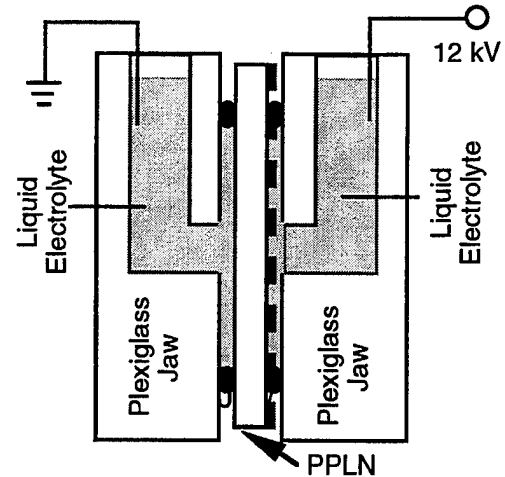
Fig. 3 Poling sample holder. The PPLN is sandwiched between two o-rings held by plexiglas jaws. The jaws hold a liquid electrolyte which contacts the sample surface. The wire leads from the amplifier are dipped into liquid to complete the circuit.
