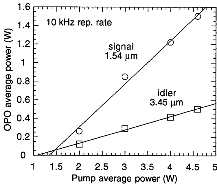
Fig. 7 Input vs. output for PPLN OPO operating at 10 kHz with the attenuator and isolator in the pump beam (limiting the pump power to <5 W).
