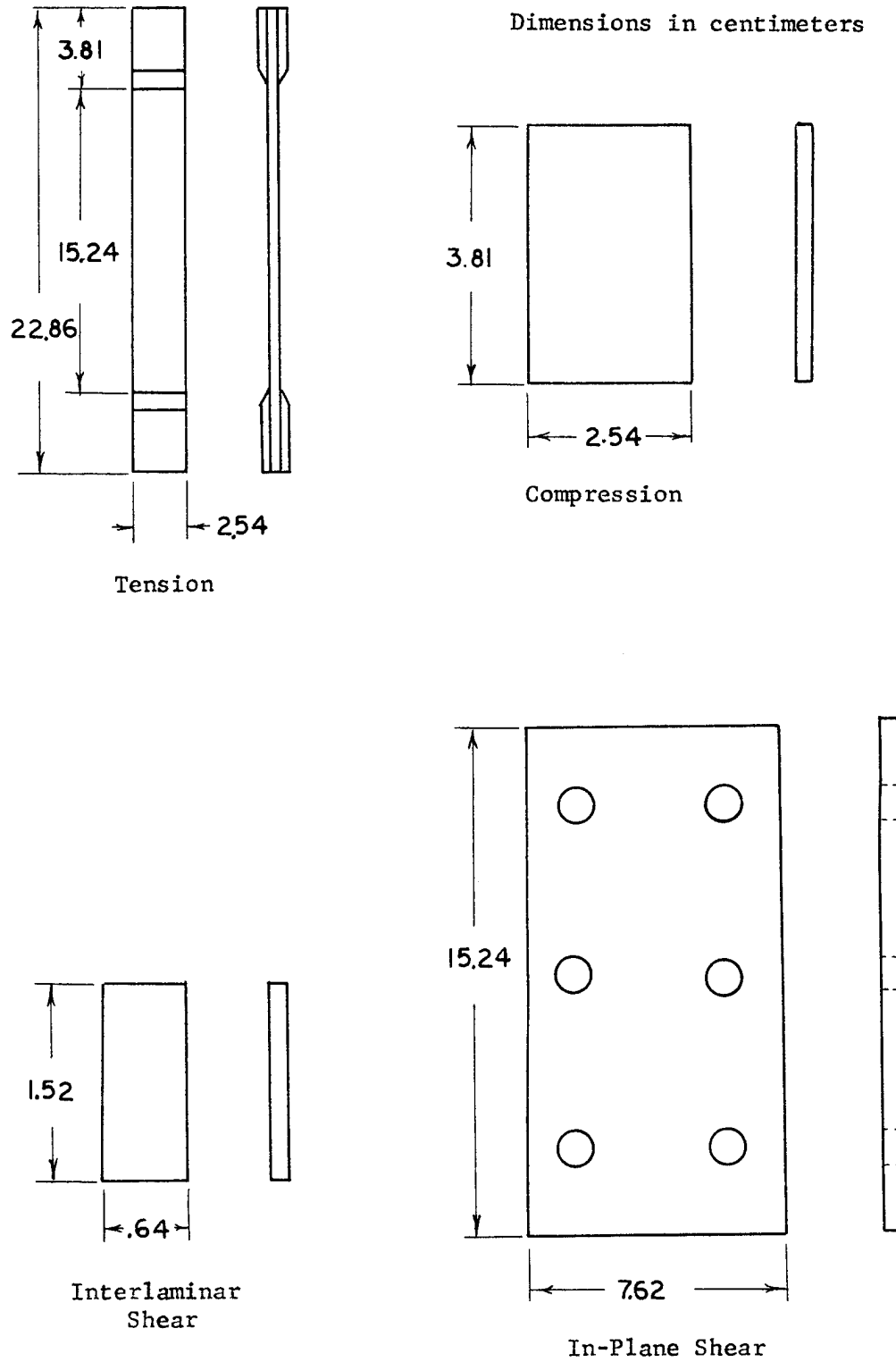
Figure 4-1. Test Specimen Configurations
