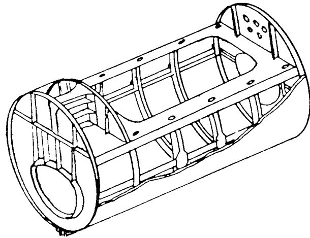
EXISTING METAL DESIGN
