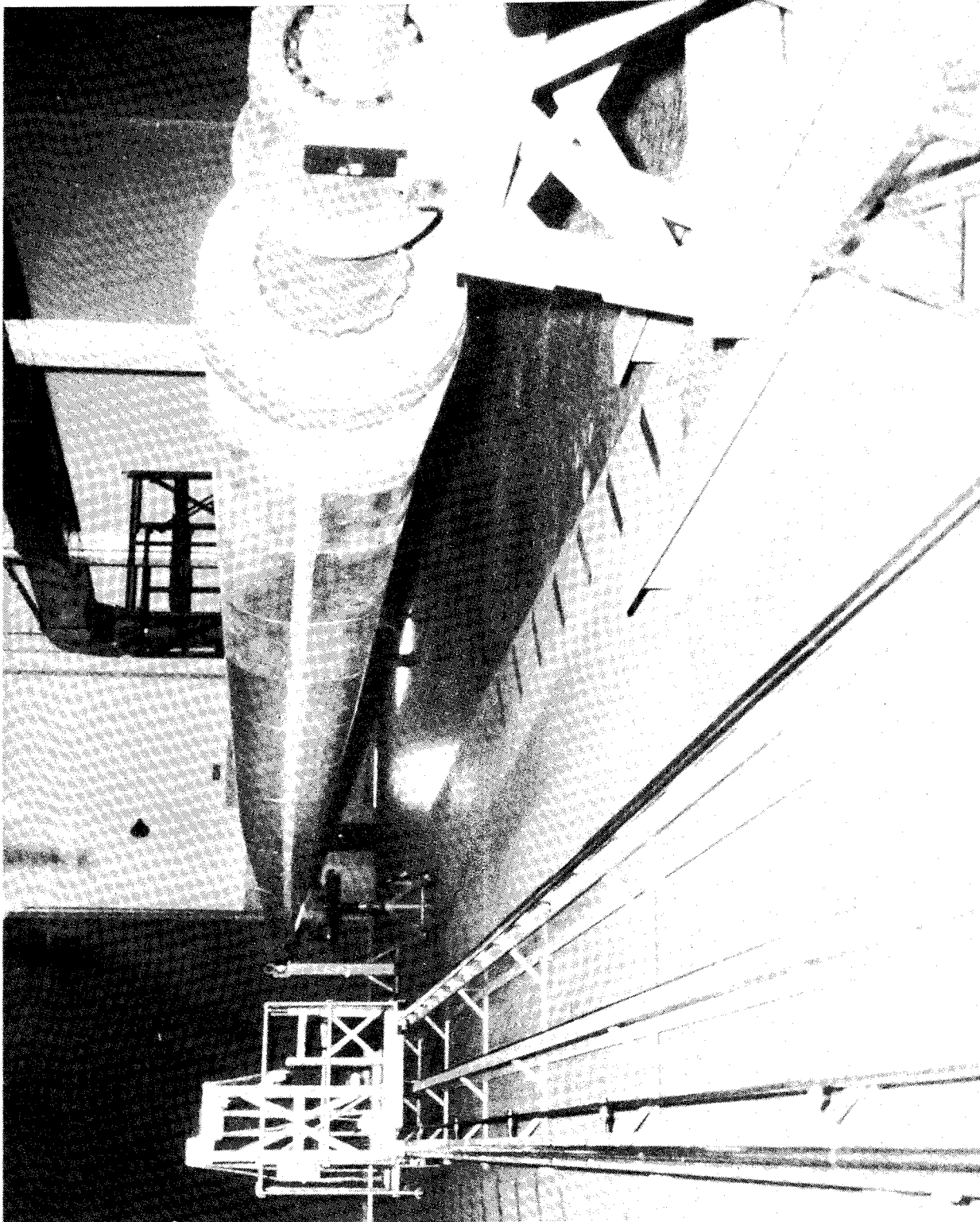
FIGURE 61. FILAMENT WINDING MACHINE
