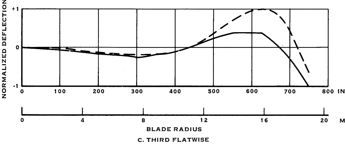
FIGURE 103. FLATWISE MODE SHAPES
