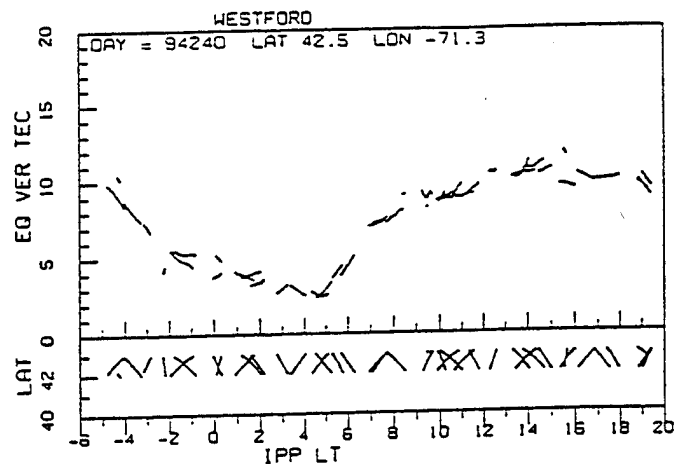
Figure 3. Diurnal TEC plot obtained from algorithm, 1° latitude band, Westford, more than 6 months after Fig. 1.
