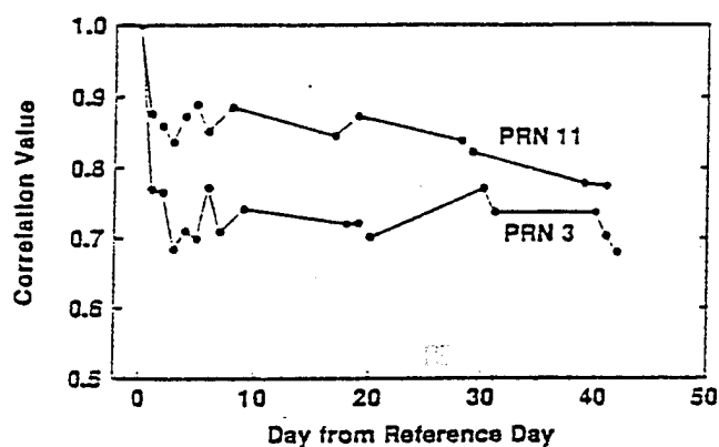
Figure 6. Peak correlation values of multipath template vs template from first day, over a 42-day period at Shemya, Alaska; PRN 11 - high multipath, PRN 3 - low.
