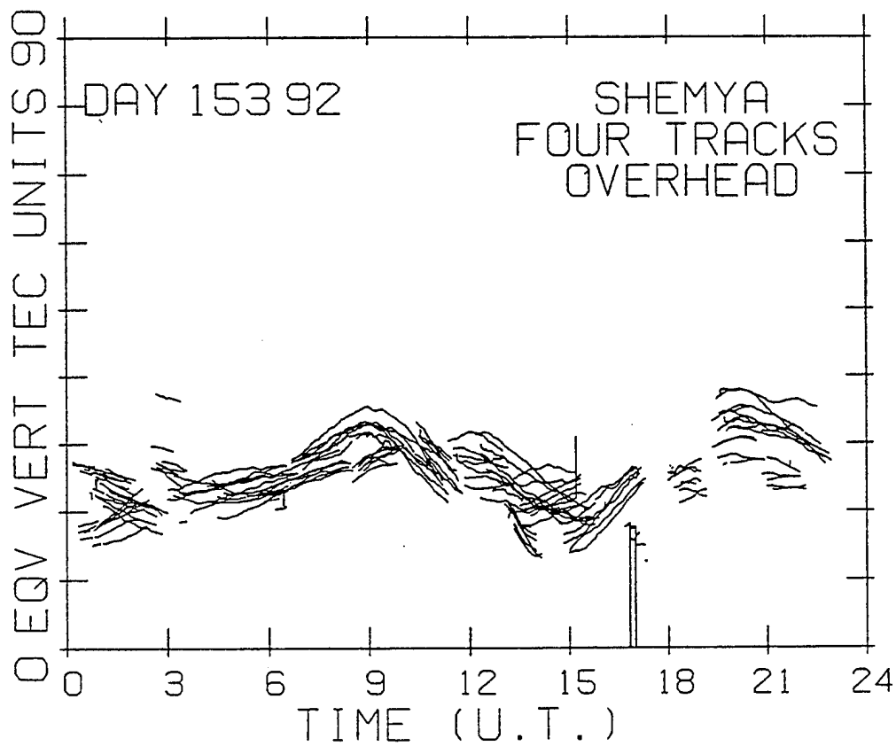
Figure 1. Overplot of Shemya TEC data from days 153 - 159, 1992.
