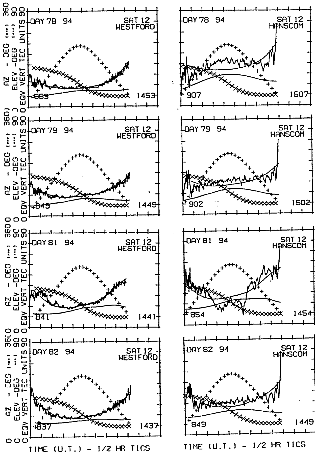
Figure 10. Data from nearby Westford, MA, (IGS) compared to Ashtech Z-12/Micropulse antenna data.
