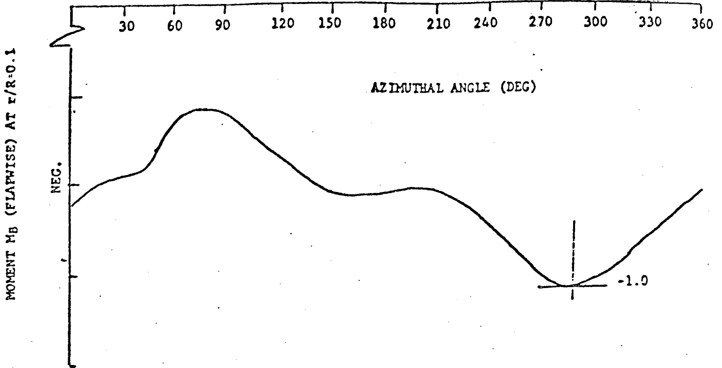
FIGURE -1 FLAPWISE MOMENT AT r/R = 0.1
