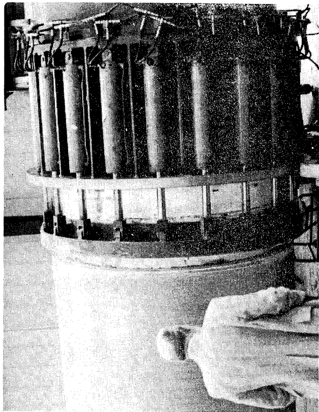
Figure 14. Removal of Spar from Mandrel.
