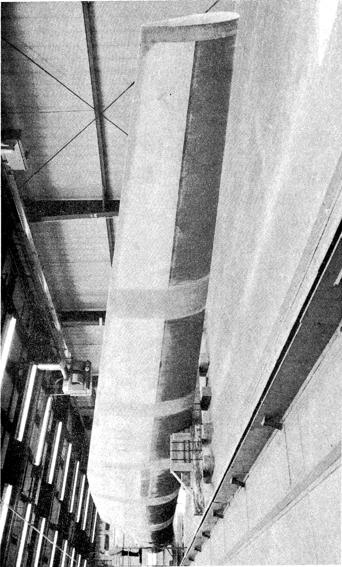
Figure 19. Five Chordwise Overwraps on Unpainted Blade.
