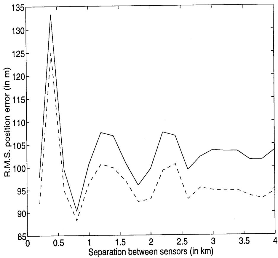
Figure 1.7: RMS position error as a function of the distance between radars (the range resolution is 100 meters and the azimuth resolution is 1 degree).
