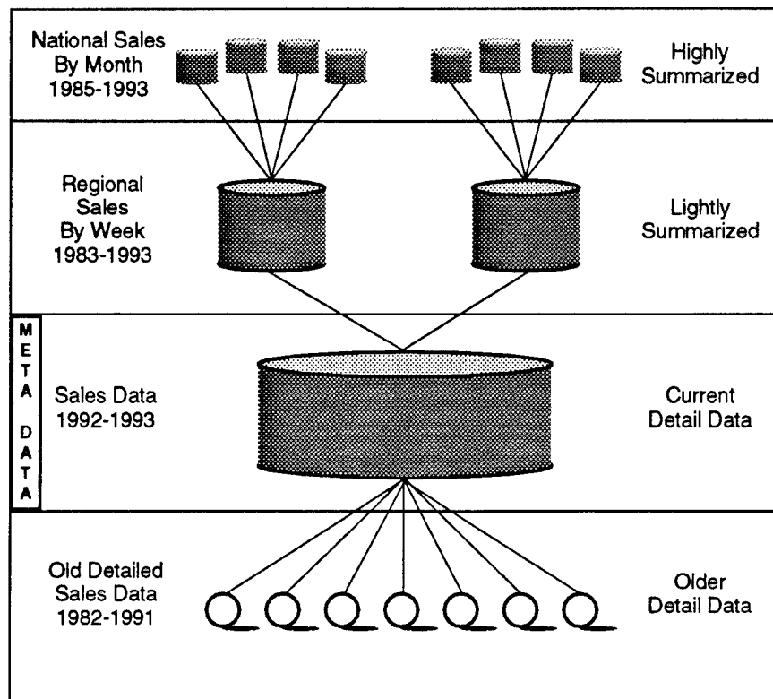
Figure 8-2. Data Warehouse After (Inmon, 1995).
