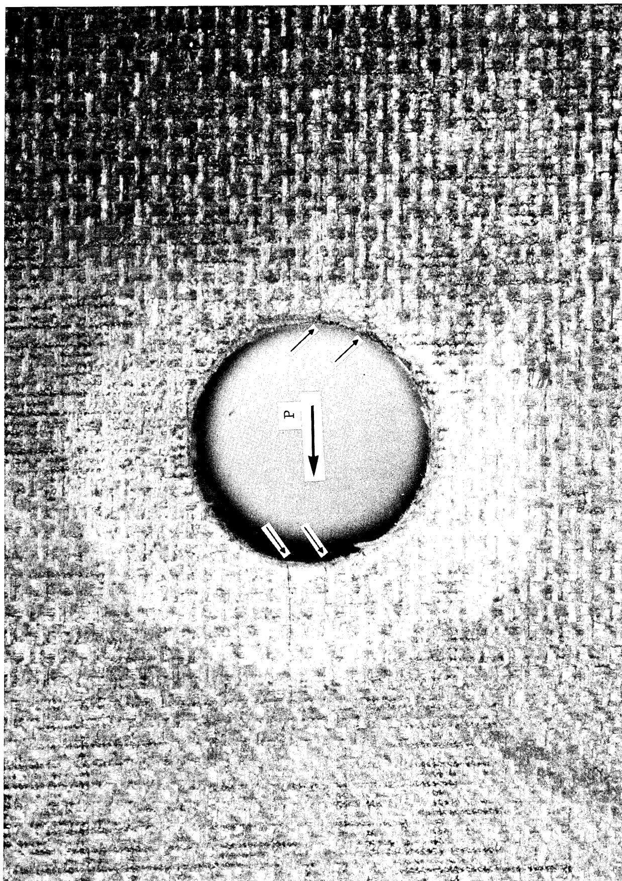
Figure 22 Splitting Failure Mode in Static Compression Specimen
