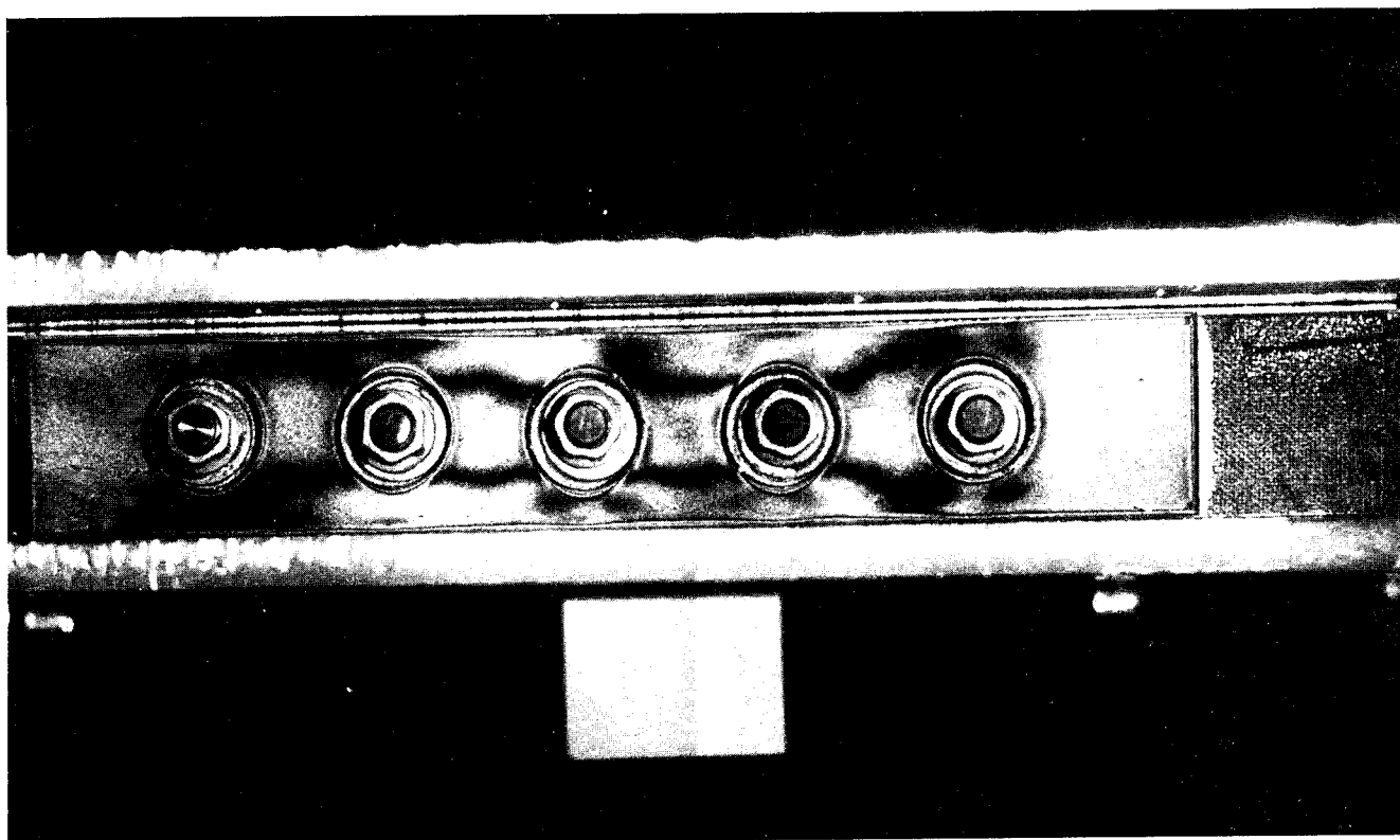
Figure 15 Compression Specimen Under Compression Load
