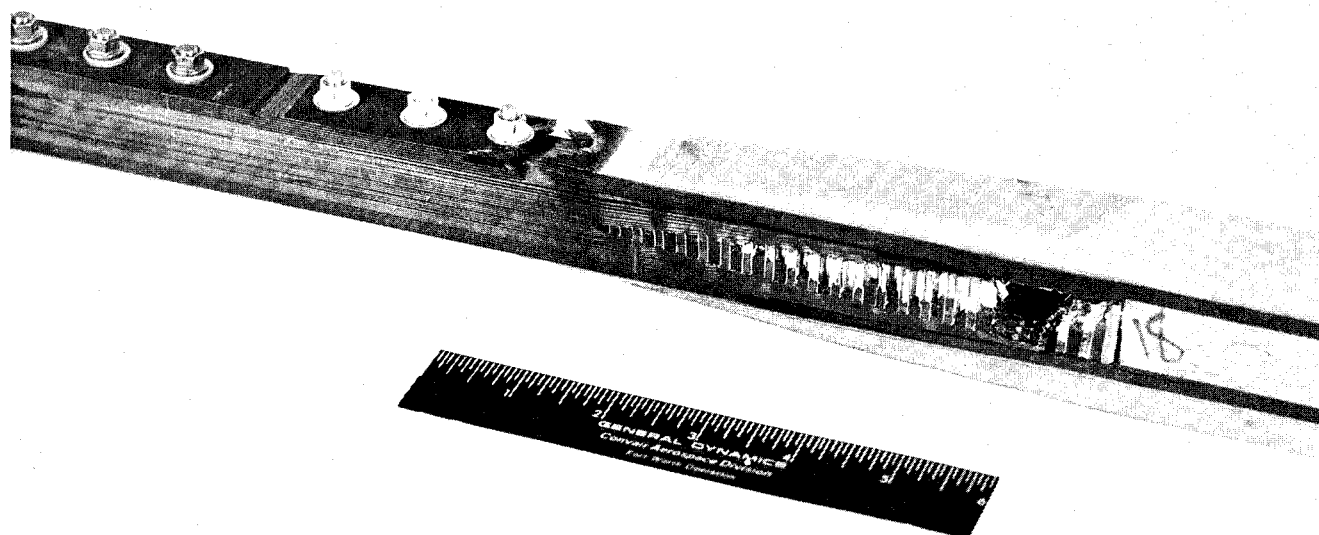
Figure 18 Static Tension Specimen End Grip Failure
