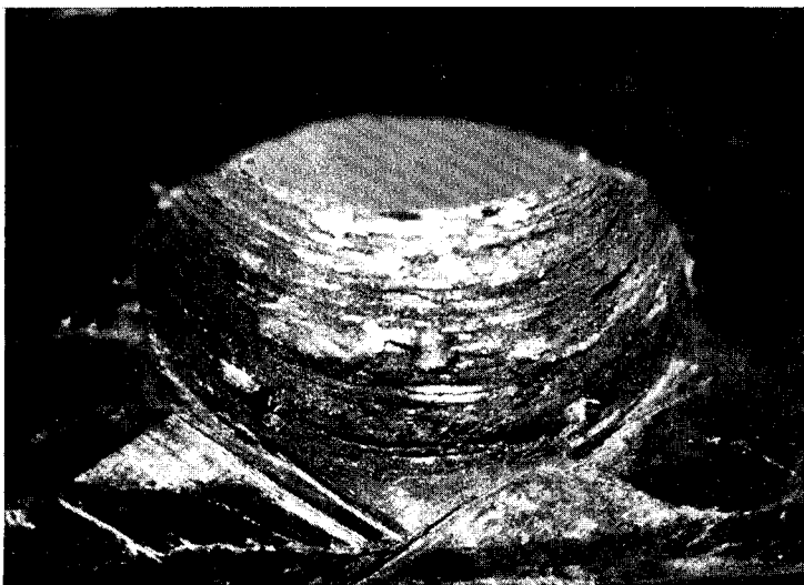
Thin End Hole - View From Inside Scarf
