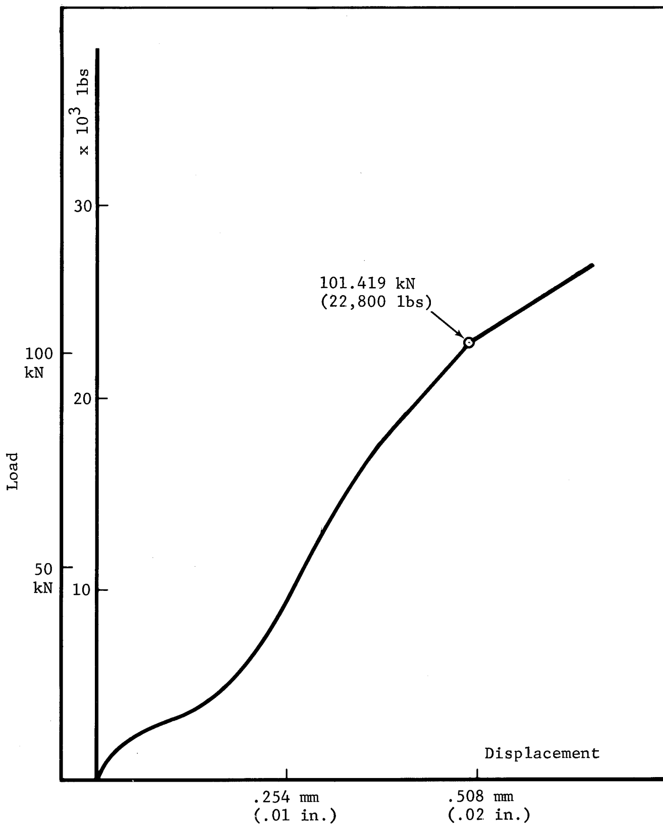
Figure 21 Typical Load-Displacement Curve for Compression Splice Specimen
