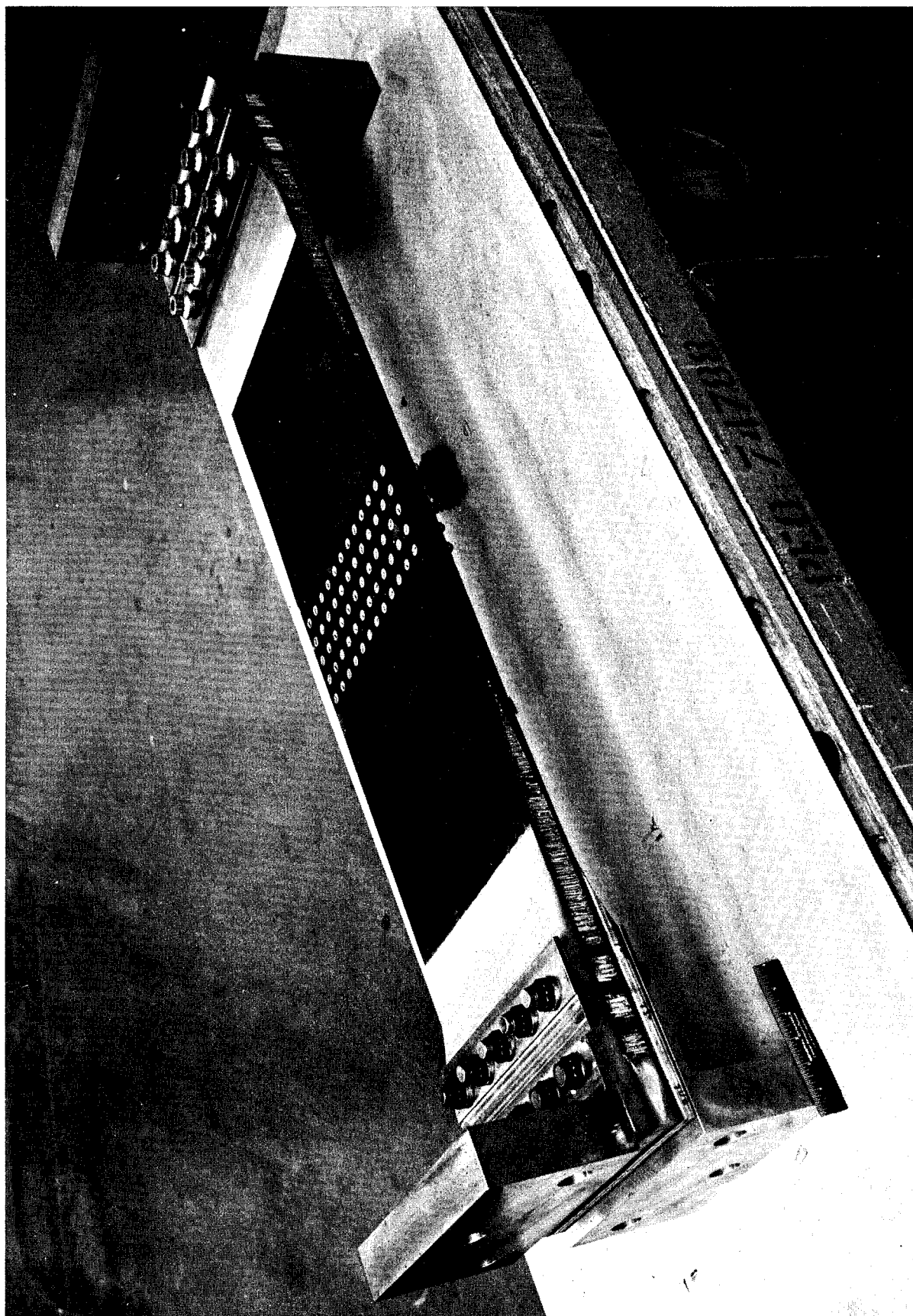
Figure 41 Compression Splice Panel - Outer Surface
