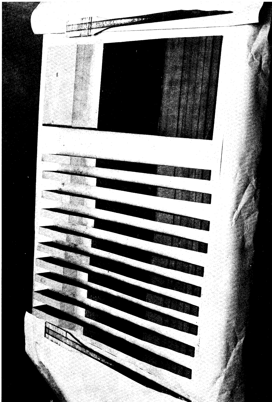
Figure 37 Large Panel and Specimens Cut From Blank
