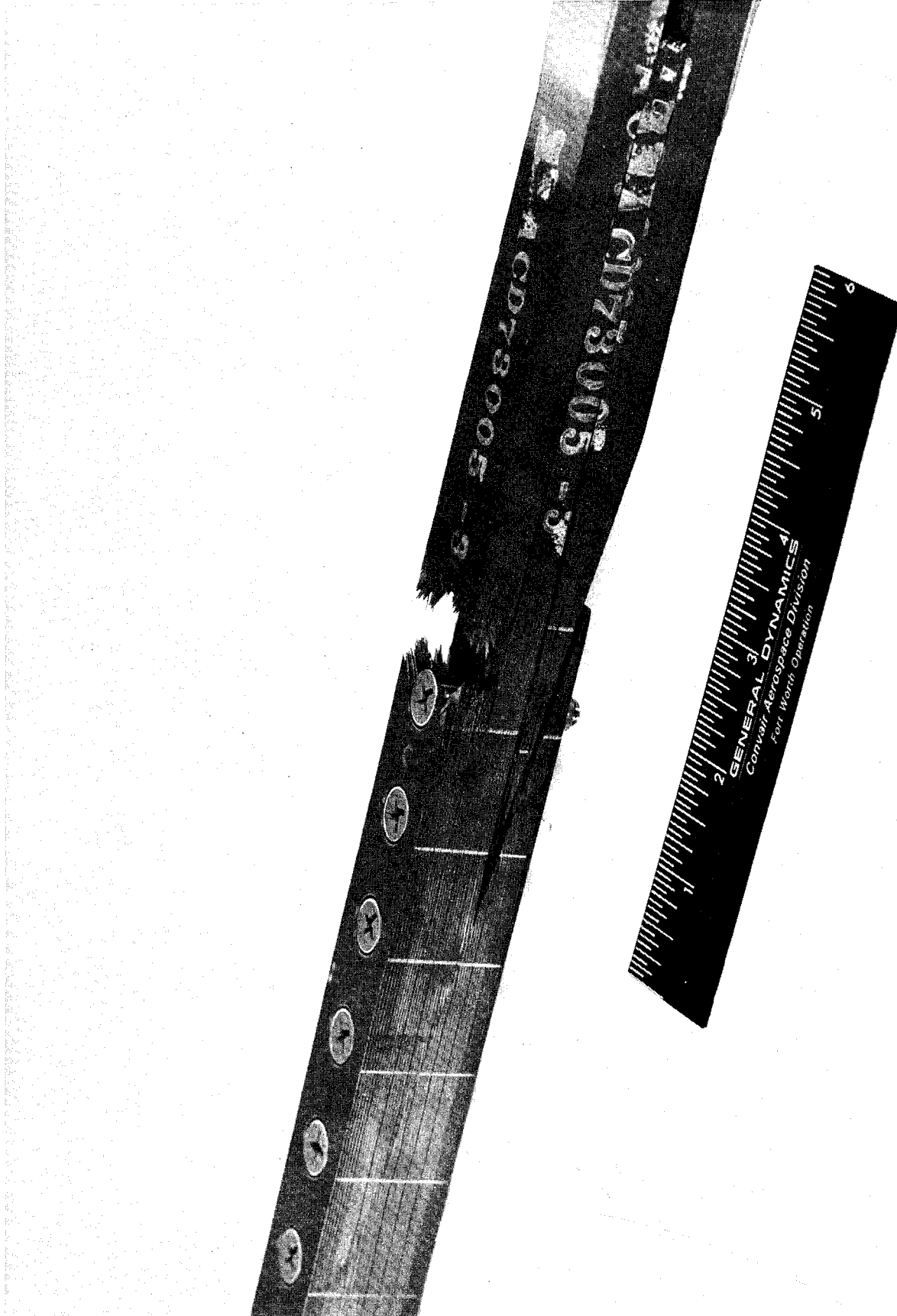
Figure 20 Static Tension Failure
