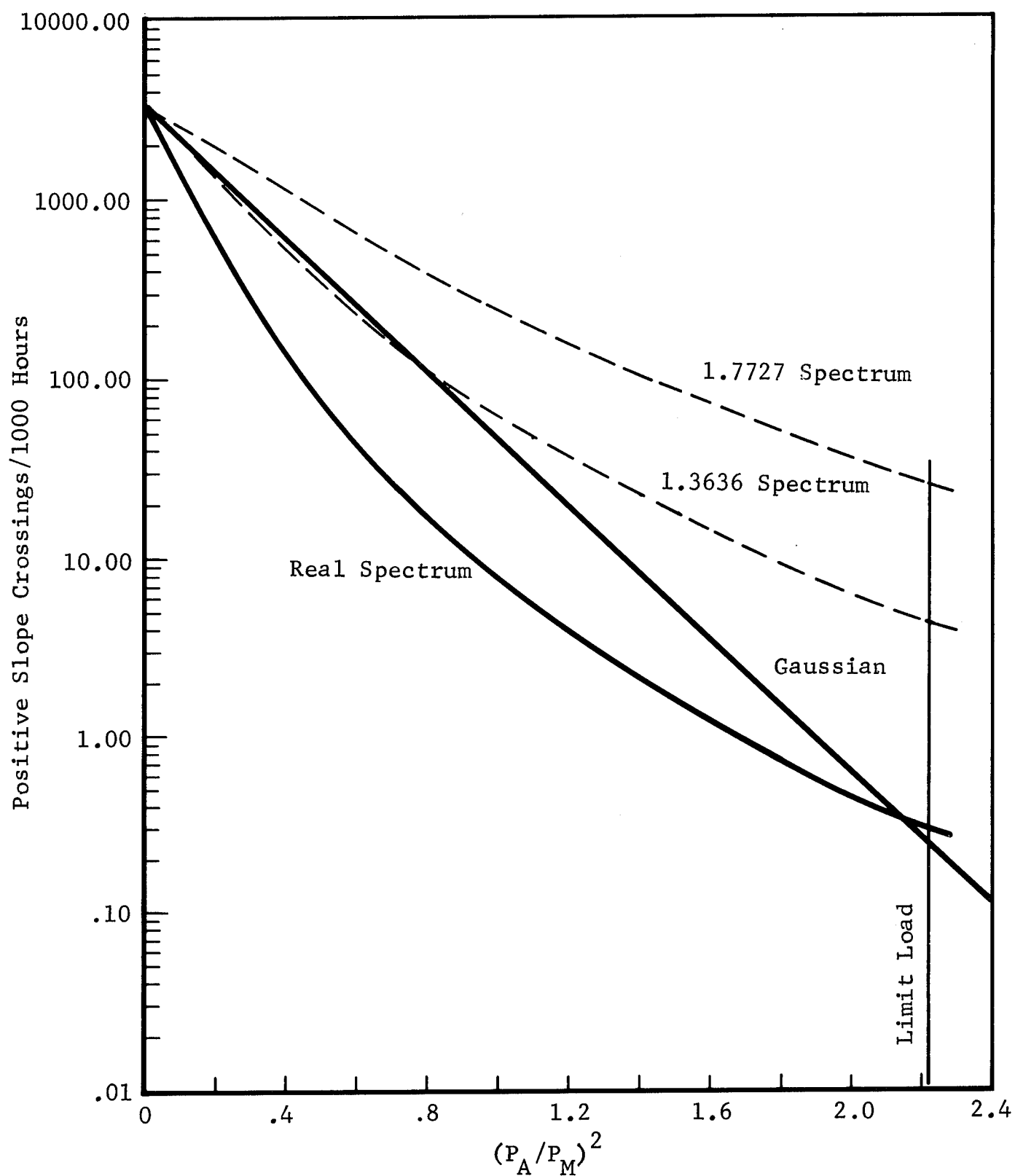
Figure 8 Transport Load Spectrum
