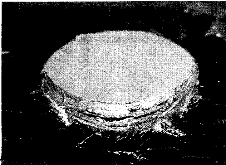
Thin End Countersunk Hole - View From Inside Scarf
