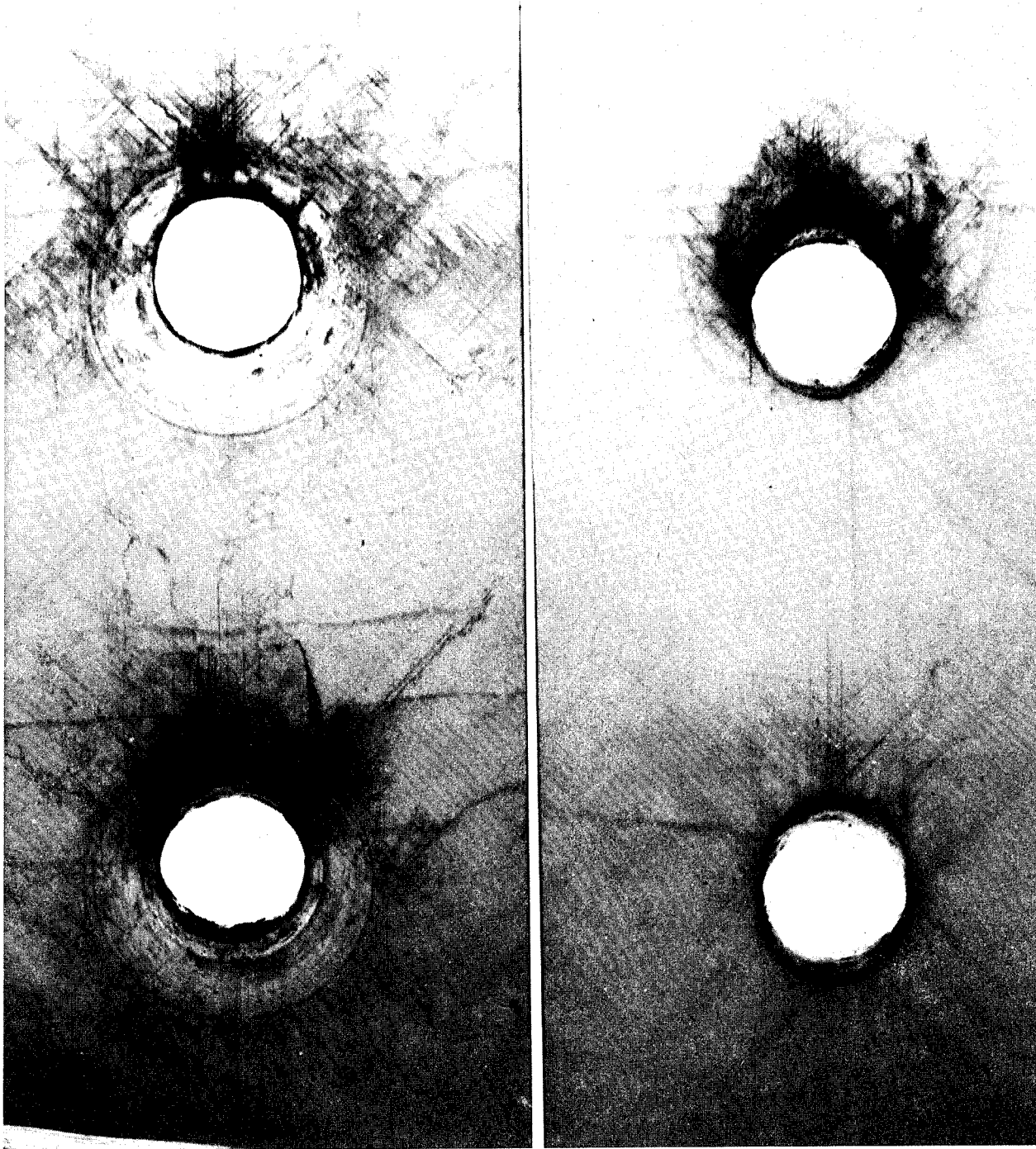
Figure 25 Tension Fatigue Damage at 0.854 Lifetimes
