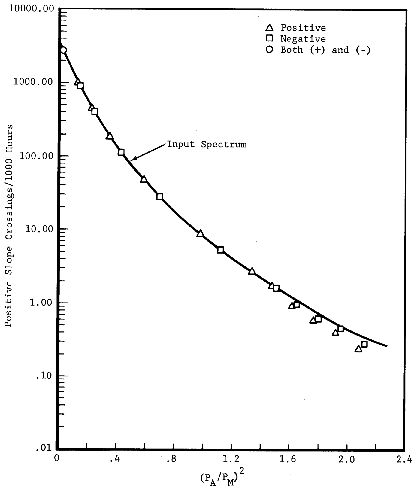
Figure 10 Comparison of Input and Output Spectra
