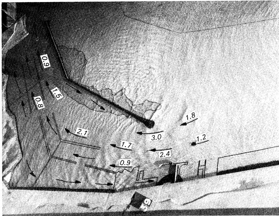
Photo 14. Typical wave patterns, current patterns, and current magnitudes (prototype feet per second) for "modified" existing conditions; 12.5-sec, 8-ft test waves; swl = +5.0 ft (maximum flood)
