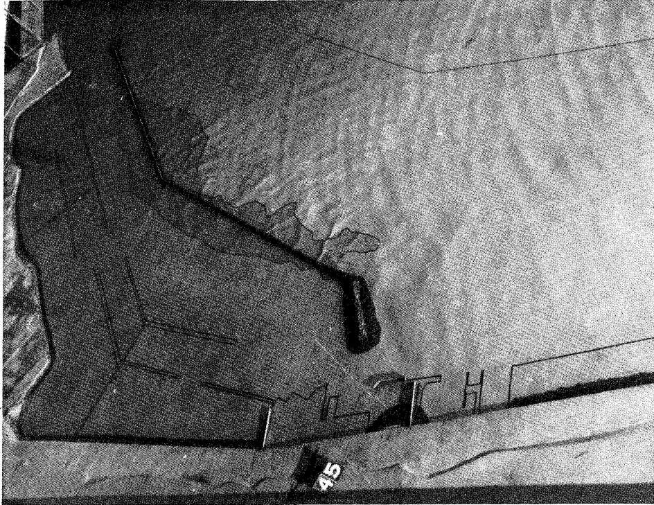
Photo 35. Typical wave patterns for Plan 5B; 12.5-sec, 8-ft test waves; swl = +8.0 ft
