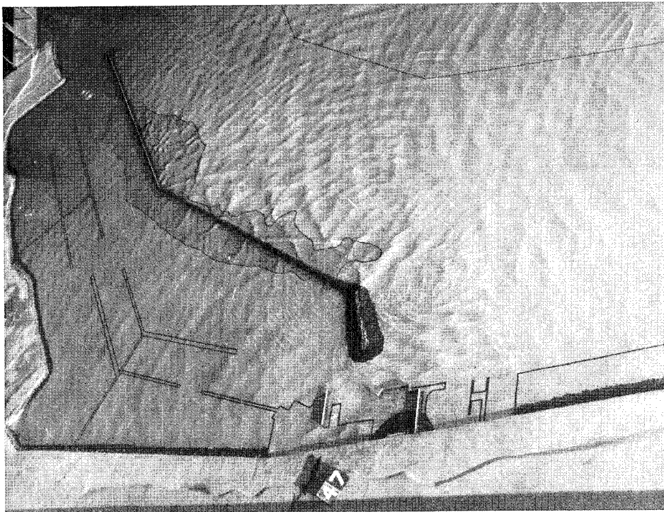
Photo 34. Typical wave patterns for Plan 5A; 12.5-sec, 8-ft test waves; swl = +8.0 ft
