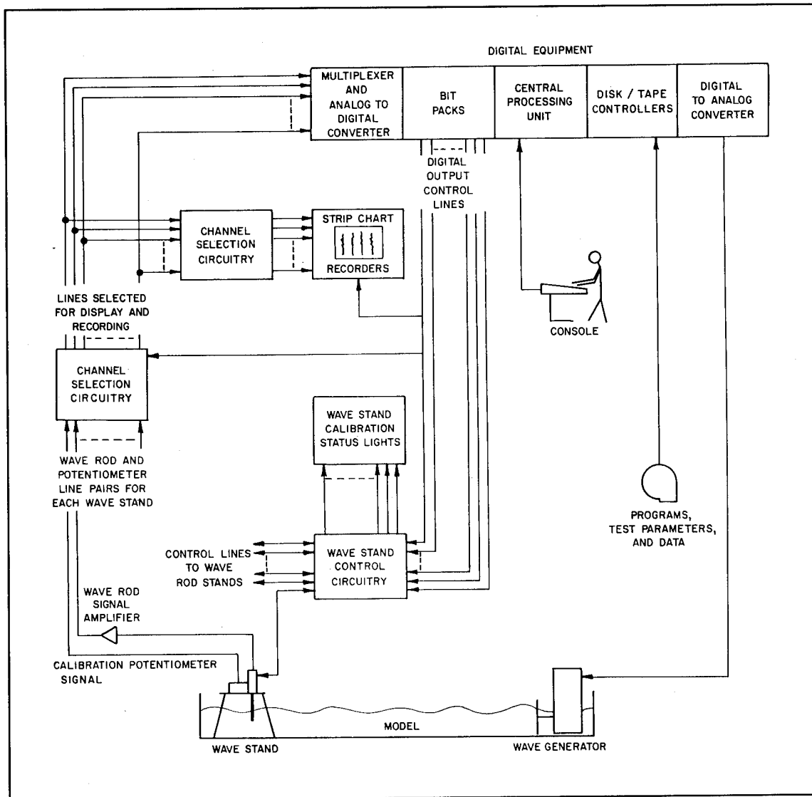
Figure 7. Automated data acquisition and control system
