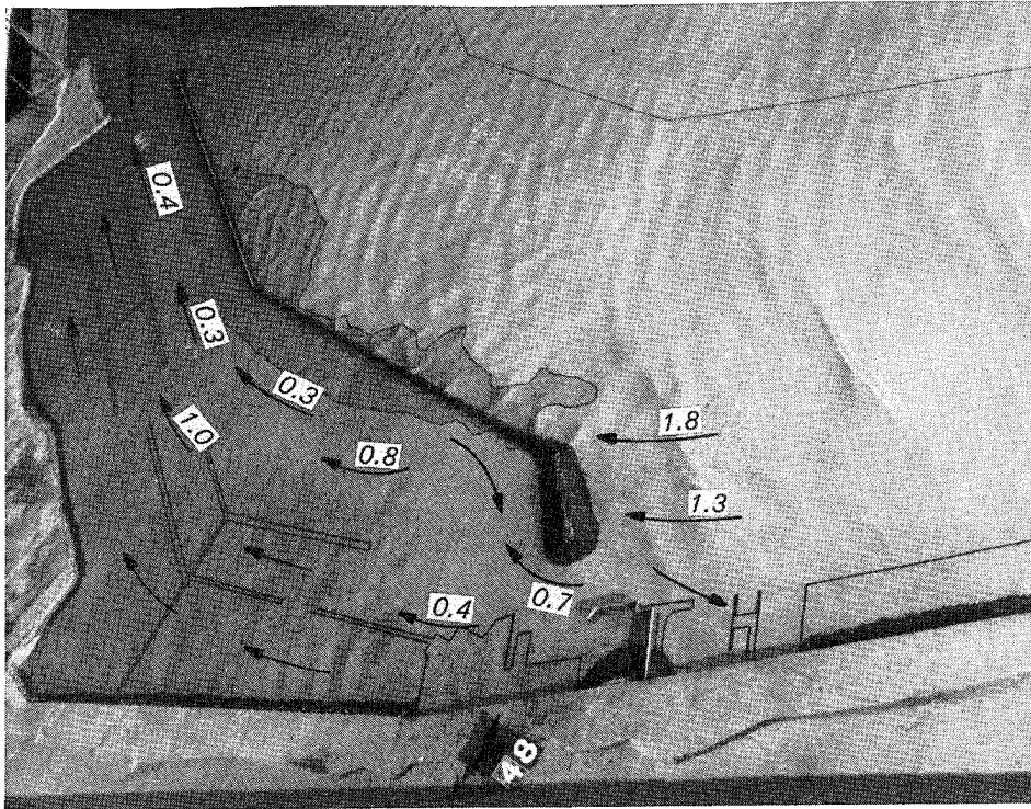
Photo 47. Typical wave patterns, current patterns, and current magnitudes (prototype feet per second) for Plan 5; 12.5-sec, 8-ft test waves; swl = +8.0 ft
