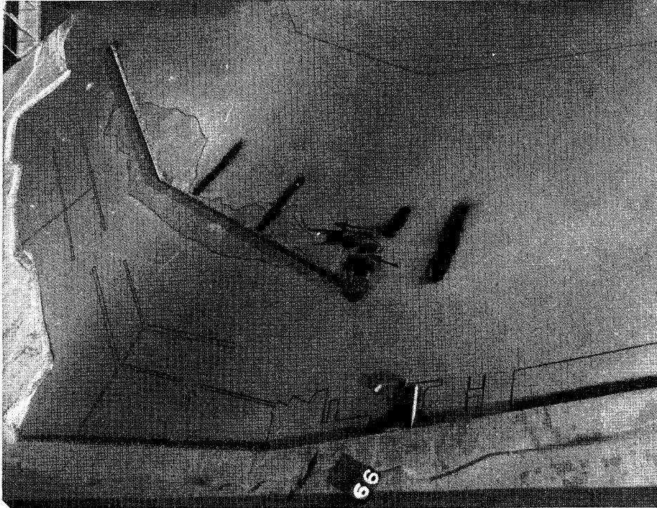
Photo 21. General movement of tracer material and subsequent deposits for "modified" existing conditions for 14.3-sec, 3-ft test waves; swl = 0.0 ft
