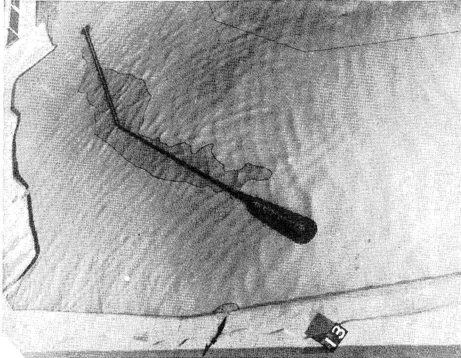
Photo 3. Typical wave patterns for Plan 1A; preliminary tests; 12.5-sec, 8-ft test waves; swl = +8.0 ft
