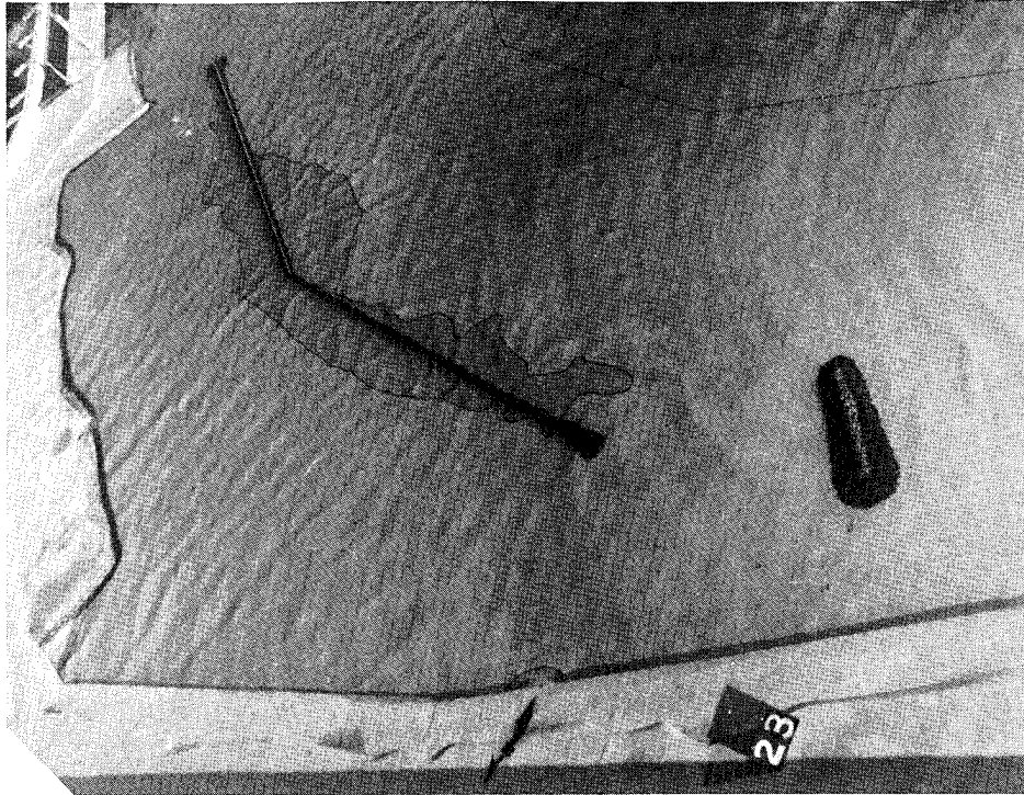
Photo 5. Typical wave patterns for Plan 2; preliminary tests; 12.5-sec, 8-ft test waves; swl = +8.0 ft
