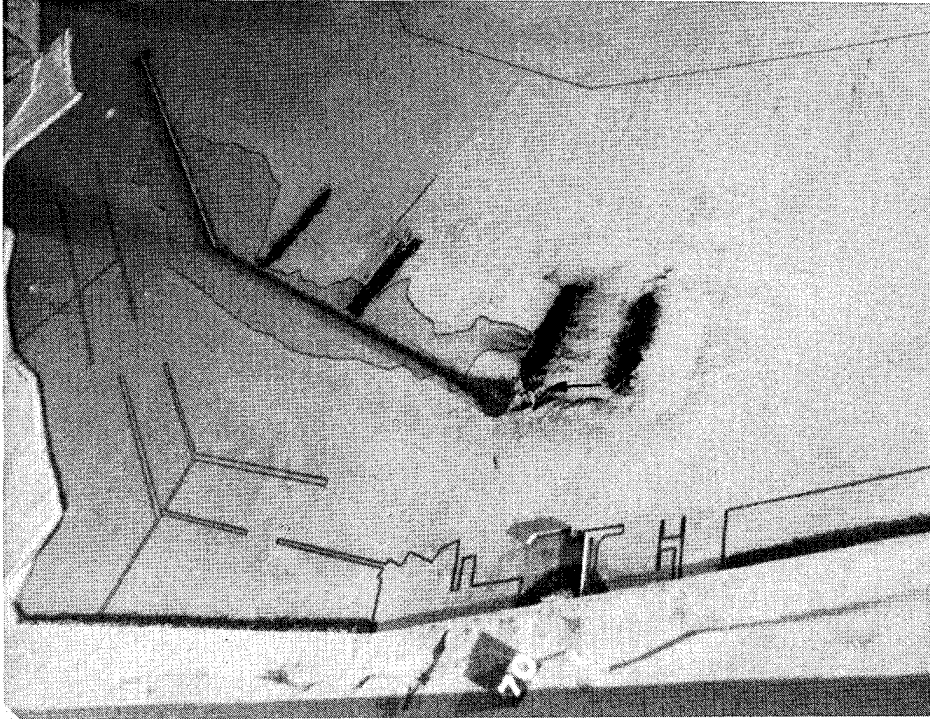
Photo 25. General movement of tracer material and subsequent deposits for "modified" existing conditions for 14.3-sec, 3-ft test waves; swl = +5.0 ft (maximum flood)
