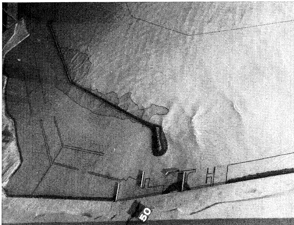
Photo 32. Typical wave patterns for Plan 4C; 12.5-sec, 8-ft test waves; swl = + 8.0 ft
