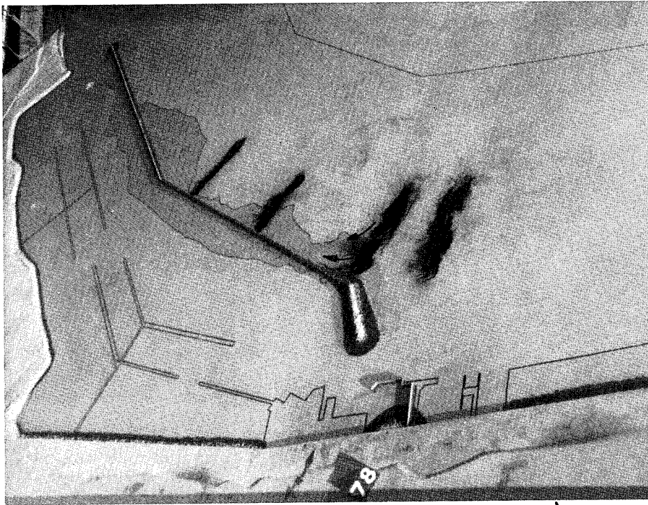
Photo 53. General movement of tracer material and subsequent deposits for Plan 5 for 14.3-sec, 3-ft test waves; swl = +5.0 ft (maximum ebb)
