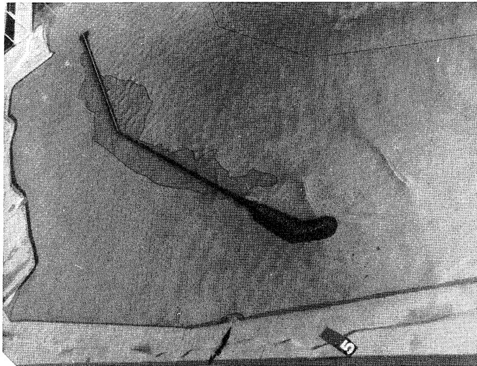
Photo 4. Typical wave patterns for Plan 1B; preliminary tests; 12.5-sec, 8-ft test waves; swl = +8.0 ft
