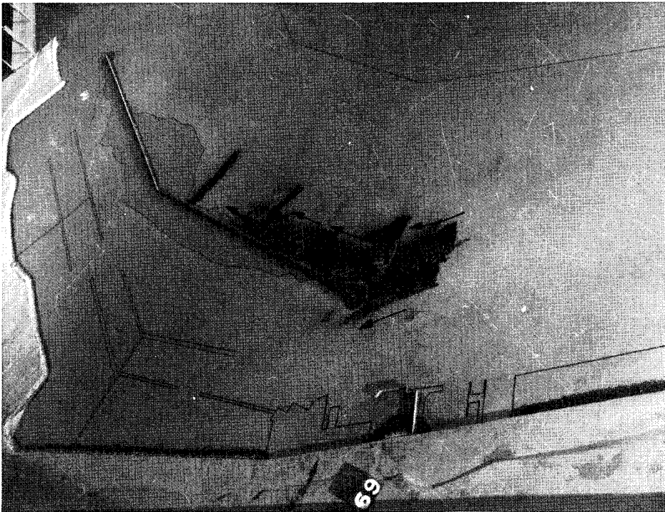
Photo 22. General movement of tracer material and subsequent deposits for "modified" existing conditions for 12.5-sec, 8-ft test waves; swl = +5.0 ft (maximum ebb)
