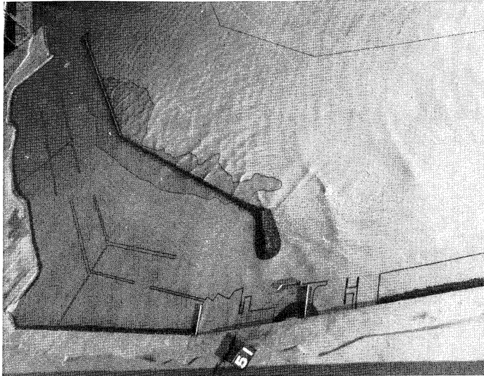
Photo 31. Typical wave patterns for Plan 4B; 12.5-sec, 8-ft test waves; swl = +8.0 ft
