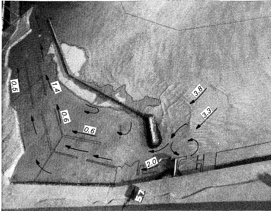
Photo 41. Typical wave patterns, current patterns, and current magnitudes (prototype feet per second) for Plan 5; 12.5-sec, 8-ft test waves; swl = 0.0 ft
