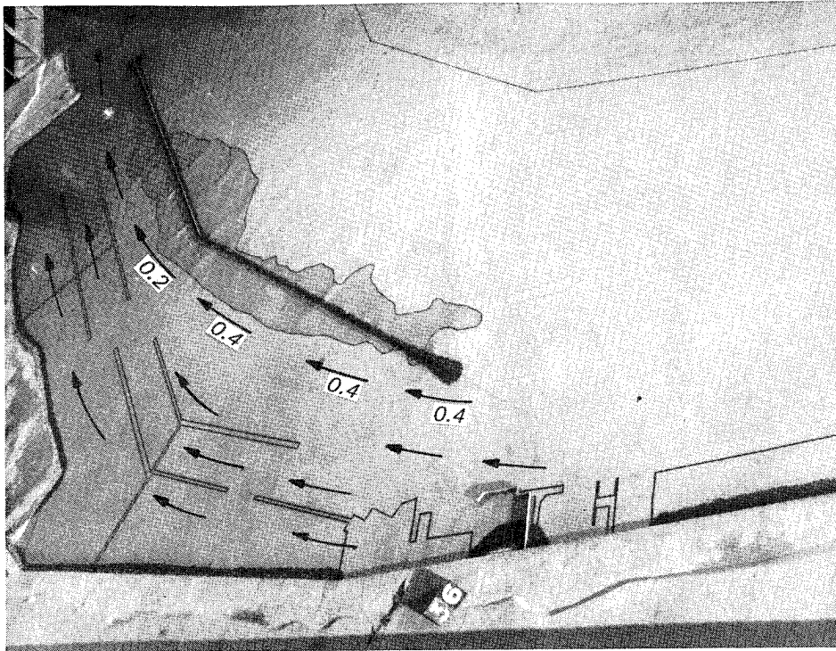
Photo 17. Typical wave patterns, current patterns, and current magnitudes (prototype feet per second) for "modified" existing conditions; 14.3-ft, 3-ft test waves; swl = +8.0 ft
