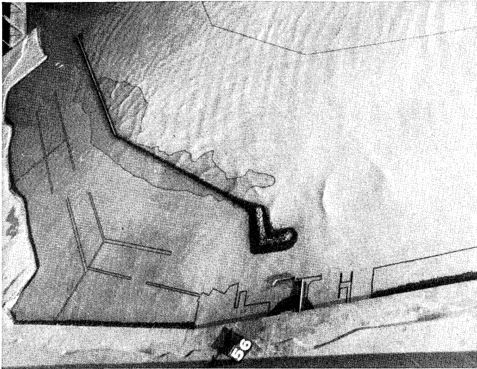
Photo 37. Typical wave patterns for Plan 6; 12.5-sec, 8-ft test waves; swl = +8.0 ft
