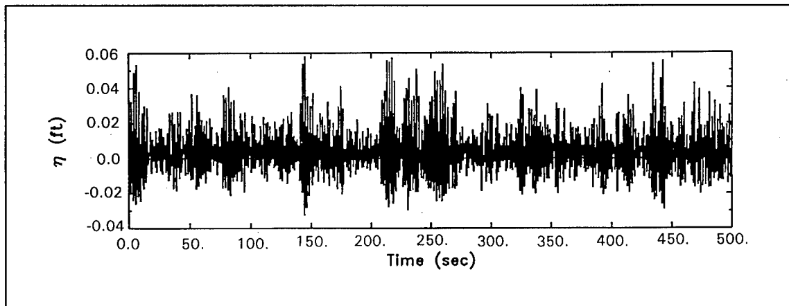
Figure 9. Typical wave train time series, 16.7-sec, 3-ft test waves
