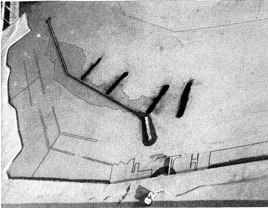
Photo 57. General movement of tracer material and subsequent deposits for Plan 5 for 14.3-sec, 3-ft test waves; swl = +8.0 ft
