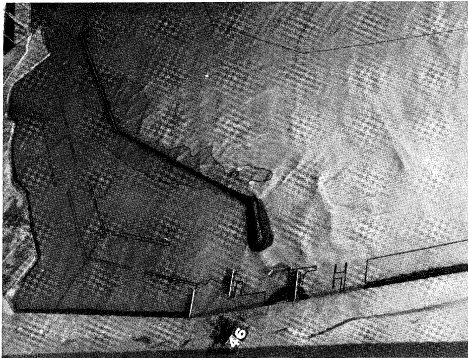
Photo 36. Typical wave patterns for Plan 5C; 12.5-sec, 8-ft test waves; swl = +8.0 ft
