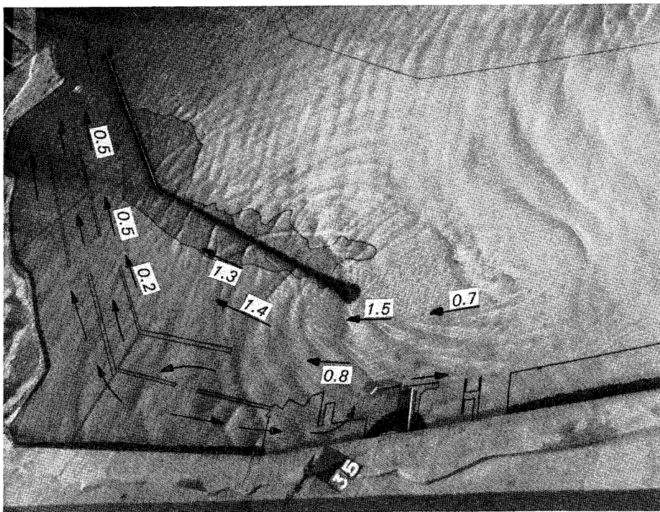
Photo 16. Typical wave patterns, current patterns, and current magnitudes (prototype feet per second) for "modified" existing conditions; 12.5-sec, 8-ft test waves; swl = +8.0 ft
