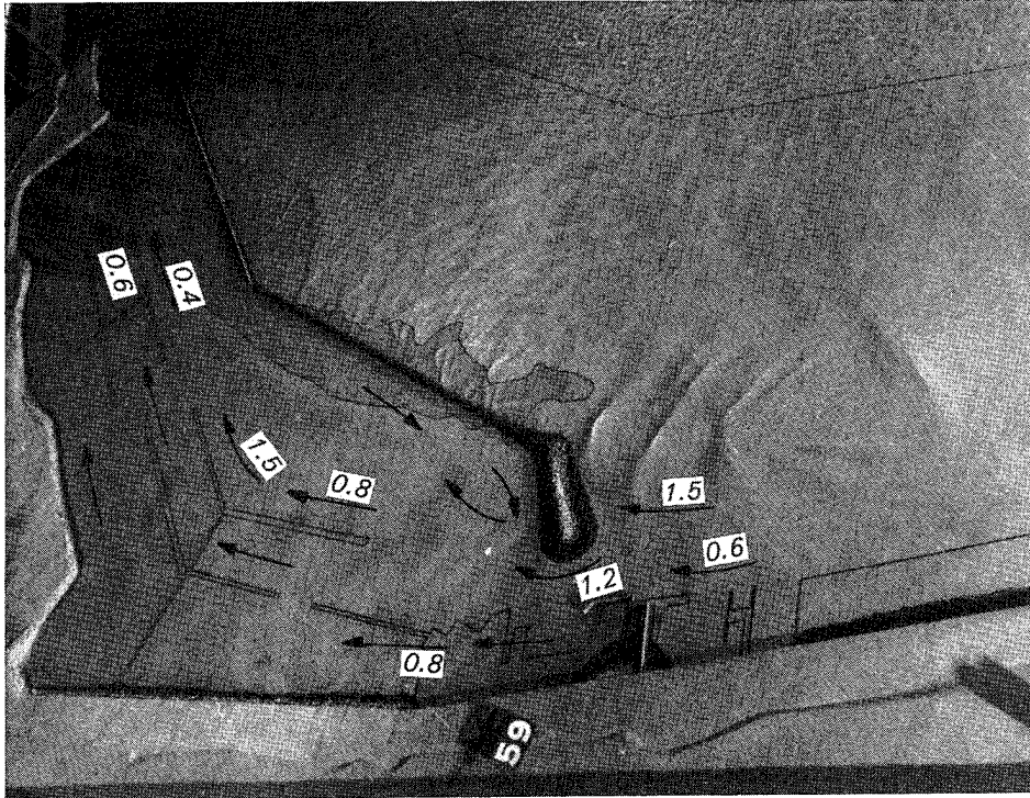
Photo 43. Typical wave patterns, current patterns, and current magnitudes (prototype feet per second) for Plan 5; 12.5-sec, 8-ft test waves; swl = +5.0 ft (maximum ebb)
