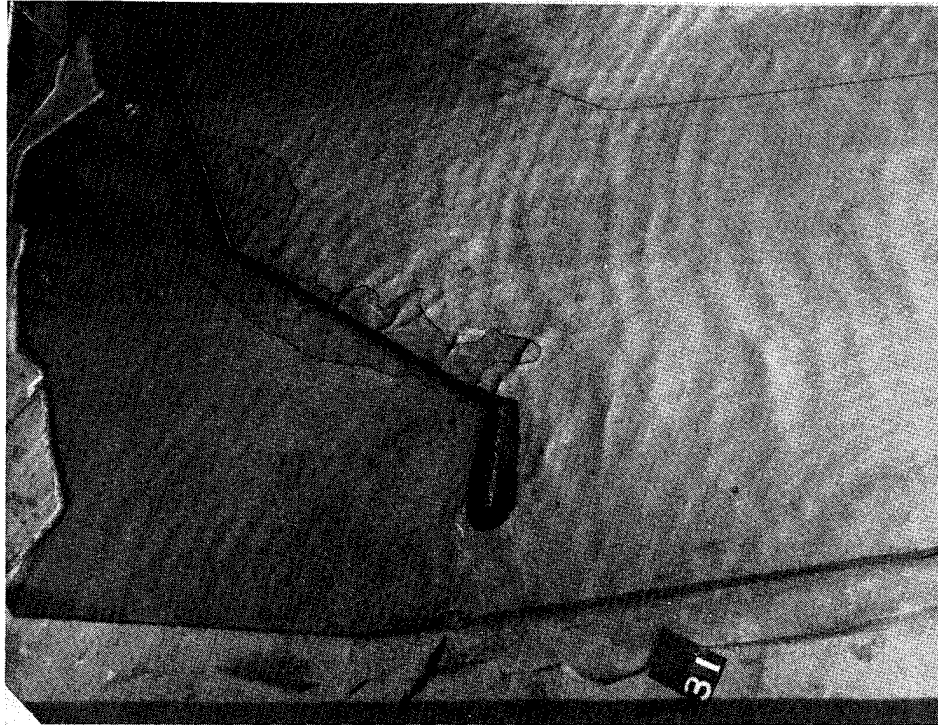
Photo 9. Typical wave patterns for Plan 3A, preliminary tests; 12.5-sec, 8-ft test waves; swl = +8.0 ft
