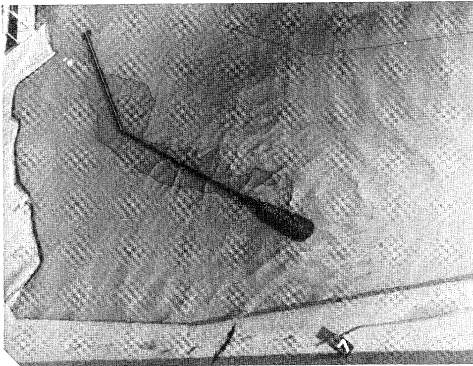
Photo 2. Typical wave patterns for Plan 1; preliminary tests; 12.5-sec, 8-ft test waves; swl = +8.0 ft
