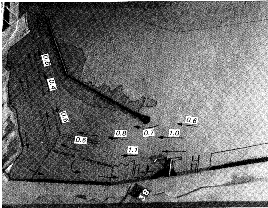
Photo 13. Typical wave patterns, current patterns, and current magnitudes (prototype feet per second) for "modified" existing conditions; 14.3-sec, 3-ft test waves; swl = +5.0 ft (maximum ebb)
