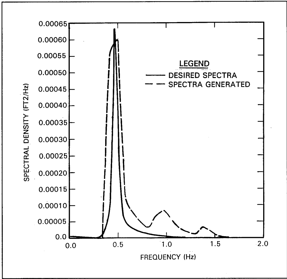
Figure 8. Typical energy density versus frequency plots (model terms) for a wave spectra; 16.7-sec, 3-ft test waves
