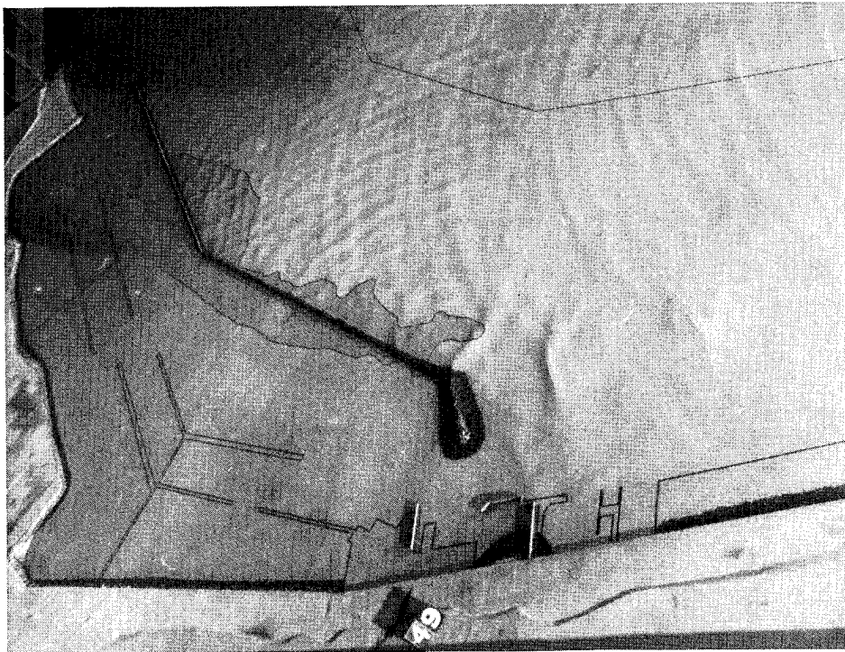
Photo 30. Typical wave patterns for Plan 4A; 12.5-sec, 8-ft test waves; swl = +8.0 ft
