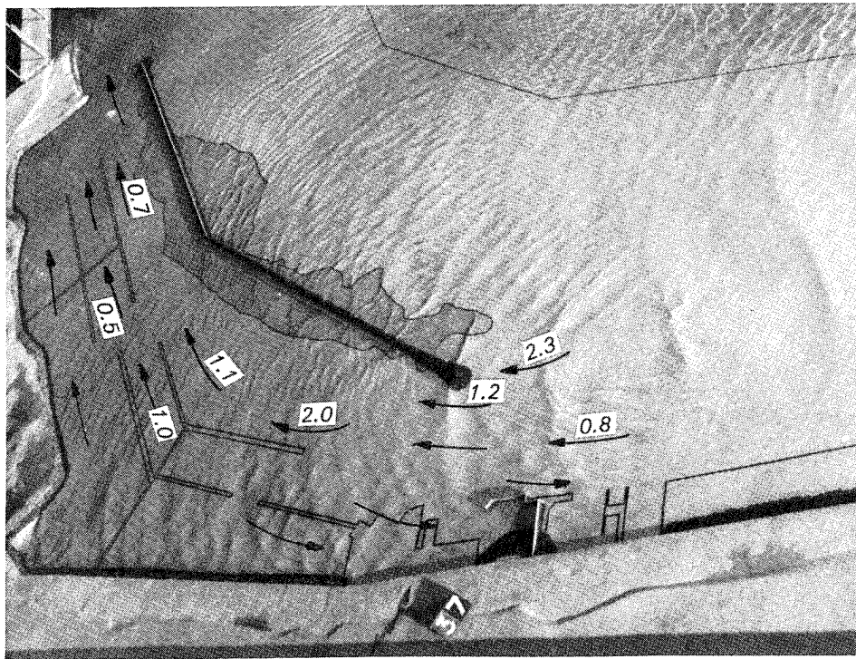
Photo 12. Typical wave patterns, current patterns, and current magnitudes (prototype feet per second) for "modified" existing conditions; 12.5-sec, 8-ft test waves; swl = +5.0 ft (maximum ebb)
