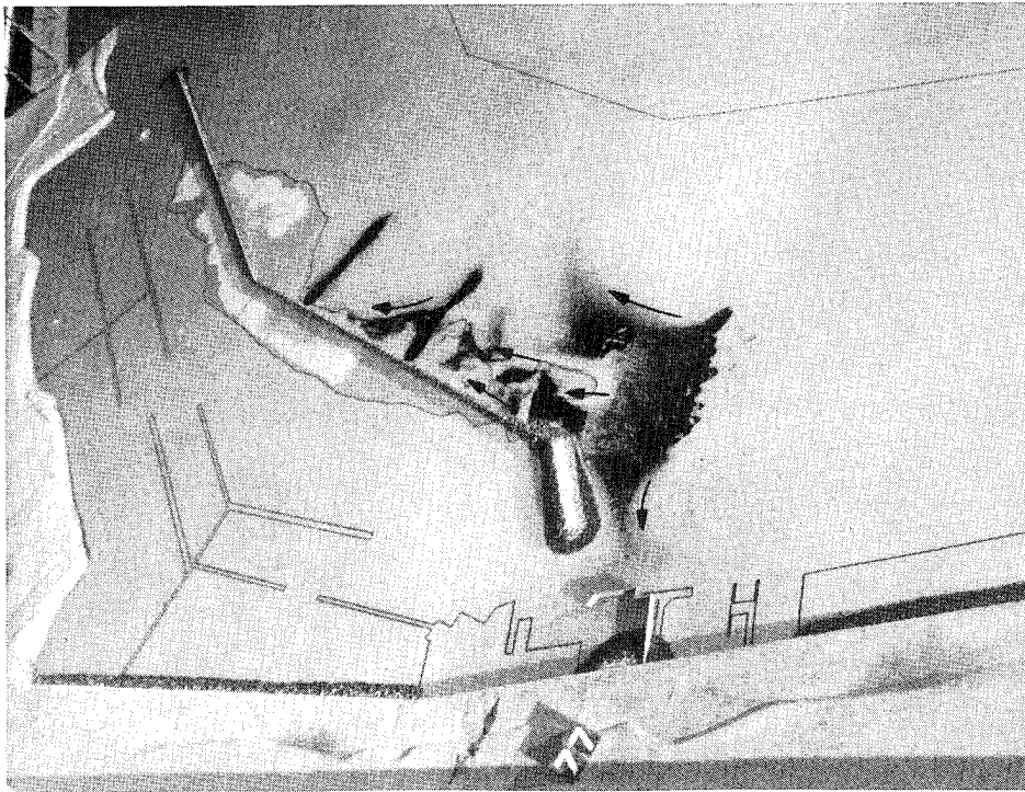
Photo 50. General movement of tracer material and subsequent deposits for Plan 5 for 12.5-sec, 8-ft test waves; swl = 0.0 ft
