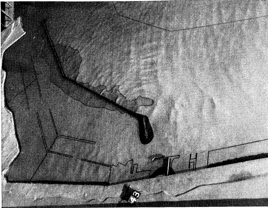
Photo 29. Typical wave patterns for Plan 4; 12.5-sec, 8-ft test waves; swl = +8.0 ft
