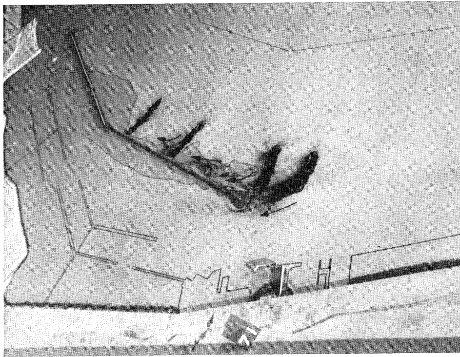
Photo 24. General movement of tracer material and subsequent deposits for "modified" existing conditions for 12.5-sec, 8-ft test waves; swl = +5.0 ft (maximum flood)
