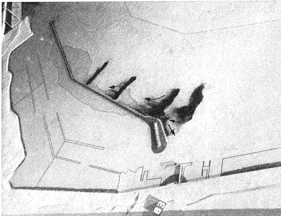
Photo 56. General movement of tracer material and subsequent deposits for Plan 5 for 12.5-sec, 8-ft test waves; swl = +8.0 ft
