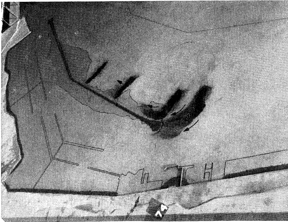
Photo 28. General movement of tracer material and subsequent deposits for "modified" existing conditions for 12.5-sec, 8-ft test waves; swl = +11.0 ft
