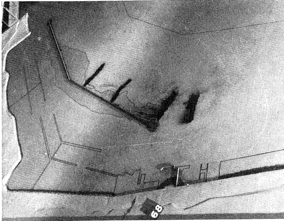
Photo 23. General movement of tracer material and subsequent deposits for "modified" existing conditions for 14.3-sec, 3-ft test waves; swl = +5.0 ft (maximum ebb)
