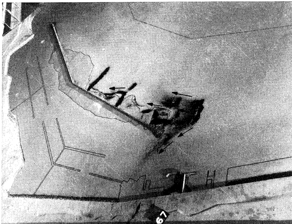
Photo 20. General movement of tracer material and subsequent deposits for "modified" existing conditions for 12.5-sec, 8-ft test waves; swl = 0.0 ft
