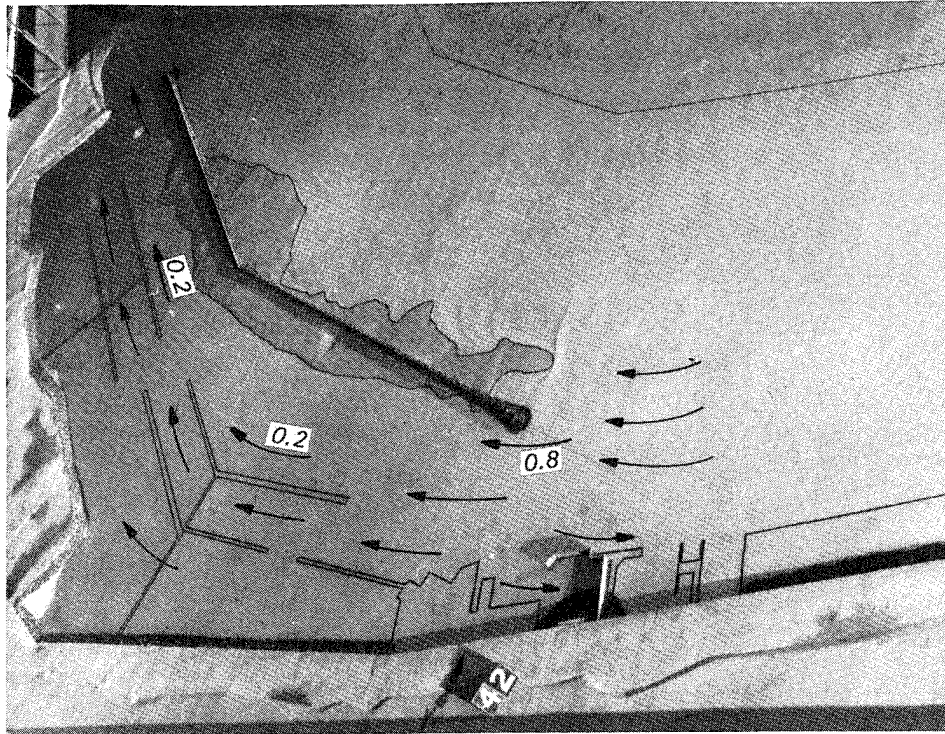
Photo 11. Typical wave patterns, current patterns, and current magnitudes (prototype feet per second) for "modified" existing conditions; 14.3-sec, 3-ft test waves; swl = 0.0 ft
