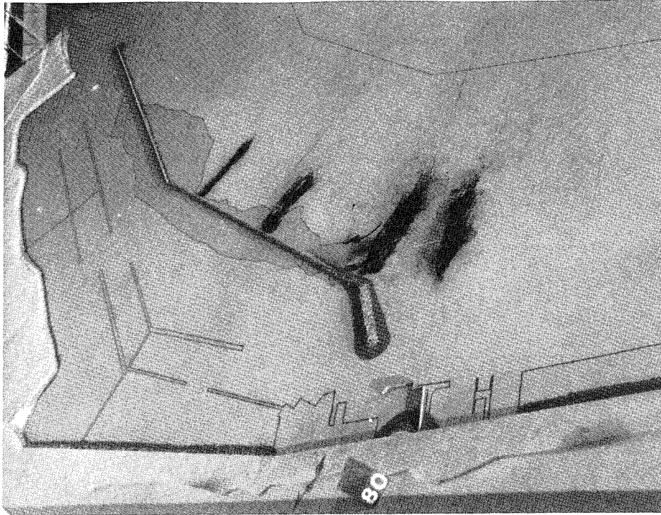
Photo 55. General movement of tracer material and subsequent deposits for Plan 5 for 14.3-sec, 3-ft test waves; swl = +5.0 ft (maximum flood)
