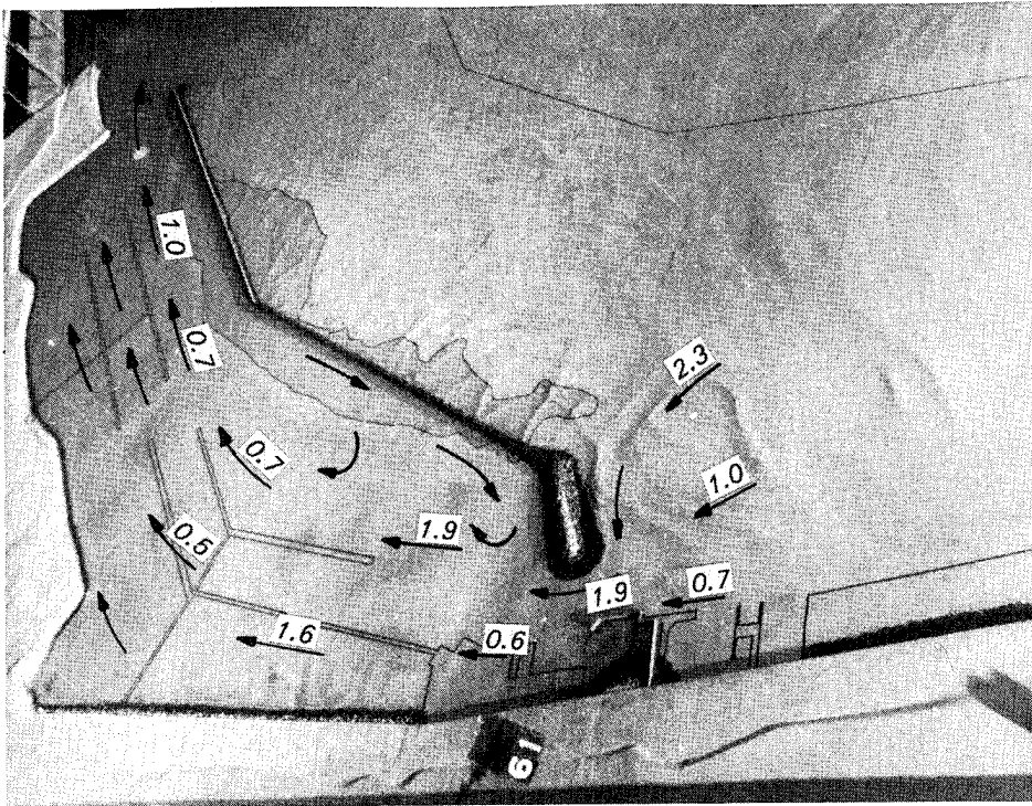
Photo 45. Typical wave patterns, current patterns, and current magnitudes (prototype feet per second) for Plan 5; 12.5-sec, 8-ft test waves; swl = +5.0 ft (maximum flood)
