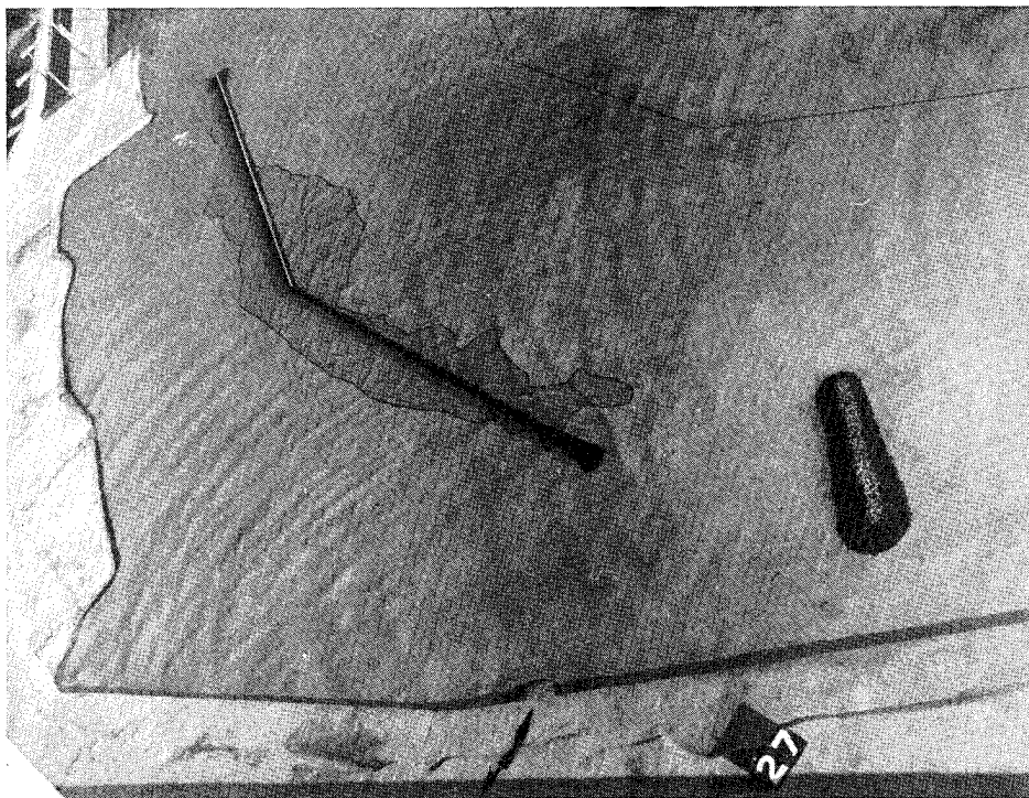
Photo 6. Typical wave patterns for Plan 2A; preliminary tests; 12.5-sec, 8-ft test waves; swl = +8.0 ft
