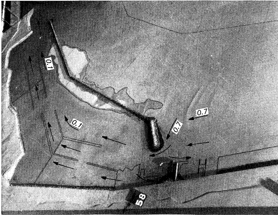
Photo 42. Typical wave patterns, current patterns, and current magnitudes (prototype feet per second) for Plan 5; 14.3-sec, 3-ft test waves; swl = 0.0 ft
