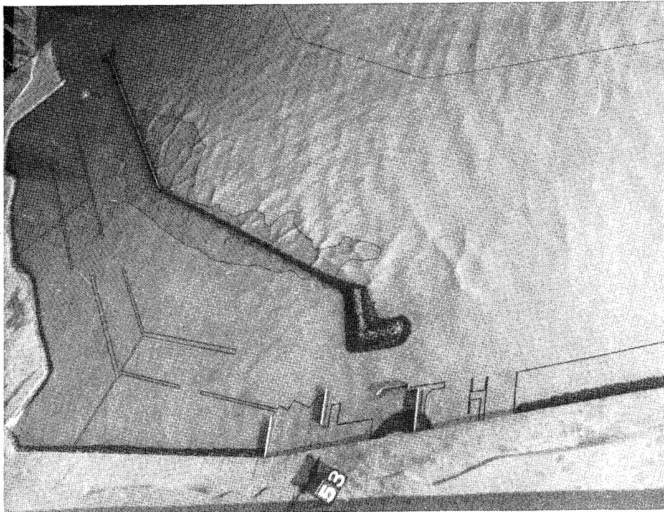
Photo 40. Typical wave patterns for Plan 6C; 12.5-sec, 8-ft test waves; swl = +8.0 ft
