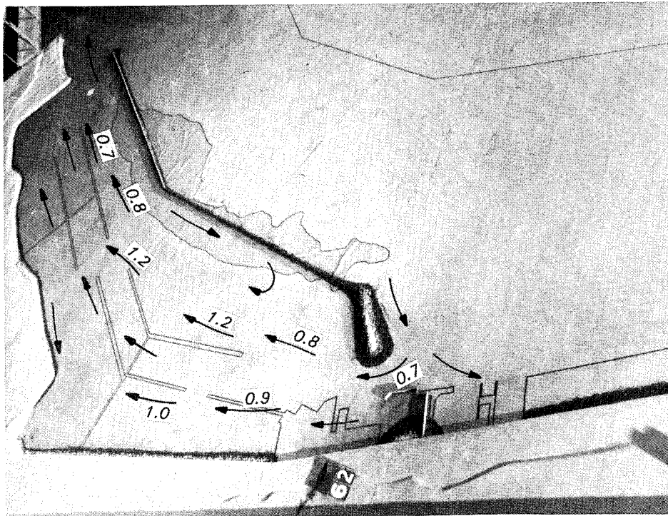
Photo 46. Typical wave patterns, current patterns, and current magnitudes (prototype feet per second) for Plan 5; 14.3-sec, 3-ft test waves; swl = +5.0 ft (maximum flood)
