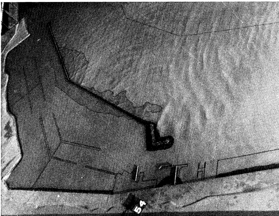
Photo 38. Typical wave patterns for Plan 6A; 12.5-sec, 8-ft test waves; swl = +8.0 ft
