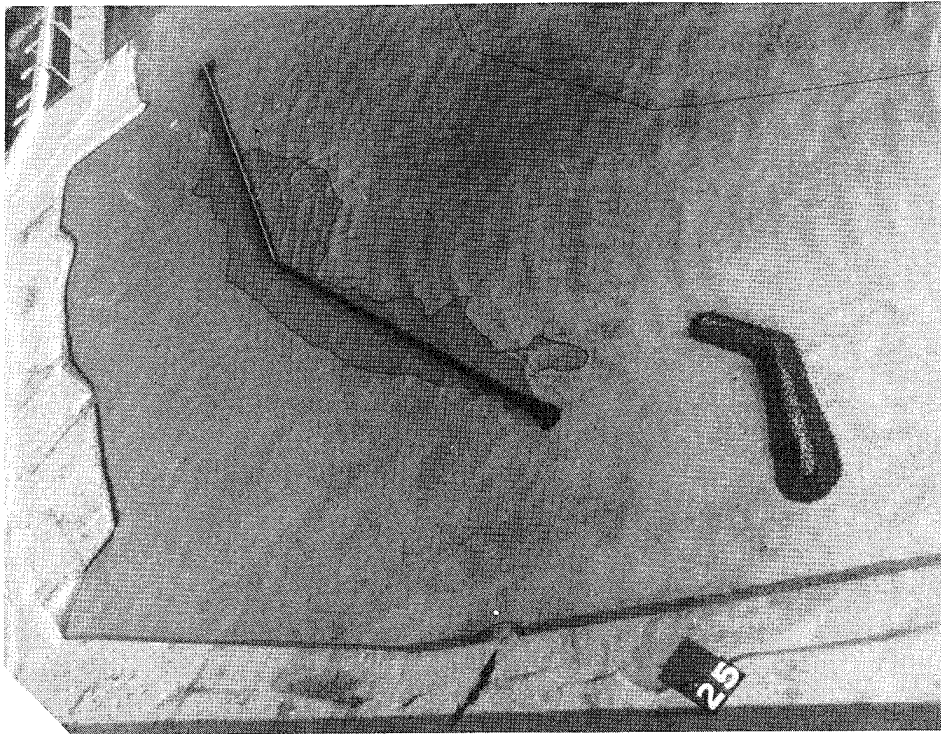
Photo 7. Typical wave patterns for Plan 2B; preliminary tests; 12.5-sec, 8-ft test waves; swl = +8.0 ft
