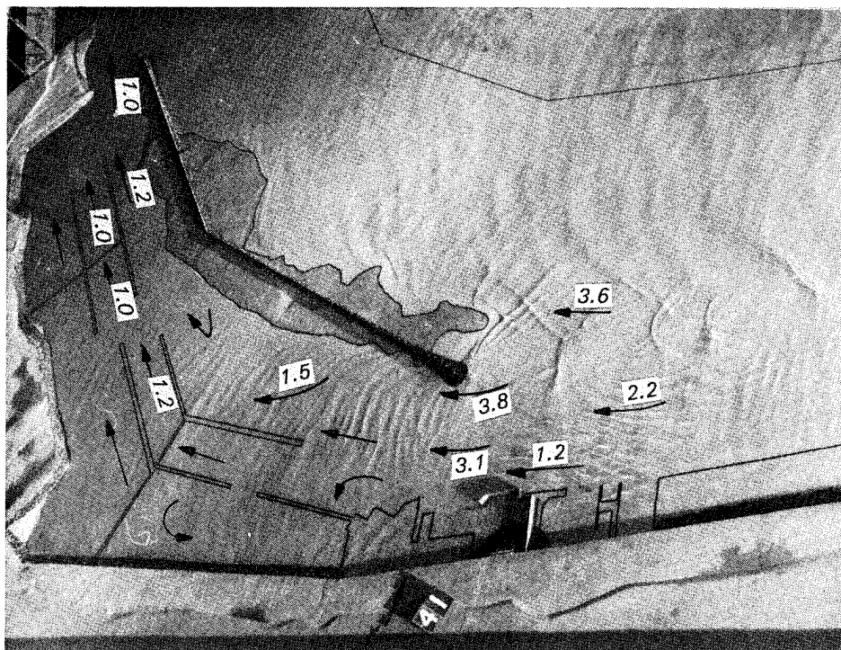
Photo 10. Typical wave patterns, current patterns, and current magnitudes (prototype feet per second) for "modified" existing conditions; 12.5-sec, 8-ft test waves; swl = 0.0 ft
