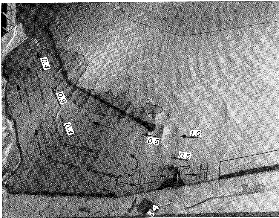
Photo 18. Typical wave patterns, current patterns, and current magnitudes (prototype feet per second) for "modified" existing conditions; 12.5-sec, 8-ft test waves; swl = +11.0 ft
