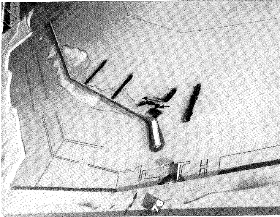
Photo 51. General movement of tracer material and subsequent deposits for Plan 5 for 14.3-sec, 3-ft test waves; swl = 0.0 ft
