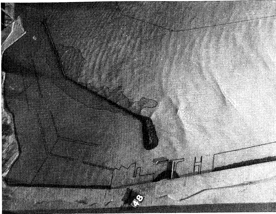
Photo 33. Typical wave patterns for Plan 5; 12.5-sec, 8-ft test waves; swl = +8.0 ft
