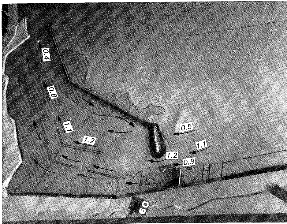
Photo 44. Typical wave patterns, current patterns, and current magnitudes (prototype feet per second) for Plan 5; 14.3-sec, 3-ft test waves; swl = +5.0 ft (maximum ebb)
