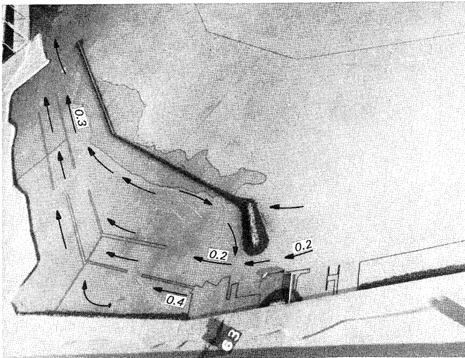
Photo 48. Typical wave patterns, current patterns, and current magnitudes (prototype feet per second) for Plan 5; 14.3-sec, 3-ft test waves; swl = +8.0 ft
