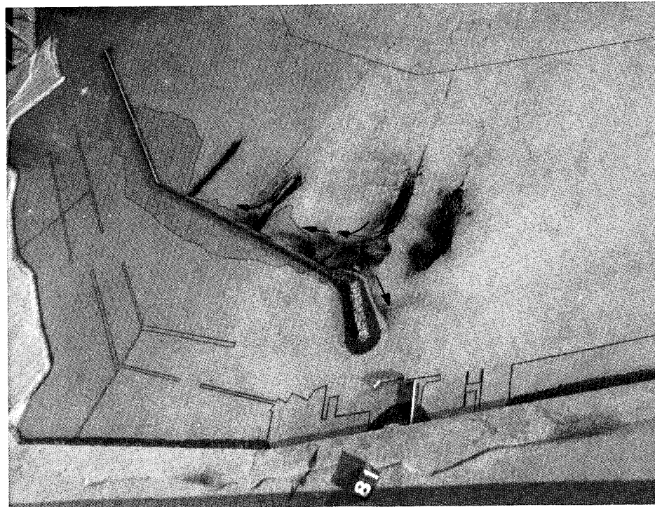
Photo 54. General movement of tracer material and subsequent deposits for Plan 5 for 12.5-sec, 8-ft test waves; swl = +5.0 ft (maximum flood)
