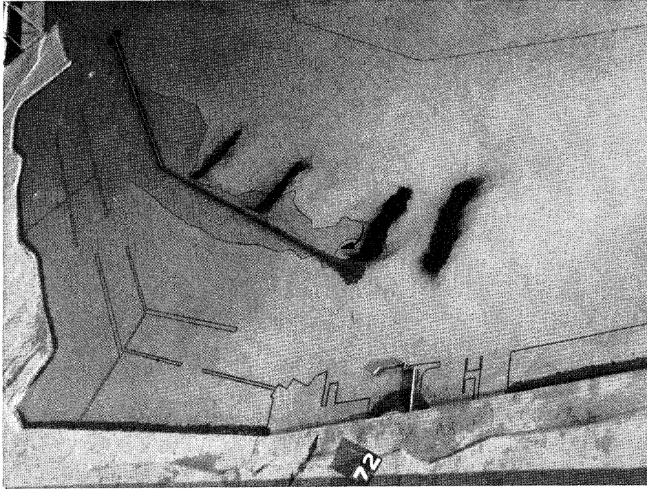
Photo 27. General movement of tracer material and subsequent deposits for "modified" existing conditions for 14.3-sec, 3-ft test waves; swl = +8.0 ft
