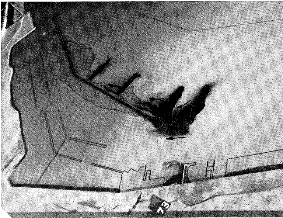
Photo 26. General movement of tracer material and subsequent deposits for "modified" existing conditions for 12.5-sec, 8-ft test waves; swl = +8.0 ft
