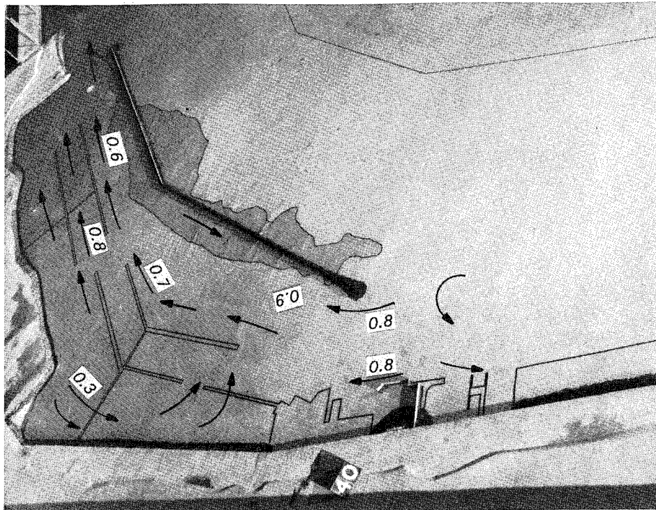
Photo 15. Typical wave patterns, current patterns, and current magnitudes (prototype feet per second) for "modified" existing conditions; 14.3-sec, 3-ft test waves; swl = +5.0 ft (maximum flood)
