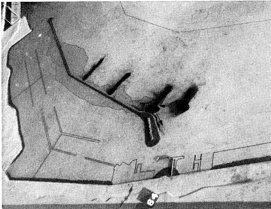
Photo 58. General movement of tracer material and subsequent deposits for Plan 5 for 12.5-sec, 8-ft test waves; swl = +11.0 ft
