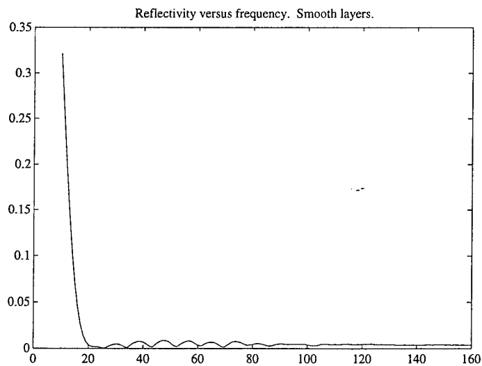
Figure 4: The frequency response of the variable-properties slab shown in figure 5.
