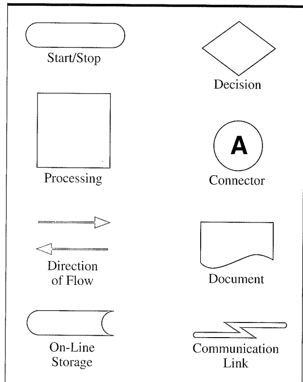
Figure 18. Flowchart Symbols 39 .
