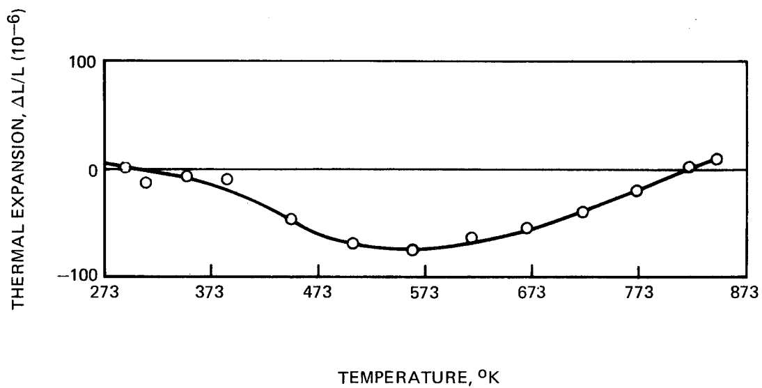
Figure 32. Thermal Expansion of 0° Celanese DG – 102 Fiber Reinforced 7740 , Slurry B
