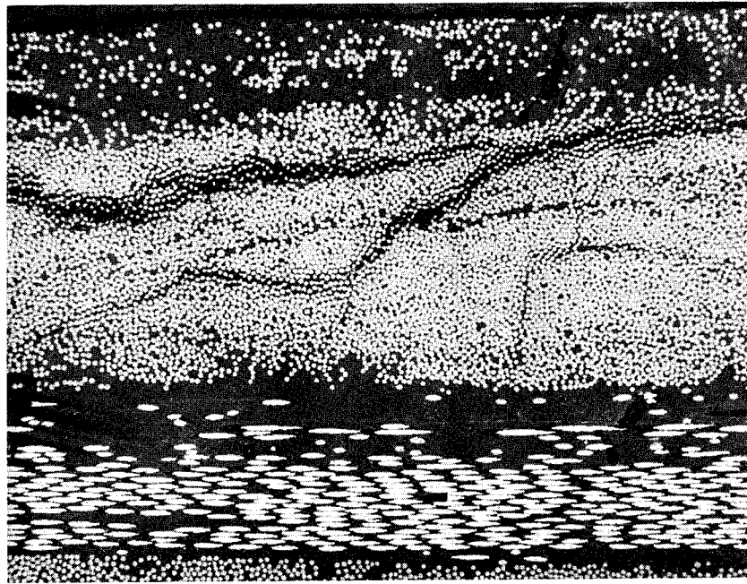
Figure 28. Microstructure of Specimen GC 30 203 Celanese DG 102 Reinforced 7740, [ ( 90 2 O 2 ) 2 ] s , Slurry B
