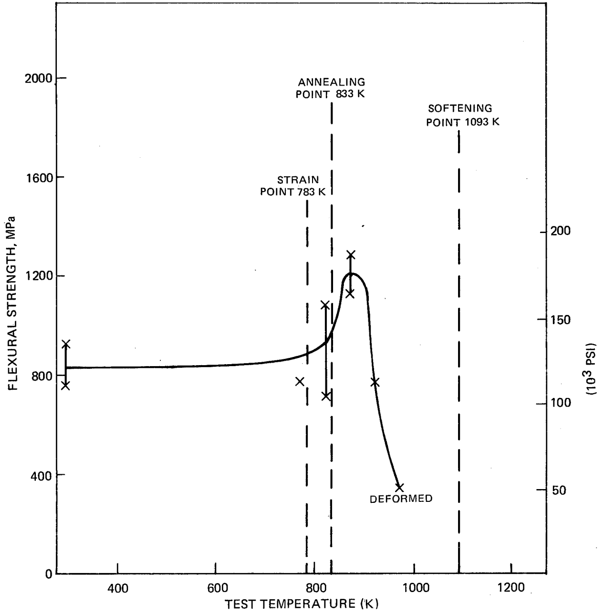
Figure 10. Flexural Strength of Hercules HMS - 10 K Fiber Reinforced 7740 Glass as a Function of Test Temperature, Slurry A
