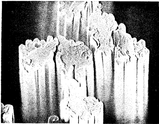
THORNEL 75 GRADE WYL 160 2 μm
