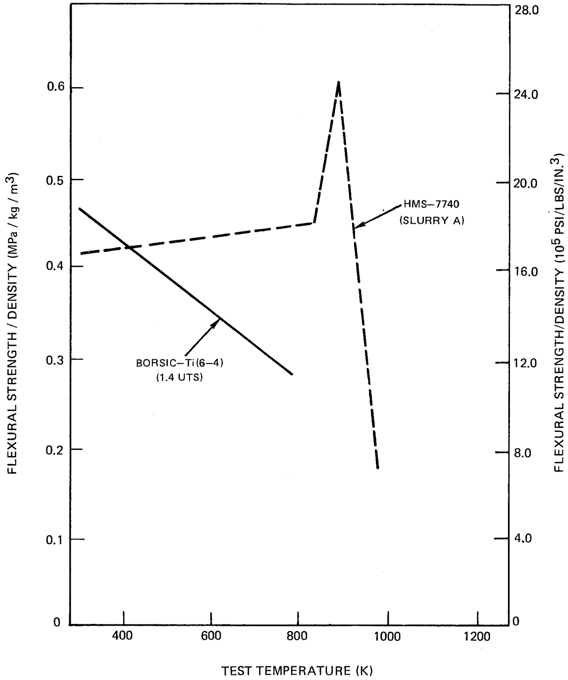
Figure 16. Specific Flexural Strength Comparison
