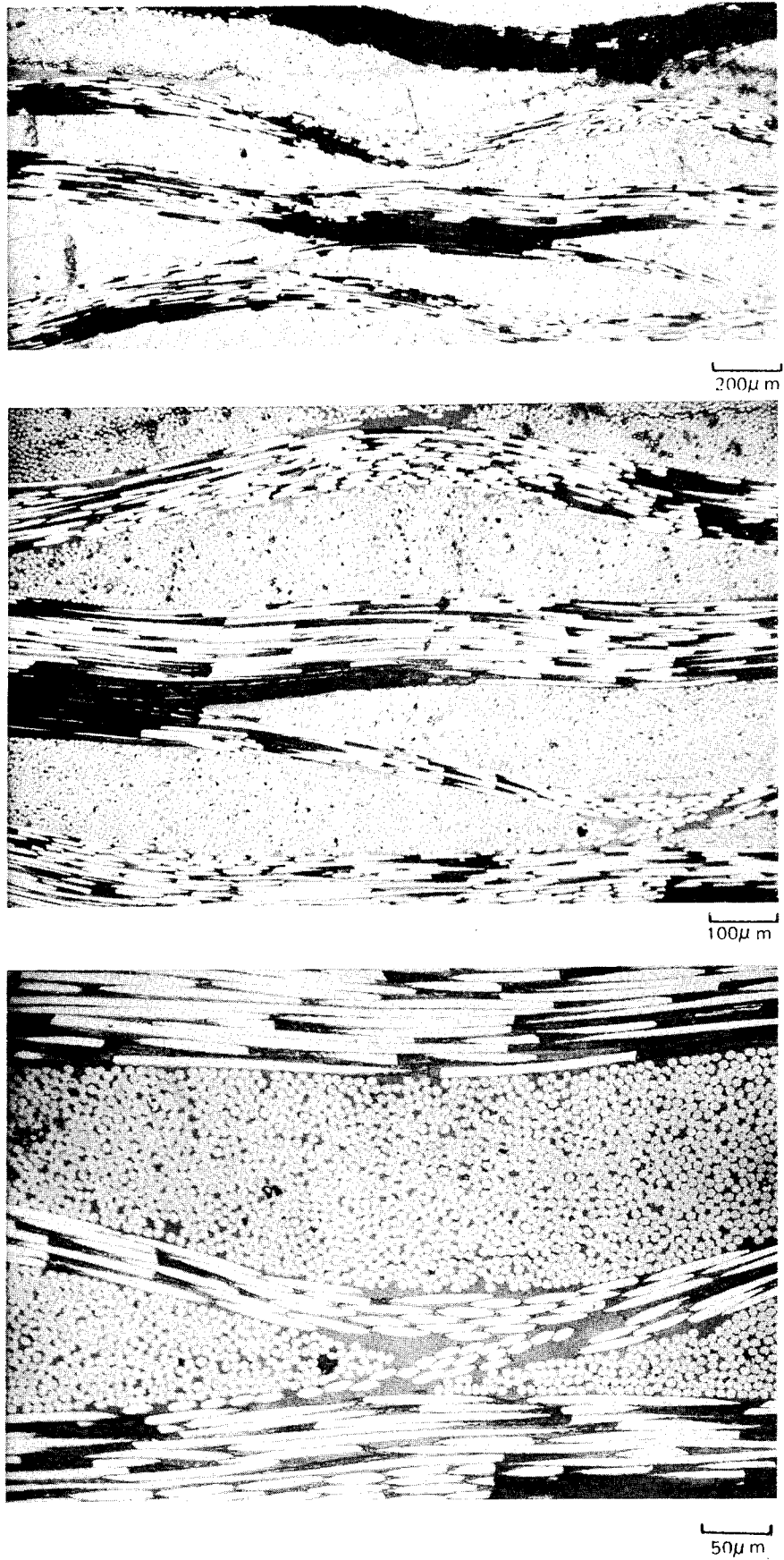
Figure 30. Microstructure of Specimen GC 218-5 Thornel 300 Cloth Reinforced 7740, Slurry B
