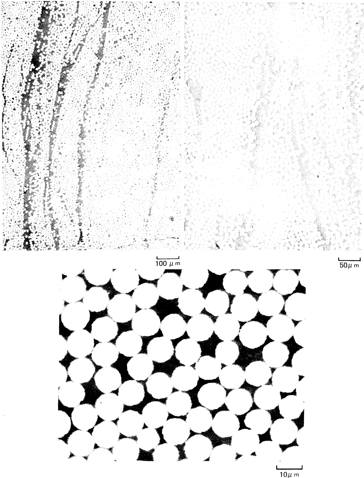
Figure 20. Microstructure of HMS Graphite Fiber Reinforced 7740 Glass Matrix (G.C. 281) Hot Pressed at 1473 K, Slurry B
